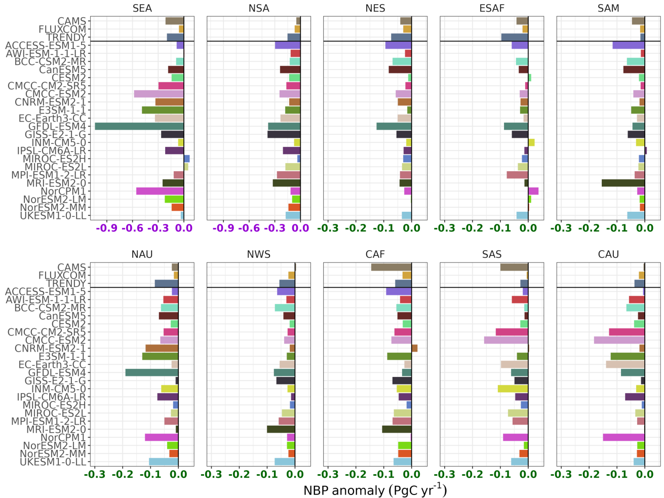
Figure 3. The regional ENSO-induced NBP anomalies in ESM and observational products from an El Niño event of a 90 th percentile intensity. Note the differences in x-axis range.
