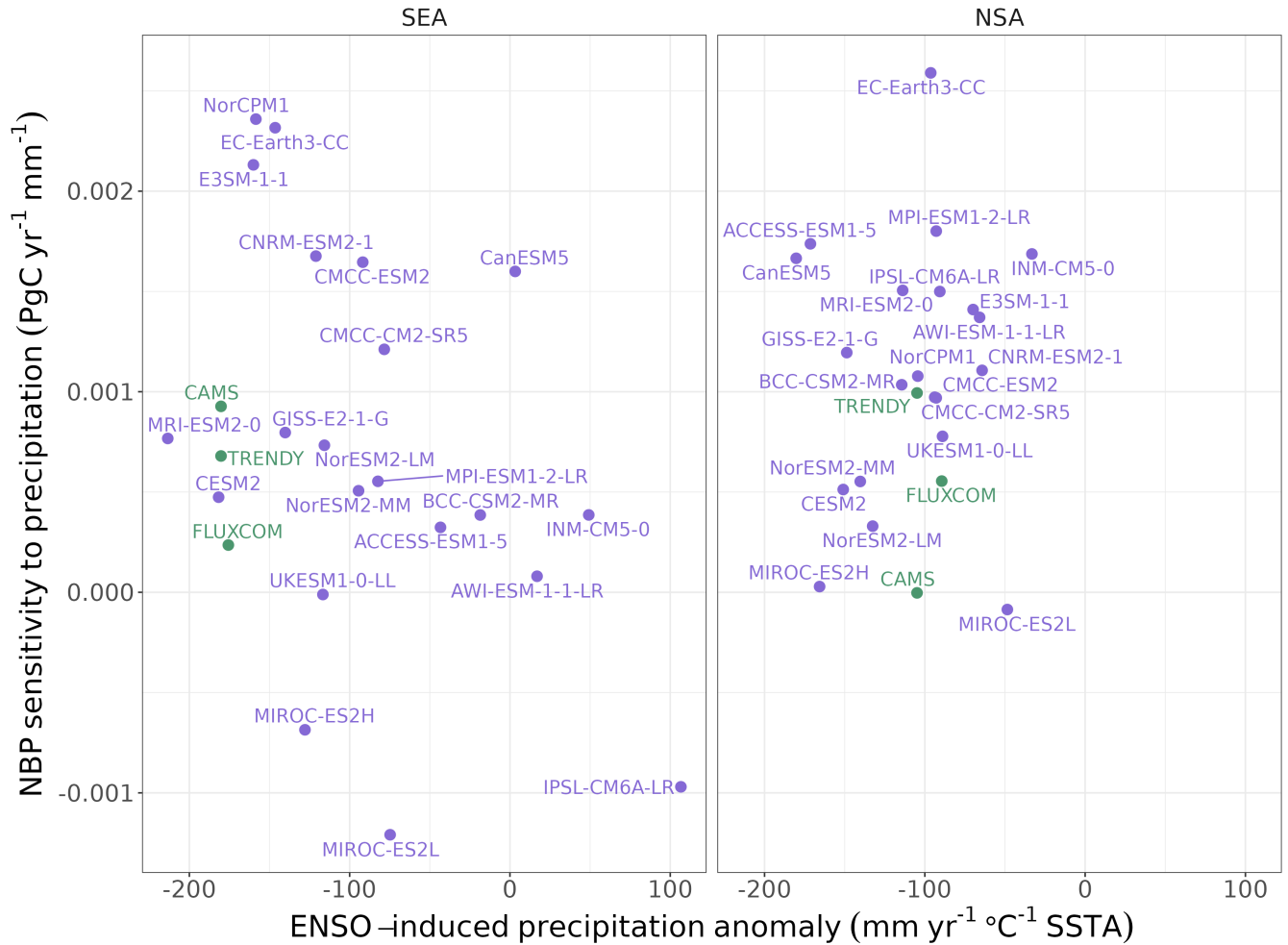
Figure 7. The composition of ENSO-induced NBP anomalies in S.E. Asia (SEA) and N.South-America (NSA). The x-axis shows the ENSO-induced precipitation anomalies, and the y-axis the sensitivity of NBP to precipitation.
