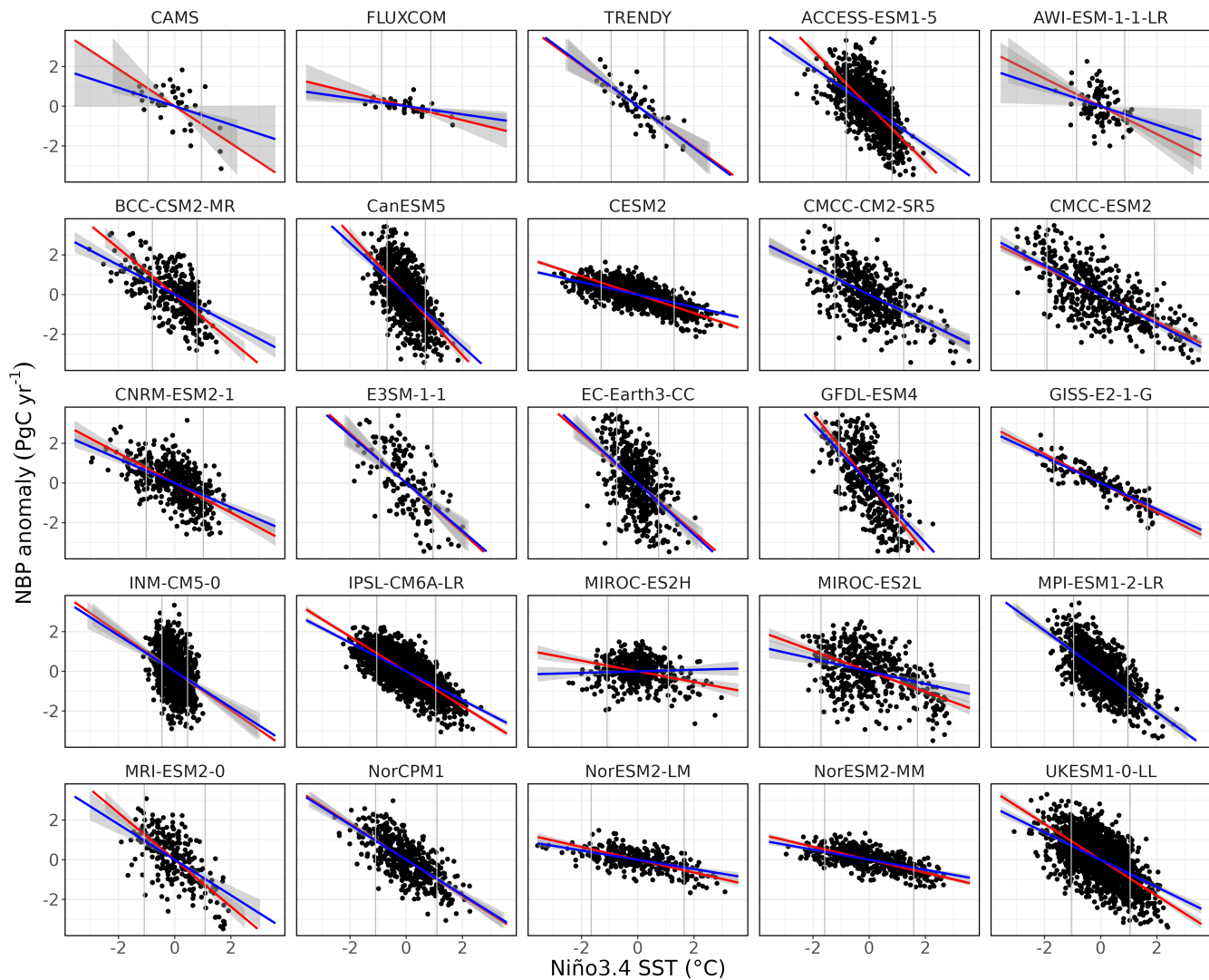
Figure A1. Global annual NBP anomalies against Niño3.4 SSTA in observational and ESM data. The red regression lines are fitted to SSTA values > 0 and the blue lines to values < 0, the grey area represents the 95% confidence interval of the regression lines. The grey vertical lines are the 10th and 90th percentile of ENSO SSTAs.
