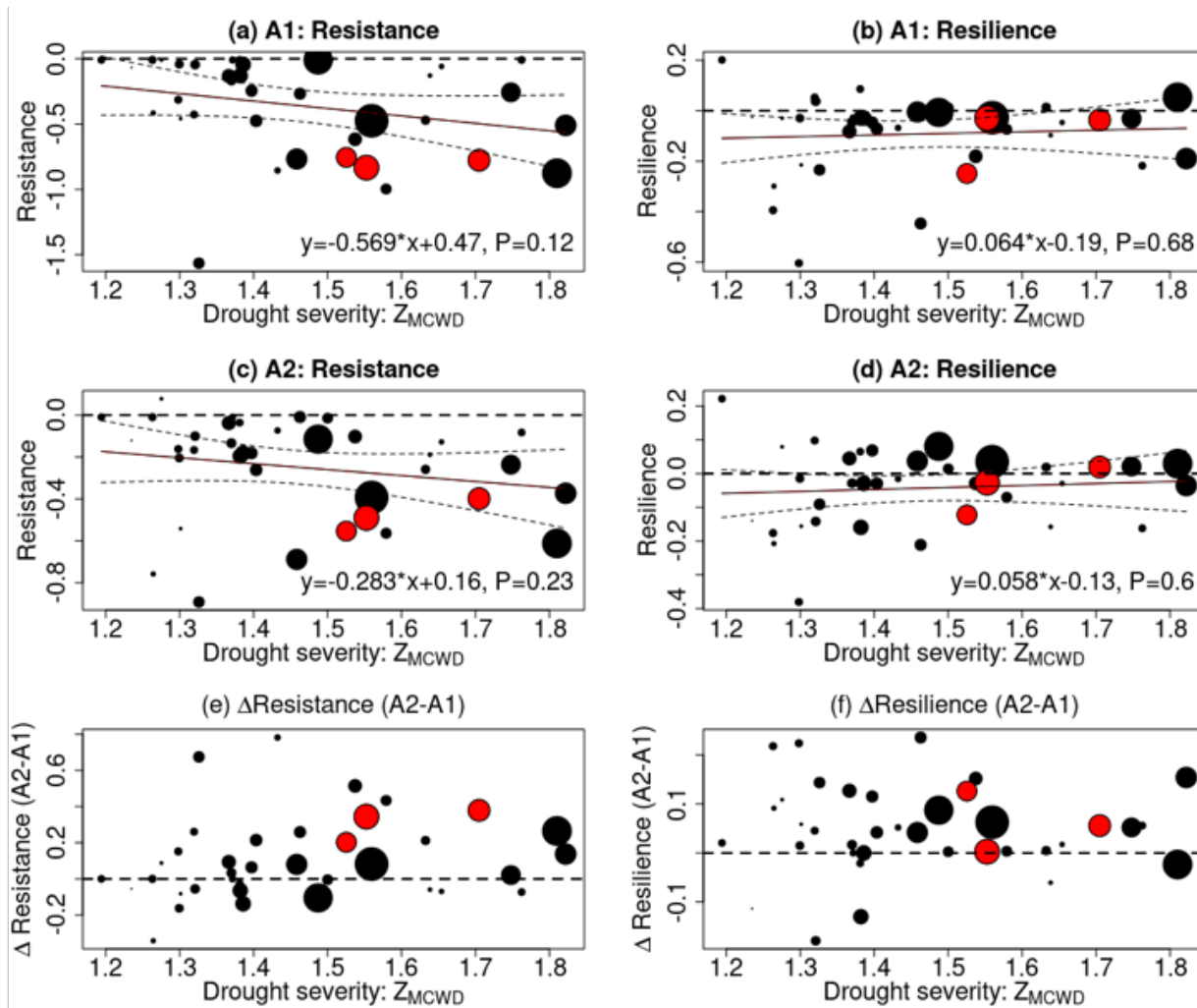
315 Figure 6. The effect of eCO 2 on drought recovery in aspects of resistance and resilience of net biomass carbon change. For 320 each drought event, the median resistance, resilience and drought severity of the drought-affected pixels ( Z_{MCWD} below -1) were calculated, shown as dots in each panel. Drought severity was defined by the Z_{MCWD} . The size of the dots indicates the area situated within the drought epicenter. The dots for 2005, 2010, and 2016 were color-coded in red. A trend fitting was applied to panels a-d, with its equation labelled and 95% confidence bound shaded. Resistance was computed, where lower values mean a more pronounced reduction in net biomass carbon sink during a drought. Resilience was computed, where positive values indicate complete recovery of the forest to pre-drought conditions, while negative values signify incomplete recovery. In panels a-d, a horizontal dashed line indicates a resistance and resilience value of zero. In panels e-f, a horizontal dashed line was drawn as well to denote no change in resistance or resilience under eCO 2 conditions.
