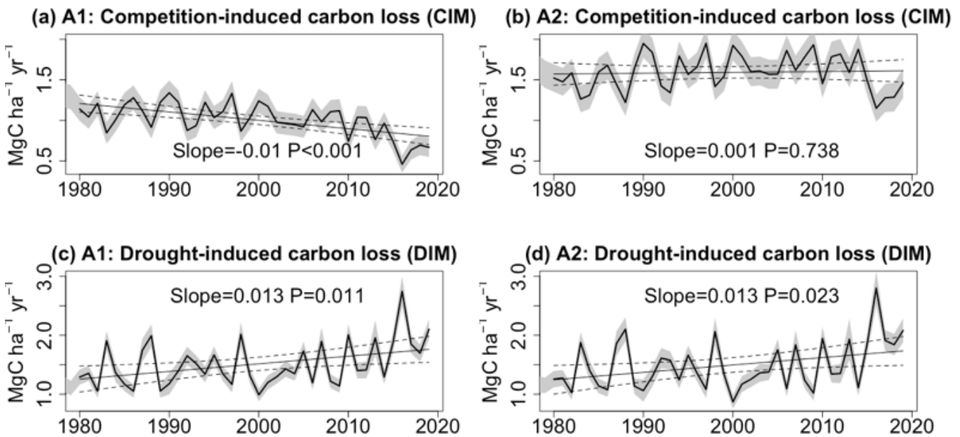
260 Figure 4. Trends in carbon losses due to (a,b) competition-induced (CIM) and (c,d) drought-induced tree mortality (DIM) with and without eCO 2 .
