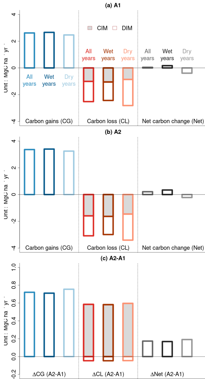
225 Figure 2. Basin-scale average of forest biomass carbon gains (CG), carbon losses (CL) and the net balance of gains minus losses (Net) over the last four decades. (a) eCO 2 , (b) constant CO 2 at pre-industrial level, (c) difference between eCO 2 and 230 constant CO 2 ( \Delta ). By convention gains are positive and losses are negative in (a) and (b). In panel (c), \Delta\text{CL} is calculated by the difference between absolute values of CL in panels (a) and (b). Dry years are defined as those in which the median of Z- transformed cumulative water deficit ( Z_{\text{MCWD}} ) at the basin scale fails below 0. For biomass carbon loss, CIM represents competition-induced self-thinning processes, and DIM represents drought-induced tree mortality processes.
