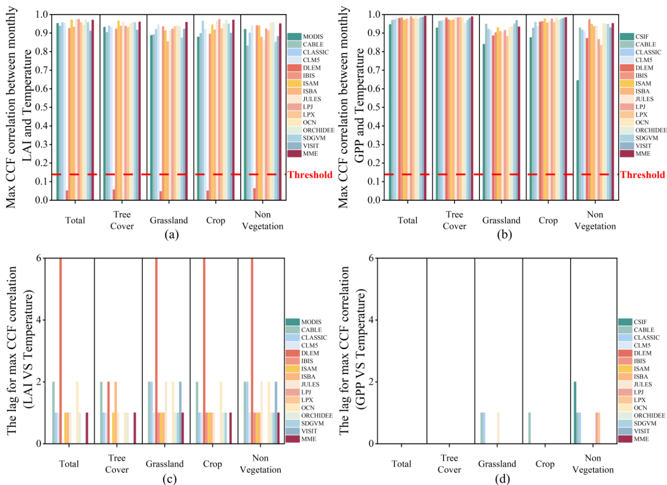
385 Fig. 11. The overall CCF of observed and simulated data with temperature. (a-b) The maximum CCF correlation between observed and simulated LAI and GPP, and temperature; (c-d) The lags between observed and simulated data corresponding to temperature. The red line indicates the correlation coefficient corresponding to the significance level ( p = 0.05 ). The values over the red line indicate that the LAI or GPP can capture the seasonality of the climate factor in phase.
