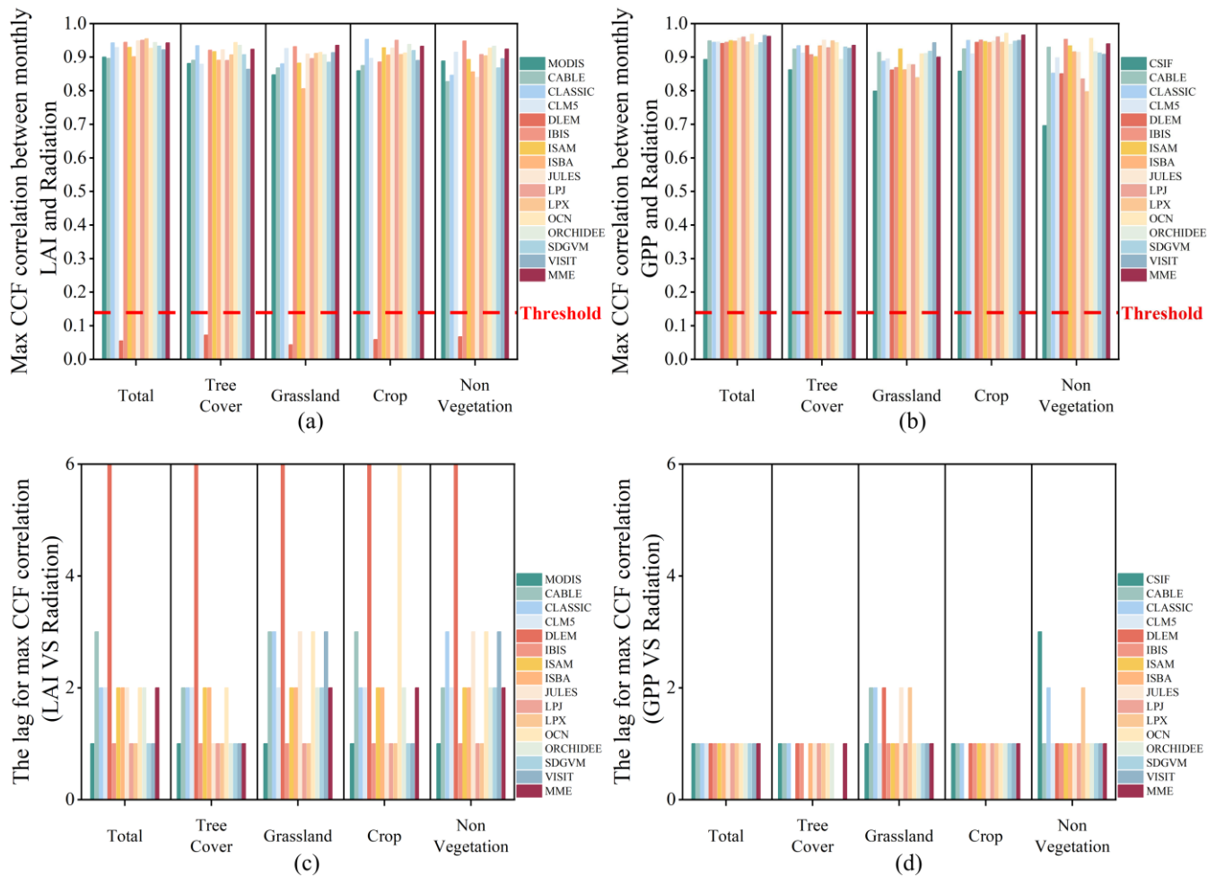
380 Fig. 10. The overall CCF of observed and simulated data with radiation. (a-b) The maximum CCF correlation between observed and simulated LAI and GPP, and radiation; (c-d) The lags between observed and simulated data corresponding to radiation. The red line indicates the correlation coefficient corresponding to the significance level ( p = 0.05 ). The values over the red line indicate that the LAI or GPP can capture the seasonality of the climate factor in phase.
