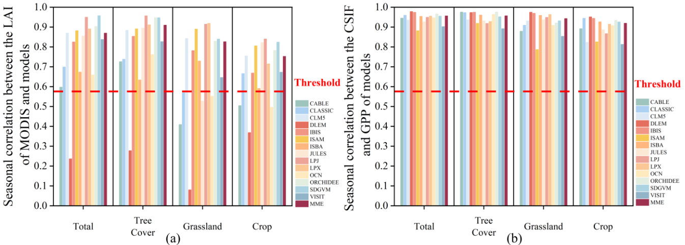
335 Fig. 6. The overall seasonal correlation between observed and simulated in China. (a) The seasonal correlation of simulated LAI with observed LAI over different land use types; (b) The seasonal correlation of simulated GPP with observed CSIF over different land use types. The red line indicates the correlation coefficient corresponding to the significance level ( p = 0.05 ). The values over the red line indicate that the model can capture the seasonality of MODIS LAI or CSIF in phase.
