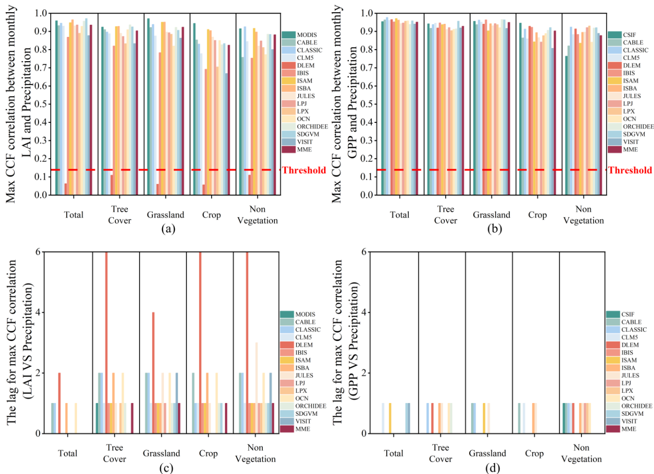
Fig. 9. The overall CCF of observed and simulated data with precipitation. (a-b) The maximum CCF correlation between observed and simulated LAI and GPP, and precipitation; (c-d) The lags between observed and simulated data corresponding to precipitation. The red line indicates the correlation coefficient corresponding to the significance level ( p = 0.05 ). The values over the red line indicate that the LAI or GPP can capture the seasonality of the climate factor in phase.
