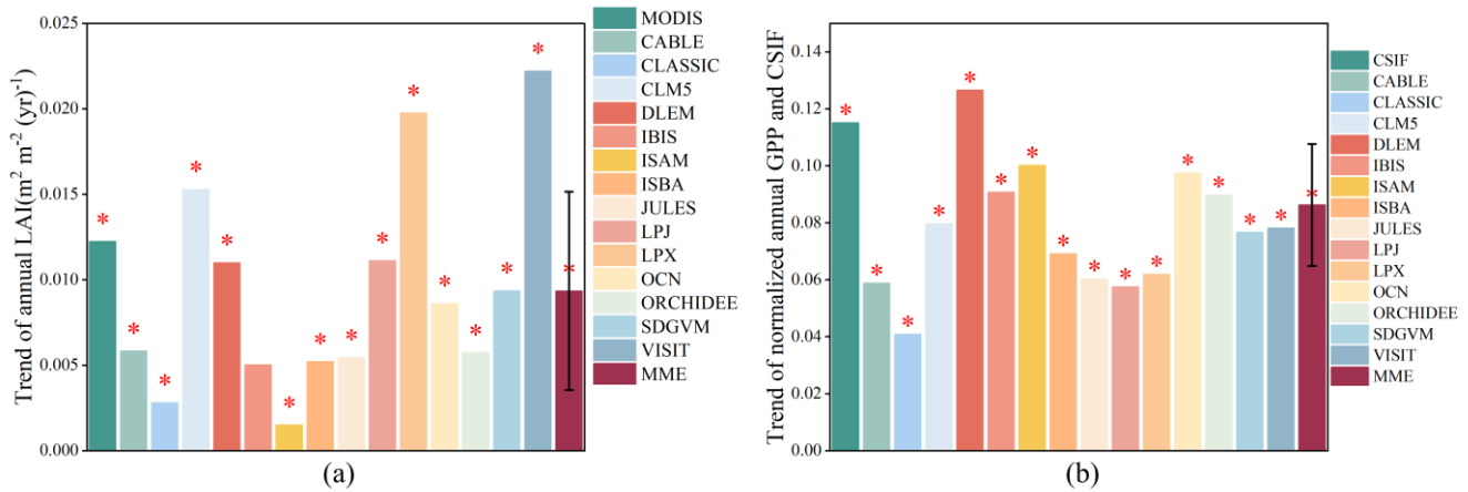
Fig.1. Overall annual average LAI and GPP trends in China during 2003-2019. (a) Annual trends in observed and simulated LAI; (b) Annual trends in observed and simulated GPP. The asterisk (*) indicates the significant trend ( p < 0.05 ). The error bar for MME is the standard deviation of the 14 modeled trends.
