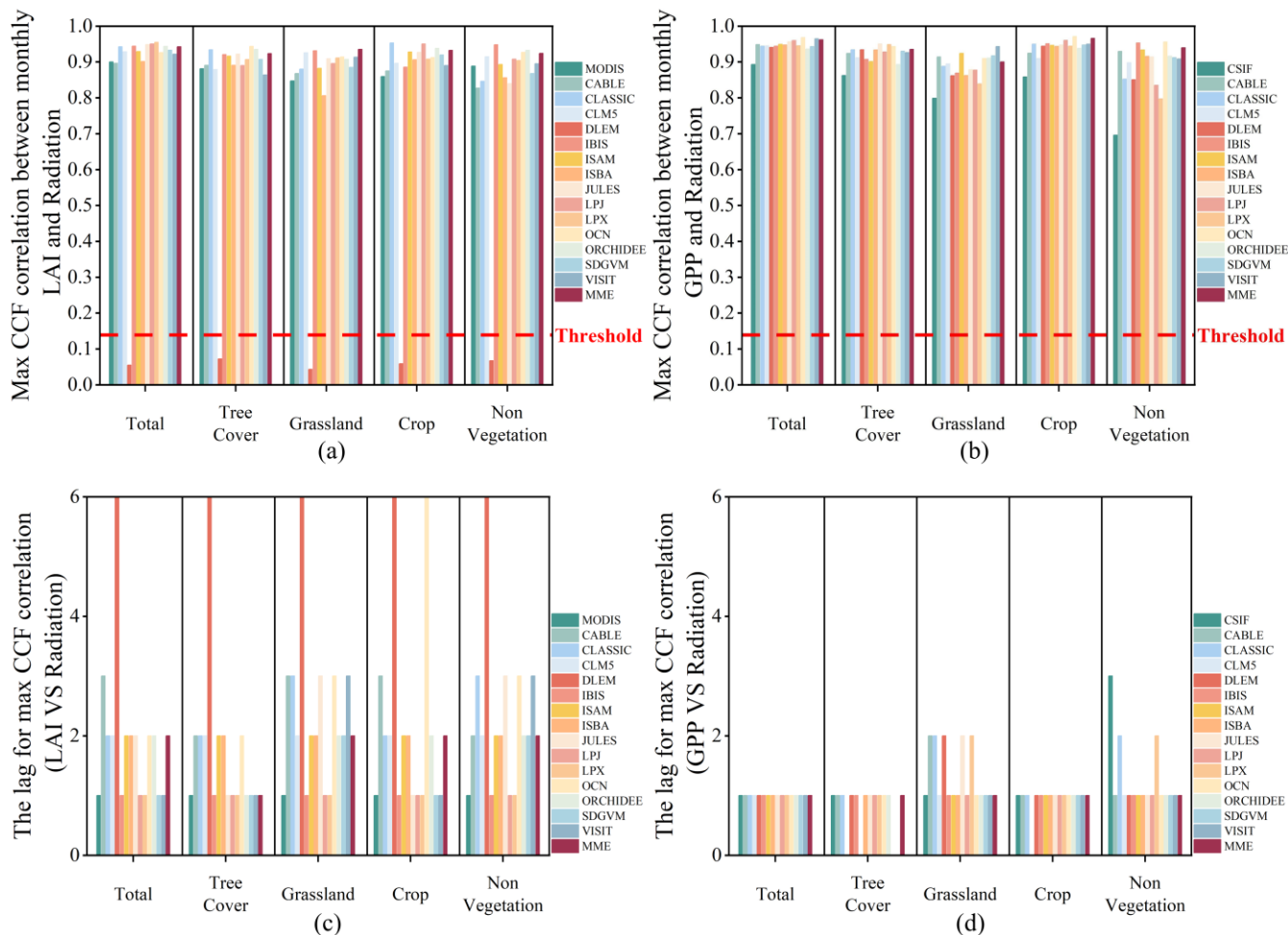
Fig. 10. The overall CCF of observed and simulated data with radiation. (a-b) The maximum CCF correlation between observed and simulated LAI and GPP and radiation; (c-d) The lags between observed and simulated data corresponding to radiation. The red line indicates the correlation coefficient corresponding to the significance level ( p = 0.05 ). The values over the red line indicated that the LAI or GPP can capture the seasonality of the climate factor in phase.
