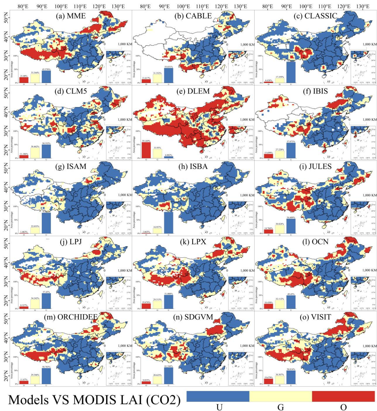
315 Fig. 5. Spatial distribution of sensitivity differences between the effects of CO 2 concentration on observed and simulated LAI in China. A paired t-tests with a sample size of 9 were conducted using a 3 × 3 sliding window to determine whether the effect of CO 2 concentration on the amount of simulated LAI change was not significantly different from the effect on the amount of observed LAI change (Good), was significantly smaller than the observed data (Underestimate), or was significantly larger than the observed data (Overestimate). U, G, and O represent 'Underestimate', 'Good', and 'Overestimate', respectively.
