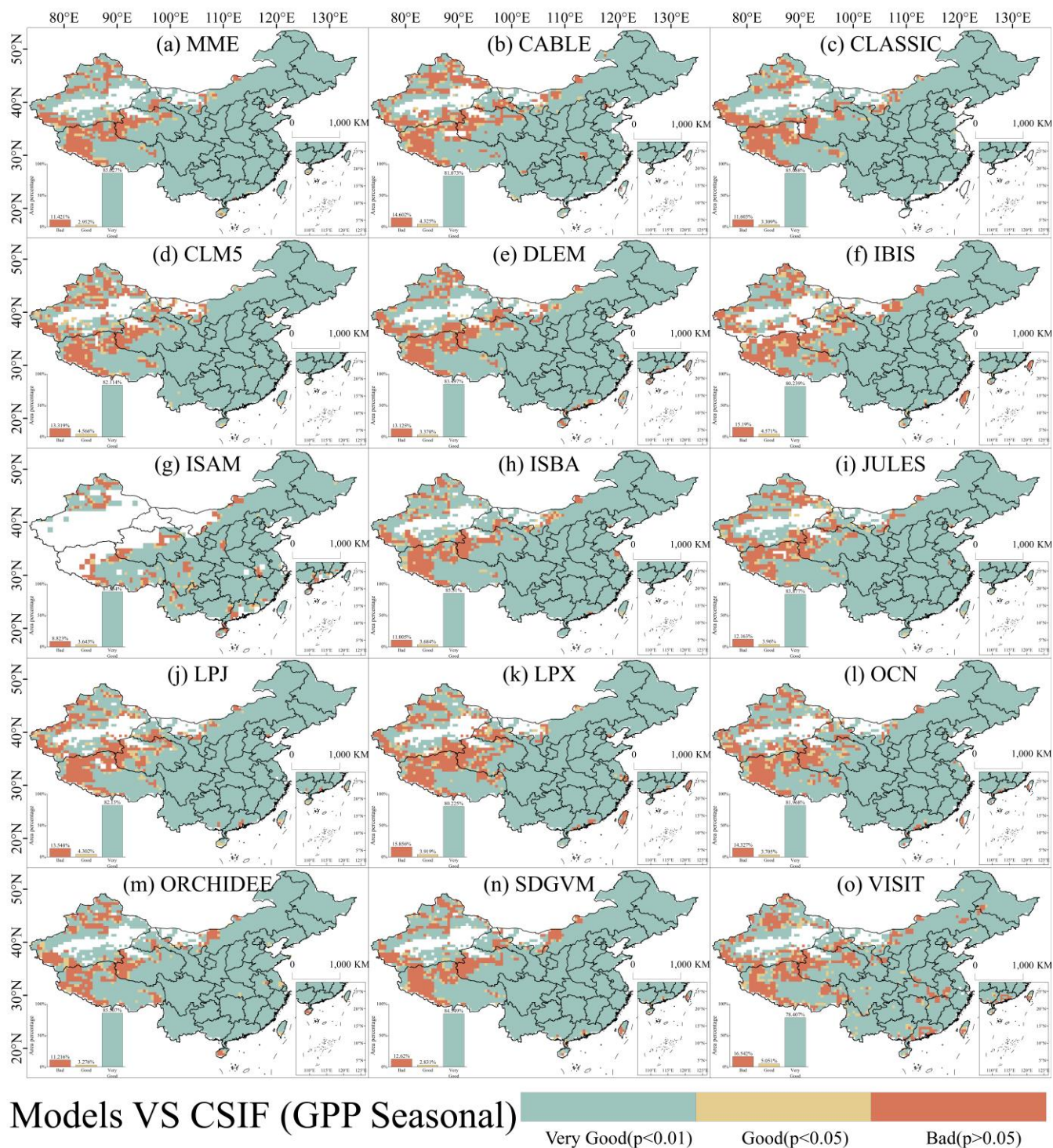
Fig. 8. Spatial distribution pearson correlations of the seasonality of observed and simulated GPP during 2003-2019 in China. Pearson correlations were using a 3 \times 3 sliding window to determine whether simulated seasonal GPP was highly significantly
