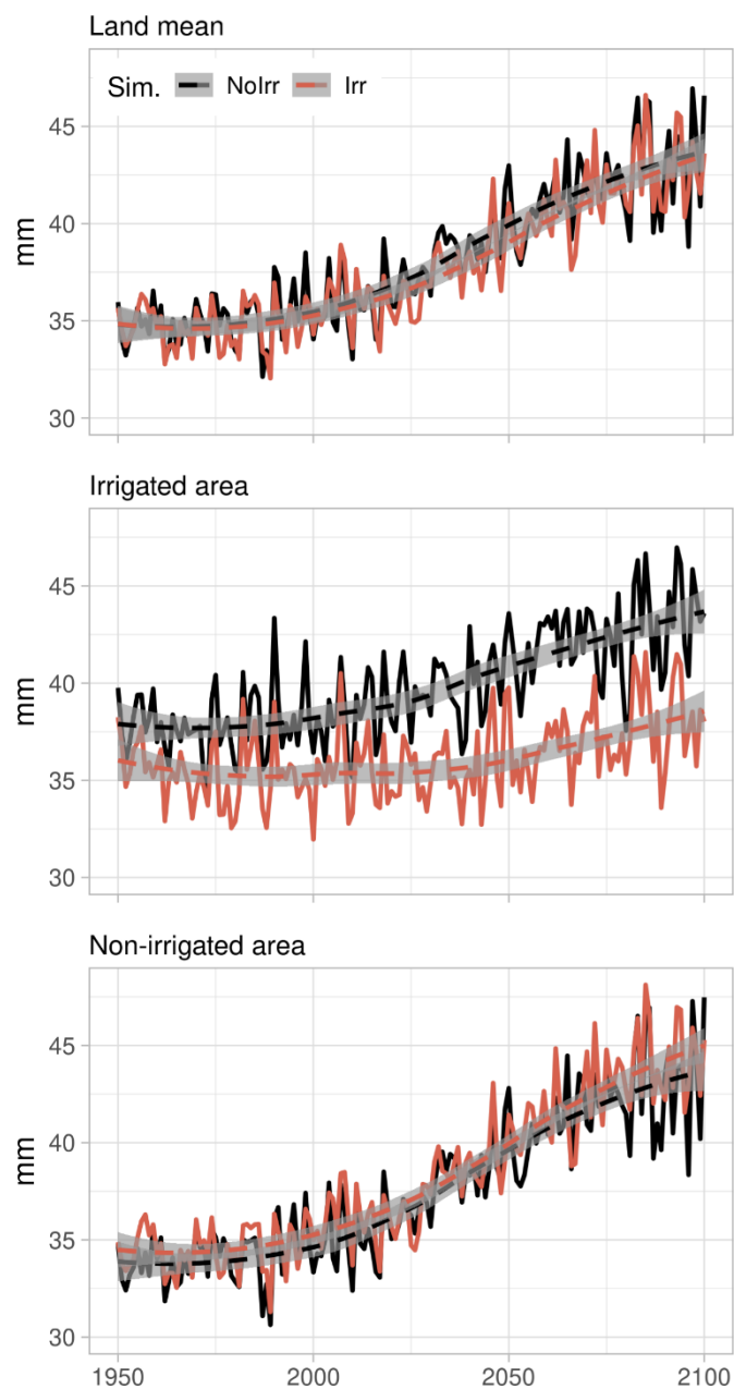
Figure 8: Time series of yearly groundwater storage (a, left column) and stream storage (b, right column). The first row corresponds to the average on land, the second row corresponds to the average in irrigated areas, and the third row corresponds to the average in non-irrigated areas. The dashed lines correspond to a fitted polynomial surface via local fitting.
