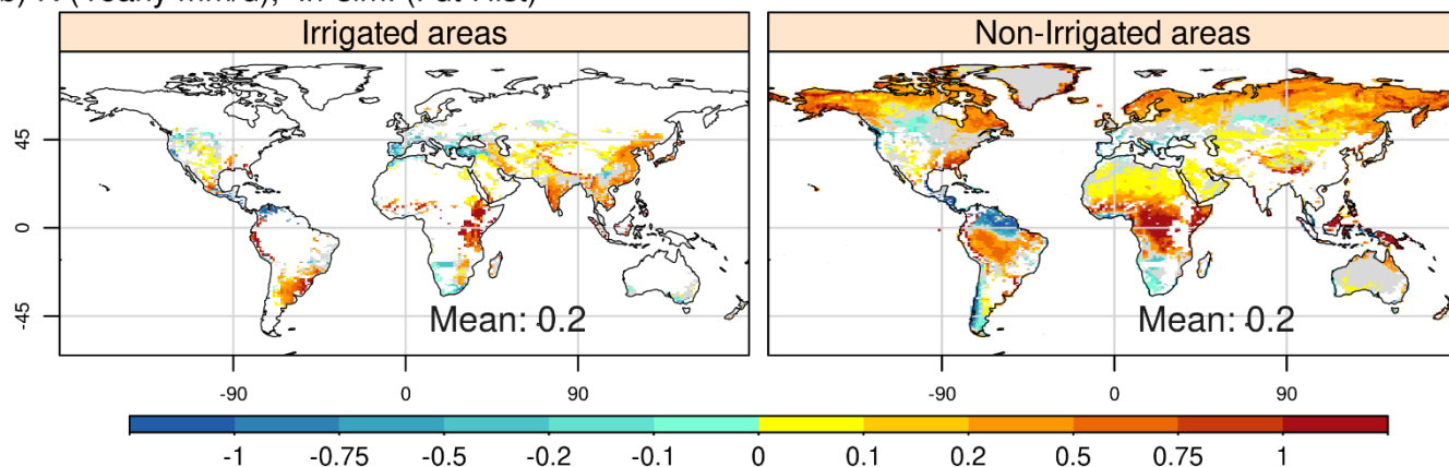
250 Figure 4: Map of the spatial distribution of yearly changes between future and historical periods for irrigated areas (left column) and non-irrigated areas (right column), for precipitation (a) and air temperature at 2 meters (b). The areas in gray correspond to a p value less than 0.05 according to Student's t test.
