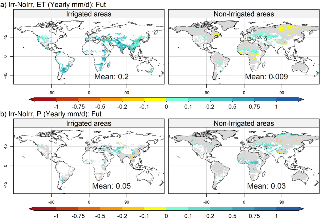
Figure 6: Map of the spatial distribution of yearly changes between the Irr and NoIrr simulations under future climate conditions for irrigated areas (left column) and non-irrigated areas (right column), for evapotranspiration (a) and precipitation (b). The areas in gray correspond to a p value less than 0.05 according to Student's t test.
