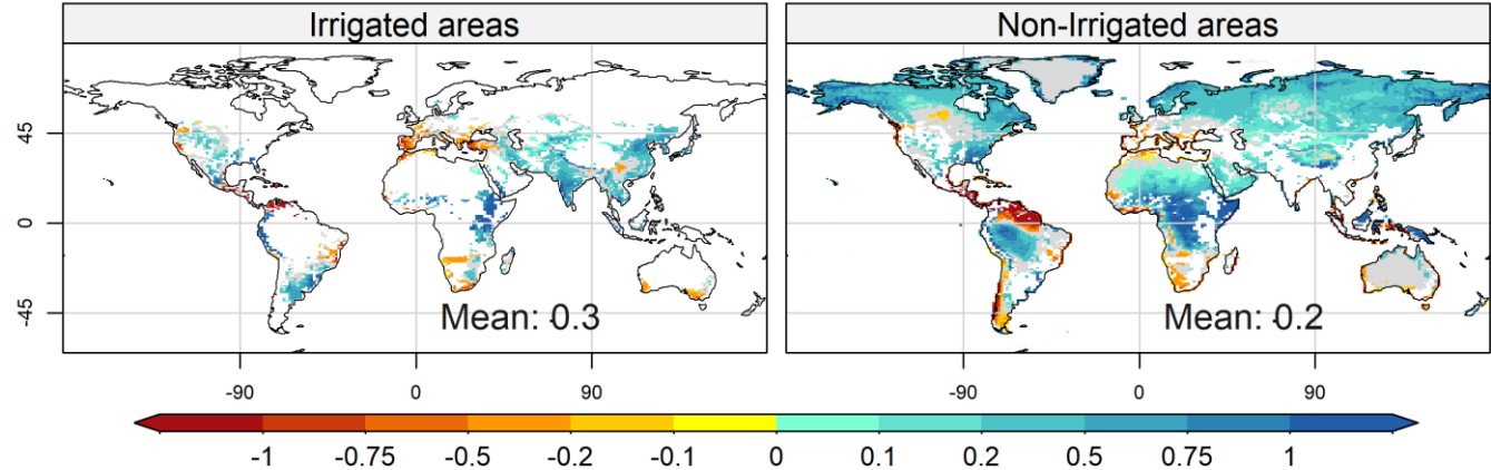
b) Tas (Yearly °C), Irr sim. (Fut-Hist)
