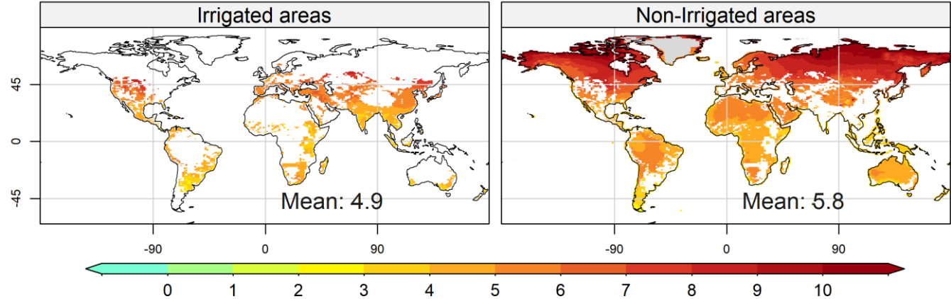
Figure 3: Map of the spatial distribution of yearly changes between future and historical periods for irrigated areas (left column) and non-irrigated areas (right column), for precipitation (a) and air temperature at 2 meters (b). The areas in gray correspond to a p value less than 0.05 according to Student's t test.
