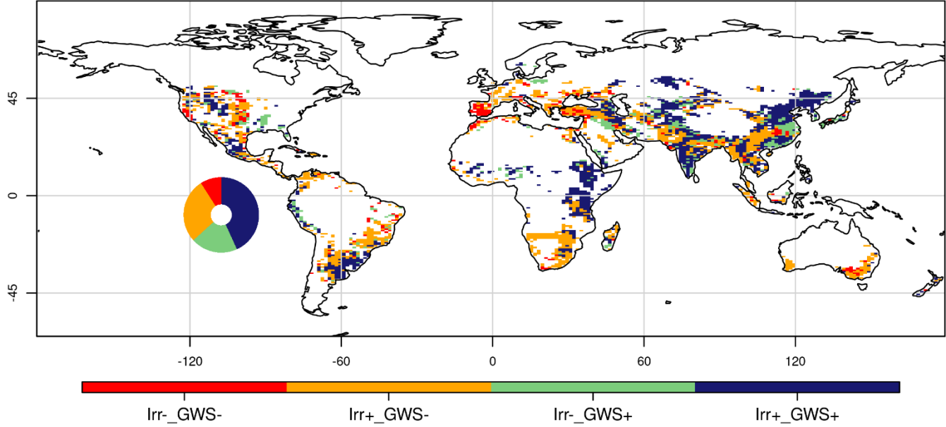
450 Figure 10: Joint changes between the future (Fut, 2050-2100) and historical (Hist, 1950-2000) periods for precipitation (P) and irrigation (Irr) in irrigated areas (a) and for groundwater reservoirs (GWS) and irrigation (Irr) in irrigated areas (b). The symbols + and - indicate positive and negative changes, respectively. The insets indicate the fraction of irrigated area by class.
