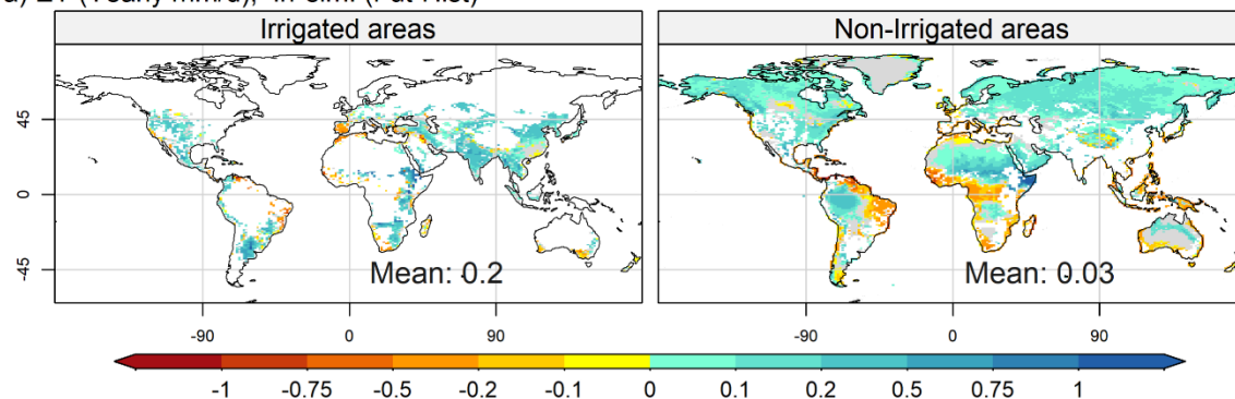
b) R (Yearly mm/d), Irr sim. (Fut-Hist)
