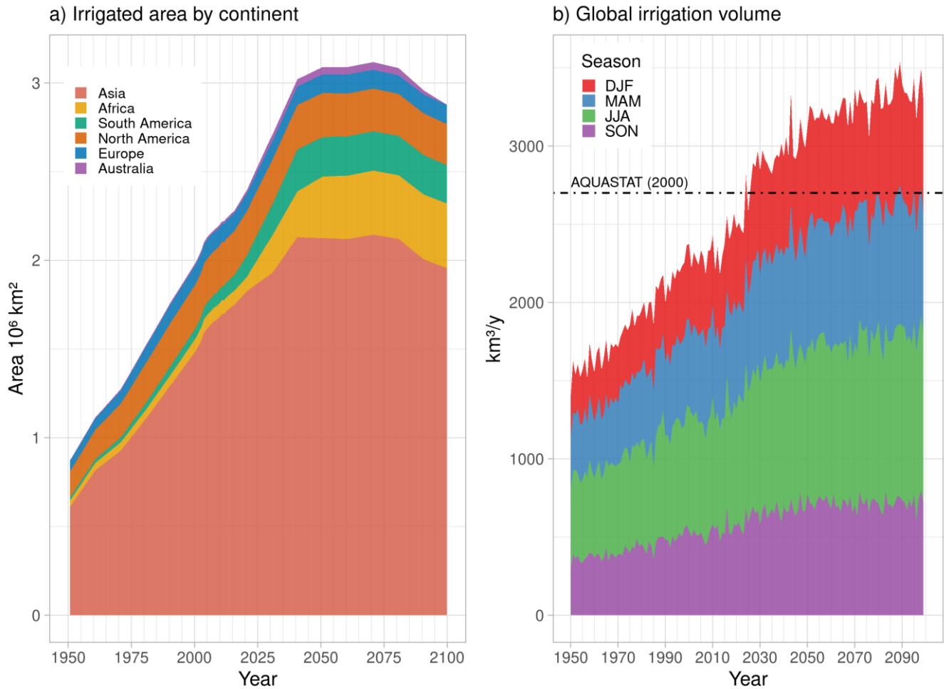
190 Figure 2: (a) Total irrigated area and by continent prescribed by LUHv2. (b) Total and seasonal irrigation volume at the global scale simulated by IPSL-CM6 in the Irr simulation. The black line represents the value reported by AQUASTAT around the year 2000 (Frenken and Gillet, 2012).
