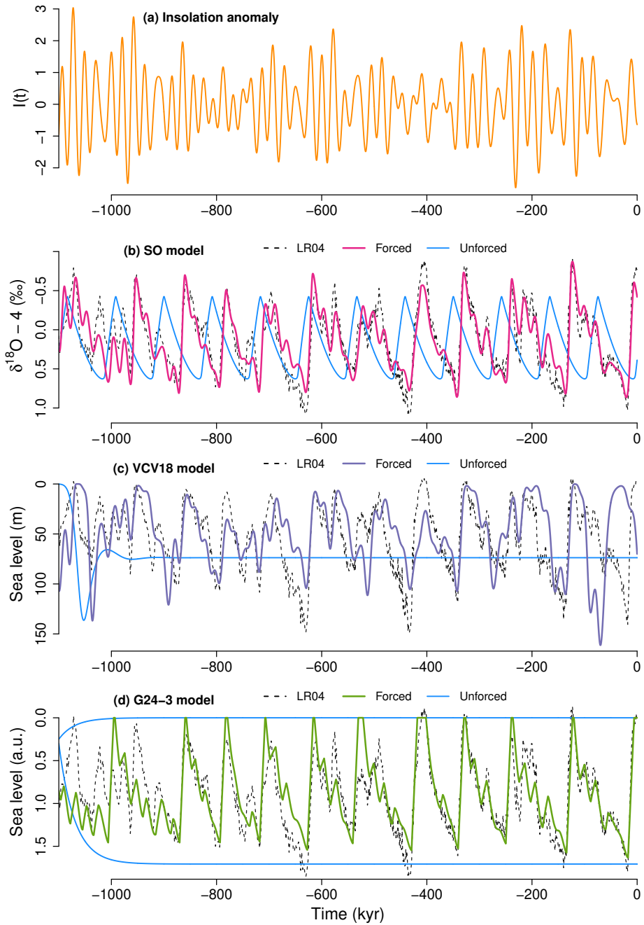
Figure 2. Forced and unforced simulations of glacial cycles over the last 1 Myr: (a) Standardized summer solstice insolation at 65^\circ\text{N} . (b) SO model with forcing (pink) and without forcing (light blue). (c) VCV18 model with forcing (violet) and without forcing (light blue). (d) G24-3 model with forcing (green) and without forcing (light blue). For all three models, the corresponding scaled versions of the paleoclimatic record are shown by the black dashed line.
