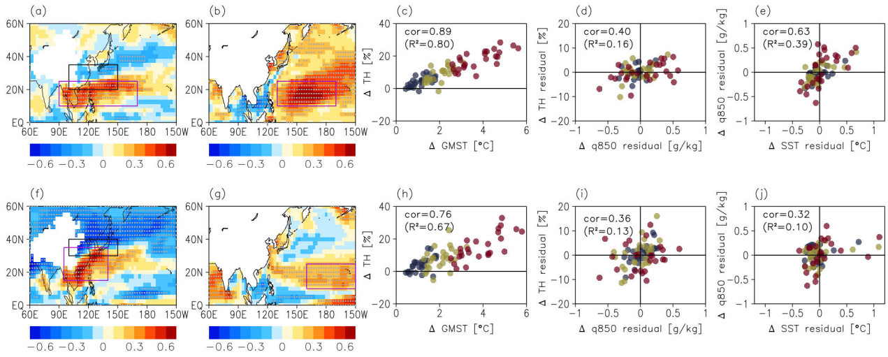
Figure 8. Analysis of global warming and regional SST influence on thermodynamic changes (TH) for the (a-e) northward migration and peak time (f-j). (a, f) Inter-model correlation patterns between the TH residual term and the 850hPa specific humidity (q850) residual. The black boxes indicate the East Asia region used for calculating the TH term. The purple boxes represent regions with high correlation between the TH residual and q850 residual (90–170°E, 10–25°N in a and 90–140°E, 15–35°N in f). (b, g) Inter-model correlation patterns between the area-averaged q850 residual (purple box from a and f) and the SST residual, with purple boxes highlighting SST regions that are strongly correlation with the area-averaged q850 residual. Scatter plots of (c, h) GMST vs. TH, (d, i) q850 residual vs. TH residual, and (e, j) SST residual vs. q850 residual. Navy, olive green, and dark red dots indicate SSP1-2.6, SSP2-4.5, and SSP5-8.5, respectively. Correlation coefficients are based on all models across scenarios. Refer to the main text for the detailed latitude-longitude range of the selected regions (black and purple boxes).
