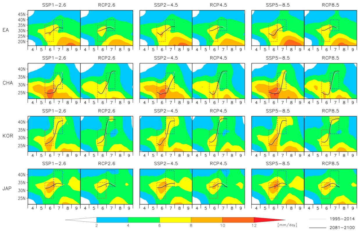
400 Figure 2. Time–latitude cross sections of pentad precipitation (mm/day) over East Asia (EA), China (CHA), Korea (KOR), and Japan (JAP) in a long-term period (2081–2100) from six future scenarios : Shared Socioeconomic Pathway (SSP)1-2.6, Representative Concentration Pathway (RCP)2.6, SSP2-4.5, RCP4.5, SSP5-8.5, and RCP8.5. Red and blue boxes represent the northward migration and peak time of monsoon rain bands, respectively. The gray and black lines follow latitudes with the 405 precipitation maximum in 1995–2014 and in 2081–2100, respectively. The red and blue boxes indicate the timing and latitude of northward migration and peak time, respectively.
