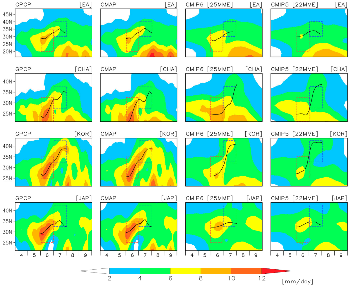
Figure 1. Time–latitude cross sections of pentad precipitation rates (mm/day) from 1995 to 2014 over East Asia (EA; 100–150°E), China (CHA; 110–120°E), Korea (KOR; 120–130°E), and Japan (JAP; 130–142°E) from the Global Precipitation Climatology Project (GPCP), Climate Prediction Center Merged Analysis of Precipitation (CMAP), Coupled Model Intercomparison Project Phase 6 (CMIP6) Multi-Model Ensemble (MME), and CMIP5 MME. Red and blue boxes represent the northward migration and peak time of monsoon rain bands, respectively. Black lines follow the latitude with the precipitation maximum ( dPR/dlat = 0 ). The red and blue boxes indicate the timing and latitude of northward migration and peak time, respectively.
