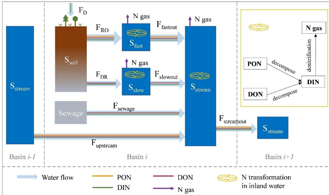
Figure 2. Schematic plot for the reservoirs and flows of water and N in LSM_Nlateral_Off. S_{soil} is the soil pool. S_{fast} , S_{slow} , S_{stream} are the “fast”, “slow” and stream water reservoirs, respectively. F_{RO} and F_{DR} are surface runoff and below-ground drainage (also called sub-surface runoff in other studies), respectively. F_{fastout} is the flow from fast reservoir to stream reservoir. F_{slowout} is the flow from slow reservoir to stream reservoir. F_{upstream} and F_{streamout} are the upstream inputs from basin i-1 and downstream outputs to basin i+1 , respectively. F_D is the wet and dry deposition of DIN from the atmosphere.
