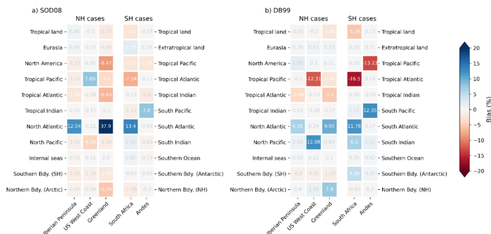
Figure 4: Bias in precipitation fraction (%) obtained using the basic configurations of the WaterSip-SOD08 and DB99 moisture source diagnostics, for trajectories generated with WRF input data (FLEXPART-WRF). Biases are computed subtracting the “true” outcomes of WRF-WVTs from the corresponding values of WaterSip-SOD08 and DB99.
