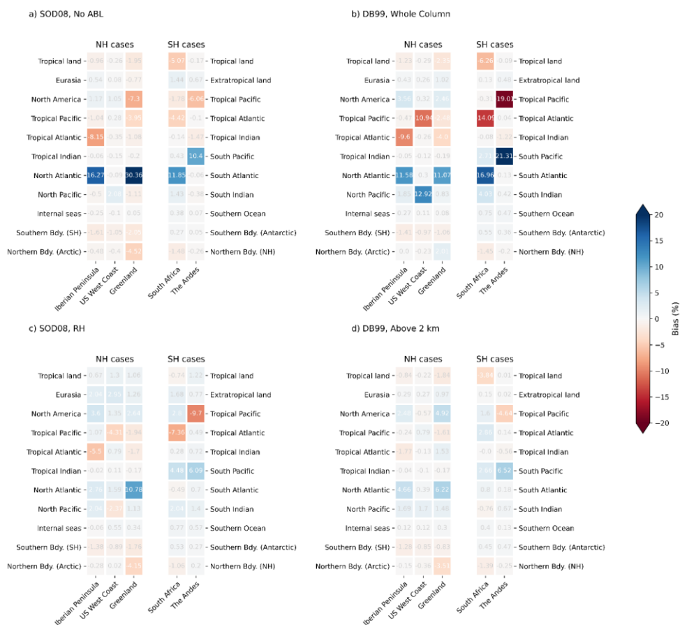
Figure 9: Bias in the precipitation fraction (%) obtained using the basic (a and b) and modified (c and d) configurations of the WaterSip-SOD08 (left) and the DB99 (right) diagnostics, for trajectories generated with FLEXPART forced with ERA5 input data (FLEXPART-ERA5). Biases are computed subtracting the “true” outcomes of WRF-WVTs from the corresponding values of the Lagrangian methodologies.
