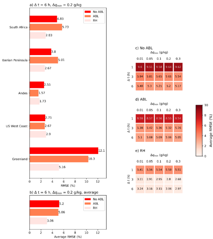
Figure 5: RMSE for the five AR-related precipitation events (panel a) and average of all of them (panel b) in the three tested configurations of WaterSipSOD08 , with the standard values of the specific humidity threshold and time step. On the right, average RMSE for a range of values of these parameters, in the case of the most basic configuration (No ABL, panel ca ), neglecting increments above the ABL (ABL, panel db ), and discarding decreases below a minimum relative humidity (RH, panel ce ).
