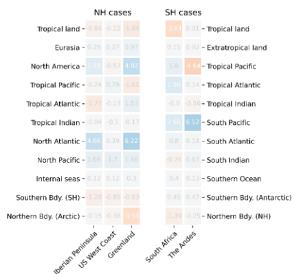
d) DB99, Above 2 km
