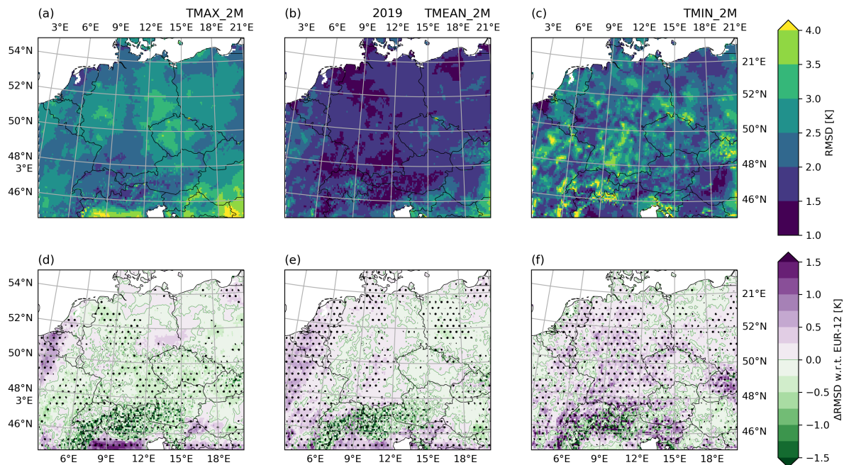
Figure 5. Added value assessment of the nested convective-permitting GER-3 simulation for June, July, August 2019 for daily maximum (left column), mean (center column), and minimum (right column) 2m temperature. (a-c): root mean square difference (RMSD) of daily 2m temperature to E-OBS of the GER-3 simulation. (d-f): Change of RMSD compared to the EUR-12 simulation (significant difference hatched, p < 0.05 ).
