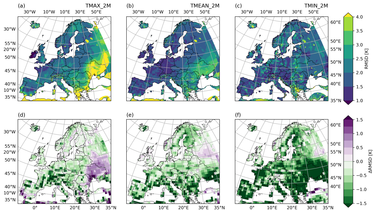
Figure 4. Added value assessment of the ICON EUR-12 simulation for June, July, August 2019 for daily maximum (left column), mean (middle column), and minimum (right column) 2m temperature. (a-c): root mean square difference (RMSD) of the simulated daily 2m temperatures by ICON EUR-12 to E-OBS. (d-f): Change in RMSD achieved by dynamical downscaling; the green colours correspond to the reduced squared error of daily temperatures.
