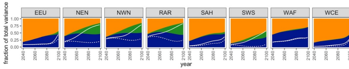
Figure A3: Same as Figure 7 but for RMS > 0.2 rather than 0.1.
