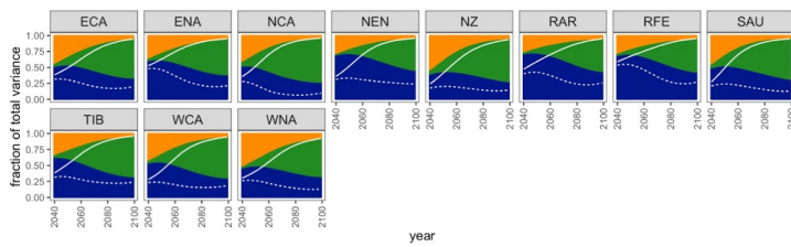
Figure A2: Same as Figure 6 but for RMS > 0.2 rather than 0.1
