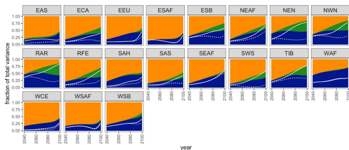
Figure 7: Same as Figure 6 but for precipitation.
