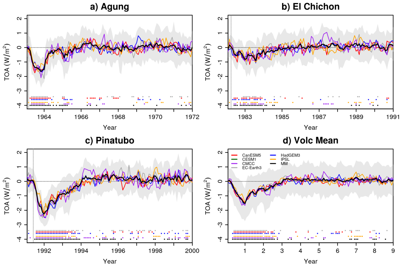
Figure 2. Global mean top-of-atmosphere radiation response ( \text{W/m}^2 ) to the volcanic eruptions (DCPP-A minus DCP-C). The ensemble mean for each model and the multi-model mean are shown. The shading is the multi-model member spread calculated as the 10 th and 90 th percentiles of the entire ensemble. Filled squares at the bottom part of the figure indicate statistically significant differences (see methods). The vertical grey dashed lines indicate the approximate time of the eruptions. The data for CESM1-1-CAM5-CMIP5 was not included since it is not available. Figure inspired by Zanchettin et al. (2022).
