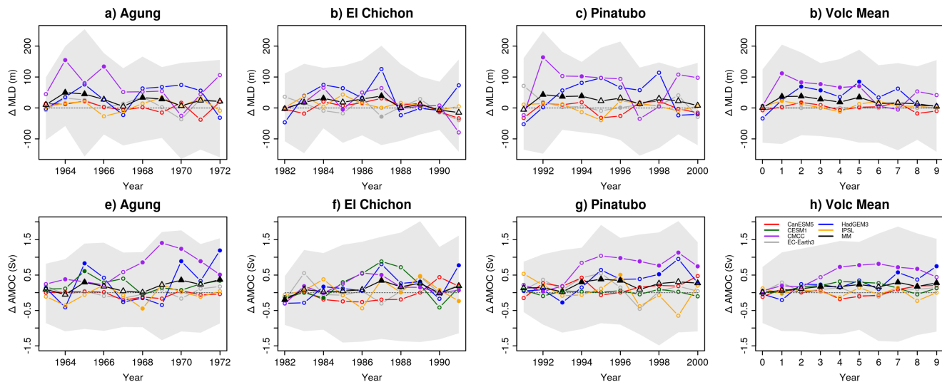
Figure 16. Volcanic response (DCPP-A minus DCPP-C) of the mixed layer depth in the Subpolar North Atlantic ( 50^{\circ}\text{N} - 65^{\circ}\text{N} , 60^{\circ}\text{W} - 35^{\circ}\text{W} ) in February-March-April (top row) and the annual mean overturning stream-function averaged over 30^{\circ}\text{N} - 50^{\circ}\text{N} and 1000m-2000m (bottom row). Filled circles/triangles indicate statistically significant differences (see methods). The ensemble mean for each model and the multi-model mean are shown. The shading is the multi-model member spread calculated as the 10 th and 90 th percentiles of the entire ensemble. The mixed layer depth for CESM1-1-CAM5-CMIP5 was not available and therefore could not be included.
