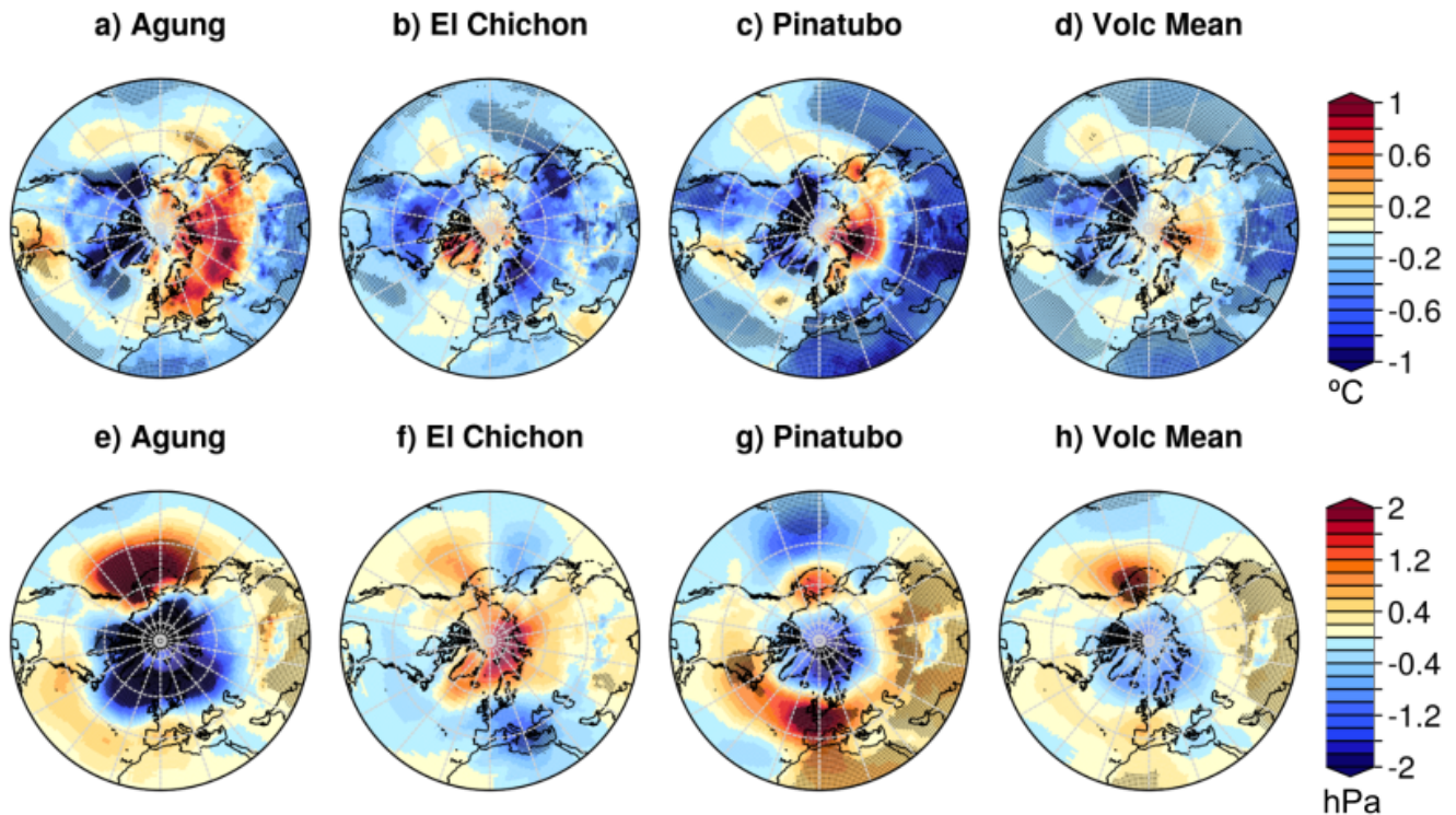
Figure 9. Multi-model and multi-eruption response (DCPP-A minus DCP-C) of surface air temperature (a-d) and sea level pressure (e-h) in the first boreal winter (DJF) following the volcanic eruptions. The ensemble mean for each model and the multi-model mean are shown. Shading indicates statistically significant anomalies.
