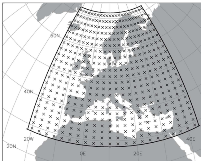
Figure 2: Domain for classification of synoptic circulation patterns: crosses show sample points every 2° in latitude and every 3° in longitude directions, 22x22 grid points in total. The solid black line shows the outer edge of the domain.
