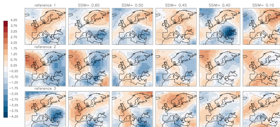
Figure 6: Examples of three synoptic patterns zg_a (left column “reference”). Each row contains examples of alternative synoptic patterns with the SSIM -value to the “reference”. Contour lines show the amplitude of anomalies with interval of 1.
