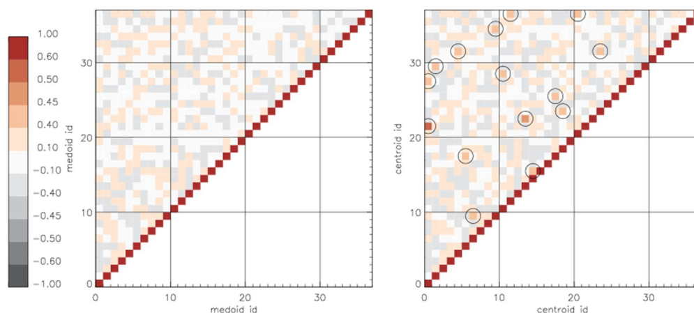
710 Figure 11: Matrix of pairwise similarity values for 37 classes derived with TH_{merge}=0.40 . Left panel: the matrix of SSIM for cluster medoids. Right panel: the matrix of SSIM for cluster centroids. Circles show similarity values greater than 0.40. The only upper left half of each matrix is shown due to the symmetry; diagonal elements have SSIM=1 .
