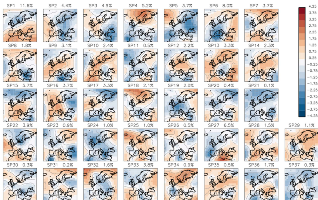
610 Figure 8: SP-classes (anomalies of geopotential height) obtained on the “reference data” (ERA-Interim Reanalysis, 1979-2018) with the threshold for similarity TH_{merge}=0.40 . Frequencies of SP-classes are shown above the corresponding plots.
