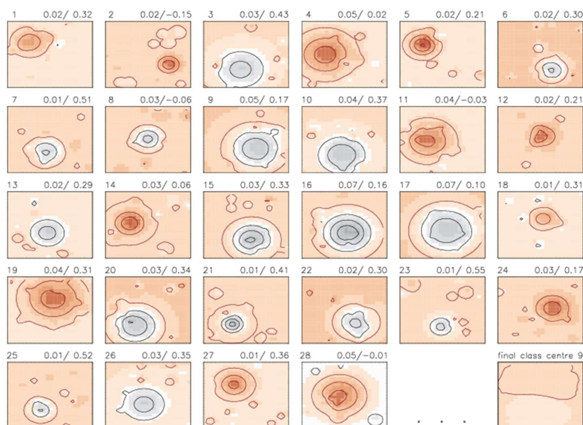
Figure 5: An example of a “snowball”-class resulted from the classification k-mean-MSE : class centre 9 (bottom right plot) has very weak structure, whereas its first 28 elements (only shown as examples out of 132) have strong anomalies of mixed sign and placed in various locations of the domain. Values of MSE and SSIM for an element to the class centre 9 are shown above plots for each element in form \langle \text{MSE} \rangle / \langle \text{SSIM} \rangle .
