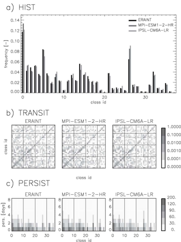
815 Figure 15: Examples of statistics for the reference data and two CMIP6-models: a) HIST – histogram of frequencies for each SP-class; b) TRANSIT matrices for each pair of SP-classes; where diagonal elements show transition for the same class i.e. persistence, c) PERSISTENCE matrices that show number of events when each SP-class persisted for 1,2, ..8 days (this statistic is shown in absolute values - non-normalized – for better readability).
