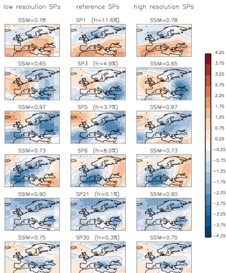
Figure 13: Examples of SP-classes on three spatial resolutions. The middle column shows reference SPs built from the “reference data” (2°x3°, 22x22 grid cells) with their frequencies (%). The left-side column shows corresponding patterns on the low-resolution (4°x6°, 11x11 grid cells), the right-side column - on the high-resolution (1°x1.5°, 44x44 grid cells). Both plots for low- and high-resolution counterparts show the SSIM-value to the reference SP-class on top of each plot.
