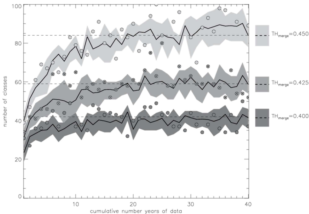
595 Figure 7: Number of classes depends on the threshold TH_{merge} and on the amount of clustered data. For each tested value of TH_{merge} the black solid line shows the mean number of classes computed on 61 classifications (1 with “reference data” + 60 with “randomized data”); the shaded area shows the range of one standard deviation from the mean. The circles show numbers of classes from classifications with the “reference data”; circles with crosses highlight class numbers with TH_{merge}=0.425 . The horizontal dashed lines show the mean number of classes for each TH_{merge} -value computed on the “reference data” of 40 years.
