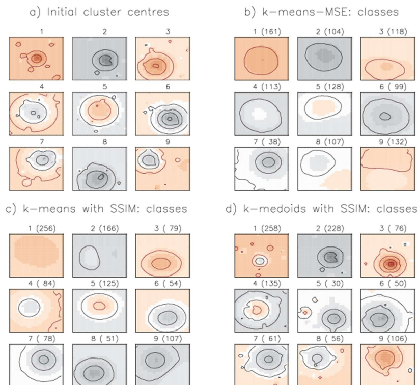
310 Figure 4: Cluster centres: a) derived by HAC -algorithm and used for the subsequent initialization of the partitioning algorithms, resulted from b) k-means-MSE classification, c) k-means-SSIM classification, and d) k-medoids-SSIM classification. Contour lines show the amplitude of negative (black) and positive anomalies (red) with interval of 0.25. In panels b), c) and d) above each plot numbers of elements (in brackets) in each class are shown.
