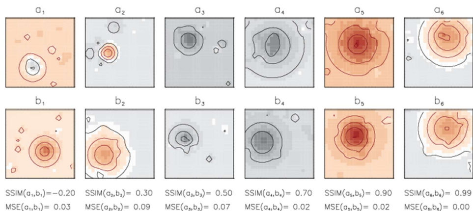
170 Figure 1: Examples of synthetic data fields. Fields are shown pairwise (a 1 -b 1 , a 2 -b 2 ,...) for demonstrating how visually perceived similarity is quantified in terms of SSIM and MSE given under the lower plot for each pair. Contour lines show the amplitude of negative anomalies (black) and positive anomalies (red) with interval of 0.25. Pairs are ordered by their SSIM-values from a dissimilar pair (on the left) to a strongly similar pair (on the right). Note: smaller MSE does not guarantee larger SSIM-values as for the pair a 1 -b 1 .
