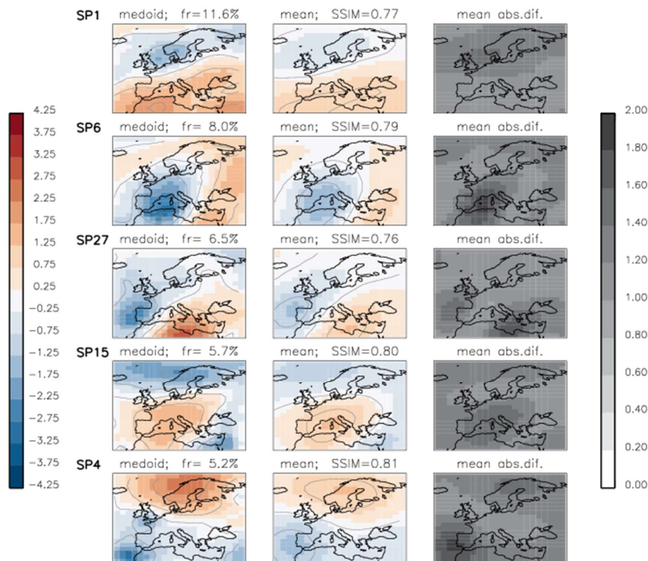
805 Figure 14: Medoids (left column), means/centroids (centre column) and their Mean Absolute Difference (right column) for five most frequent SP-classes. Frequency of each SP-class is shown on top of each medoid plot, SSIM between medoid and centroid is shown on the top of each plot of the mean.
