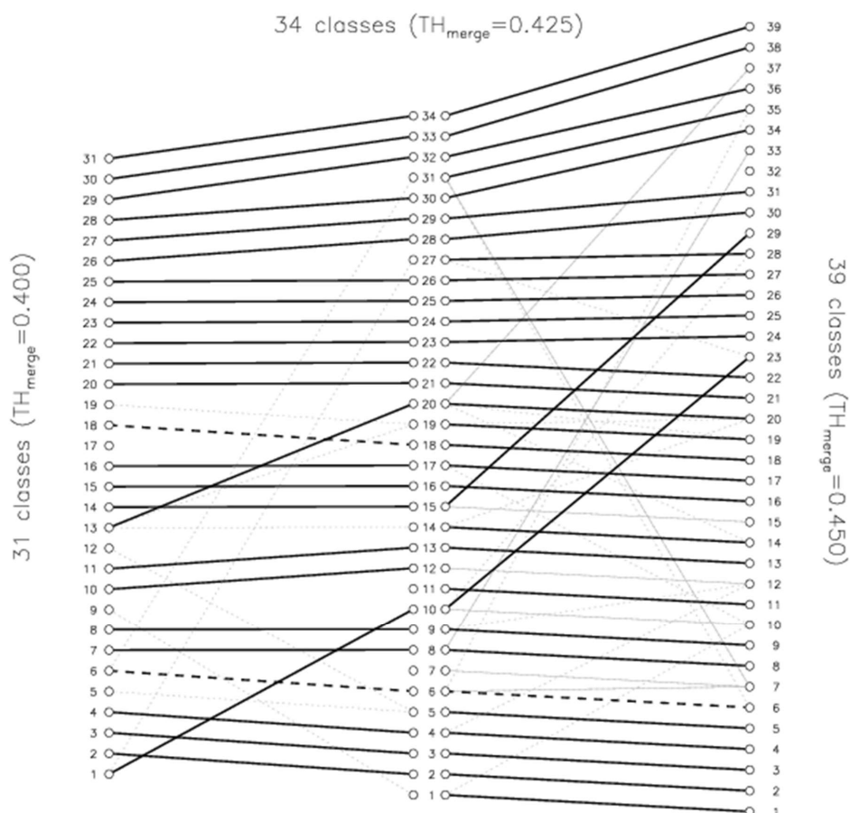
660 Figure 10: Similarity between classes derived with different merging threshold: (left) 31 classes obtained with TH_{merge}=0.40 , (middle) 34 classes with TH_{merge}=0.425 , and (right) 39 classes with TH_{merge}=0.45 . Black thick lines connect identical classes ( SSIM=1 ), black dashed lines connect "strongly similar" classes ( 0.60 \leq SSIM < 1 ), grey lines connect similar classes ( 0.40 \leq SSIM < 0.60 ), where connections with 0.40 \leq SSIM < 0.425 are dashed. Following the black solid lines from left-to-right: 23 classes retain their medoids.
