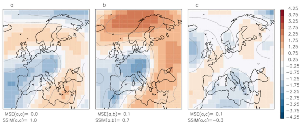
Figure 3: The pairs of geopotential anomaly fields a - b and a - c have same small MSE=0.1 but are strongly different in terms of SSIM: SSIM(a, b) = 0.7 means fields a and b are similar, SSIM(a, c) = -0.3 means fields a and c are dissimilar. Contour lines show the amplitude of anomalies with interval of 1.
