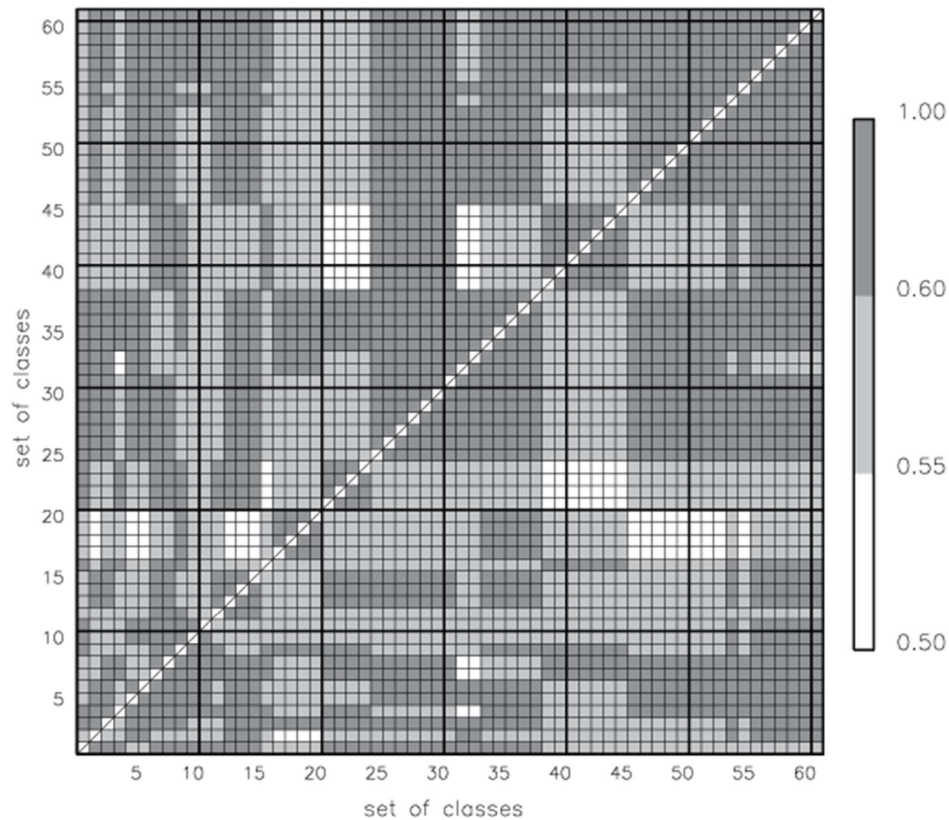
740 Figure 12: Mean weighted similarity, mwSSIM , for each of 61 sets of classes to each other. Each set of classes was derived on minNYR=30 years of input data. The diagonal elements are not shown because mwSSIM=1 of a set of the classes to itself. The matrix is not symmetric: mwSSIM(k,l) \neq mwSSIM(l,k) as the sets of classes k and l may have different number of classes.
