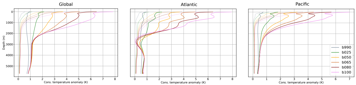
Figure 10. Global-mean-Mean profile of the ocean temperature anomaly at depth with respect to the pre-industrial climate for the global ocean (left), Atlantic (middle) and Pacific (right) . The dotted lines represent the starting point of the simulations, the solid ones the final state. Shown are 30-yr averages, the conservative temperature variable has been used.
