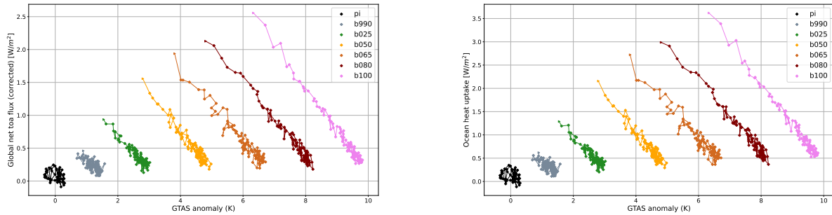
Figure 4. Global-Left panel: global net energy imbalance at TOA (corrected for spurious model energy sources) vs GTAS anomaly of the different simulations. Right panel: global surface ocean heat uptake vs GTAS anomaly. Dots represent 10-year averages.
