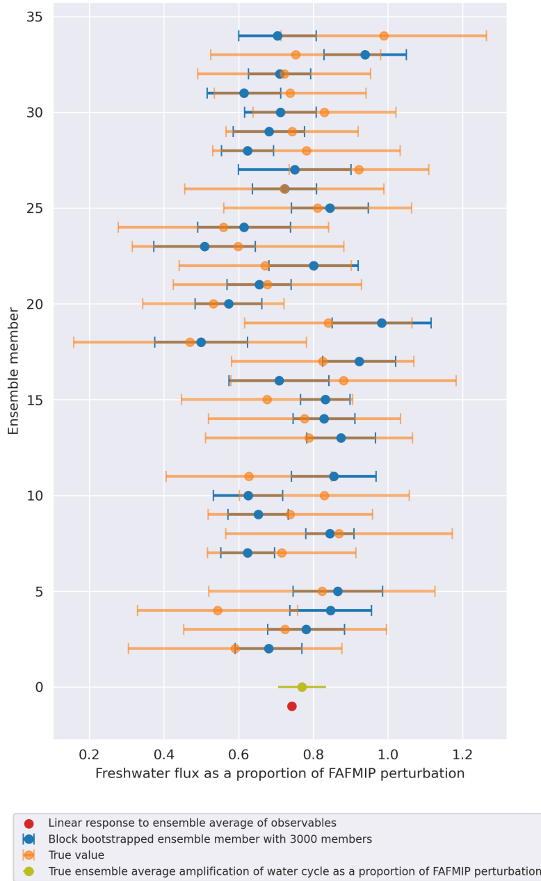
Figure S6: Freshwater flux responses over the period 2011 to 2055 (RCP8.5 pathway) for individual CESM ensemble members following our methodology described in text (blue) compared to truth from E-P model fields (orange). Here, we only plot members which met salinity significance criteria, and thus dropped 3 members.
