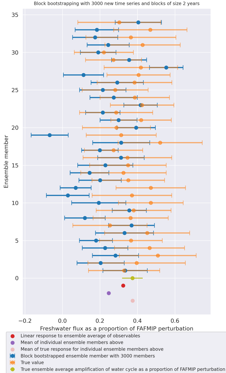
Freshwater flux as a proportion of FAFMIP perturbation for each ensemble member
