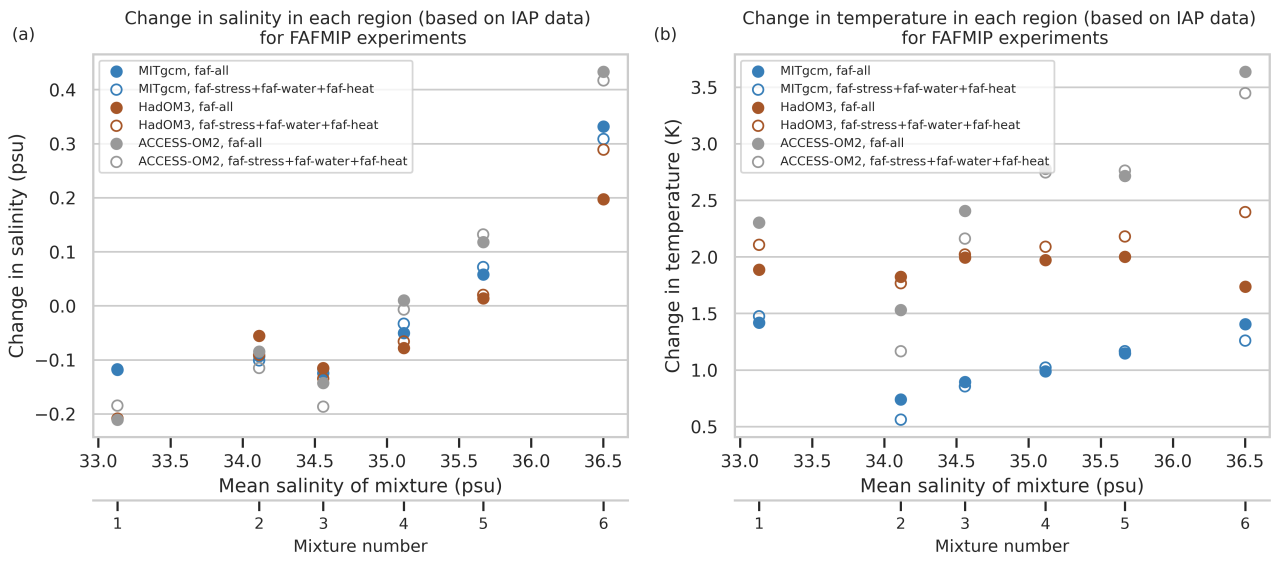
Figure S3: Comparing the surface salinity response (a) and surface temperature response (b) in each region between two cases: the sum of the response when forcings are applied individually (faf-stress+faf-water+faf-heat) and the response to all forcings applied at once (faf-all). The response is defined as the difference between the last decade of a forced run and the last decade of the control run. The response is largely linear with the exception of the sixth mixture for the HadOM3 model. Here the regions are found by a GMM fit to the IAP data.
