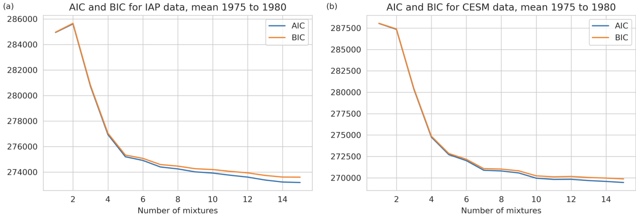
Figure S1: The AIC and BIC versus number of mixtures. Panel a uses the IAP surface salinity distribution south of 65N over the period 1975 to 1980, while panel b uses the CESM ensemble mean surface salinity distribution over the same region and time period.
