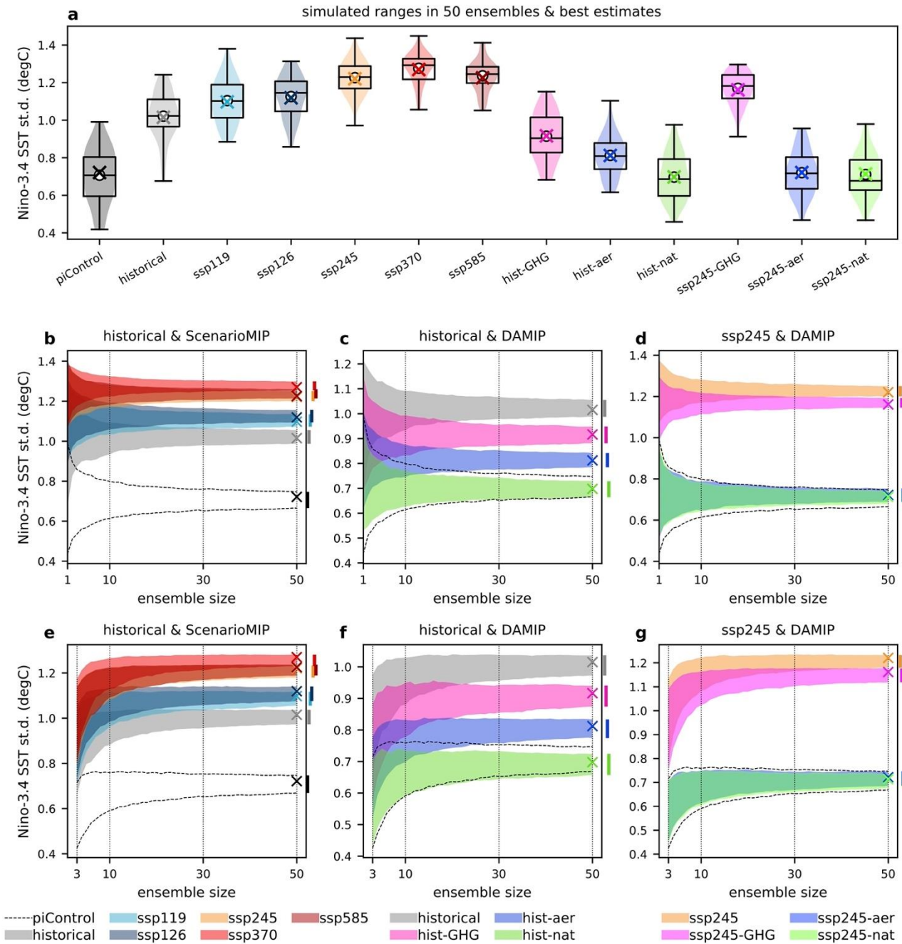
605 Figure 10: The standard deviations of the 10-year high-pass filtered Niño-3.4 SSTa and SSTi averaged in December-January- February. (a) The best estimates derived from the 50 members of SSTi (cross marks) and the single-member-trend removed estimates derived from each member of SSTa (box-whisker plots for the ensemble medians, interquartile ranges, and minimum- maximum ranges; opened circles for the ensemble mean; shadings for probability density functions). The ensemble-size (N) 610 dependence of the 95% ranges of (b-d) the ensemble means of randomly selected SSTa from the 50 members and (e-g) the SSTi as the departures from the ensemble means of randomly selected members. The cross marks indicate the best estimates. The vertical bars outside of each panel show the 95% ranges at N=50.
