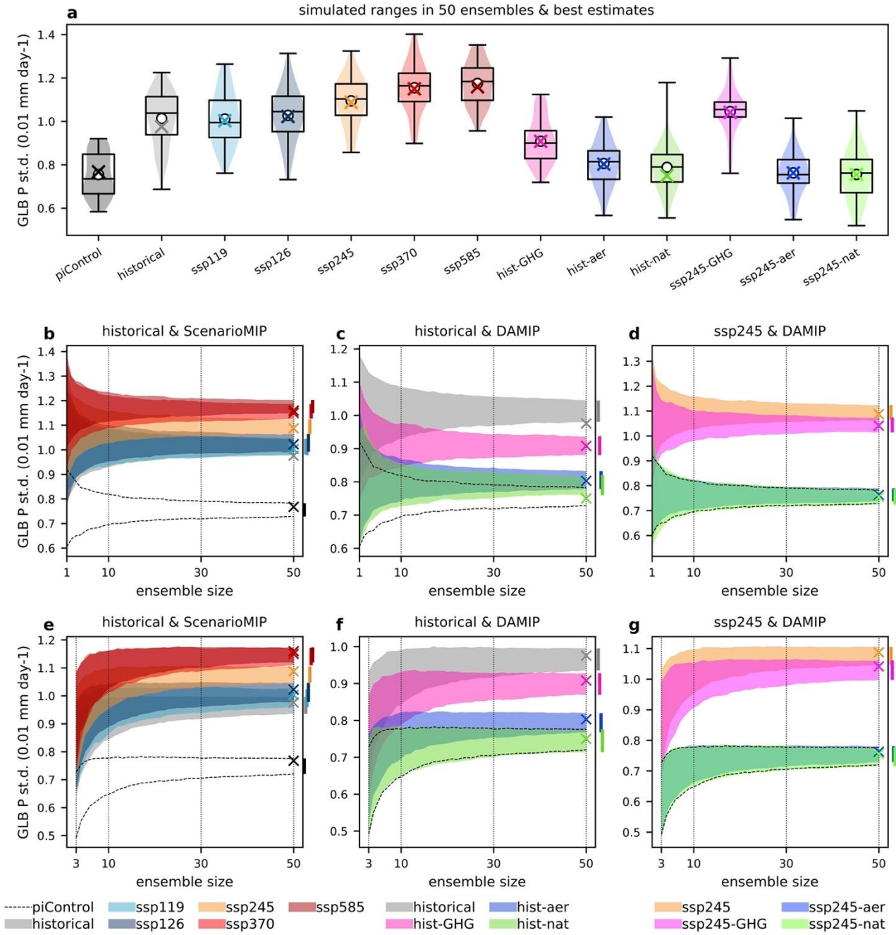
615 Figure 12: As in Figure 10 but for the 10-year high-pass filtered global annual mean P (0.01 mm/day).
