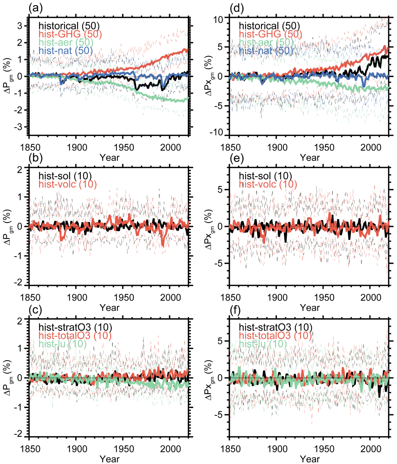
Figure 2: Global mean changes in P (left, %) and Px (right, %) of historical all and single forcing experiments relative to the 1850-1900 averages of the ensemble-mean historical all forcing simulations. Solid lines are the ensemble means. Thin dashed lines denote the minimum and maximum values of the ensemble members. Numbers in parentheses indicate the ensemble sizes.
