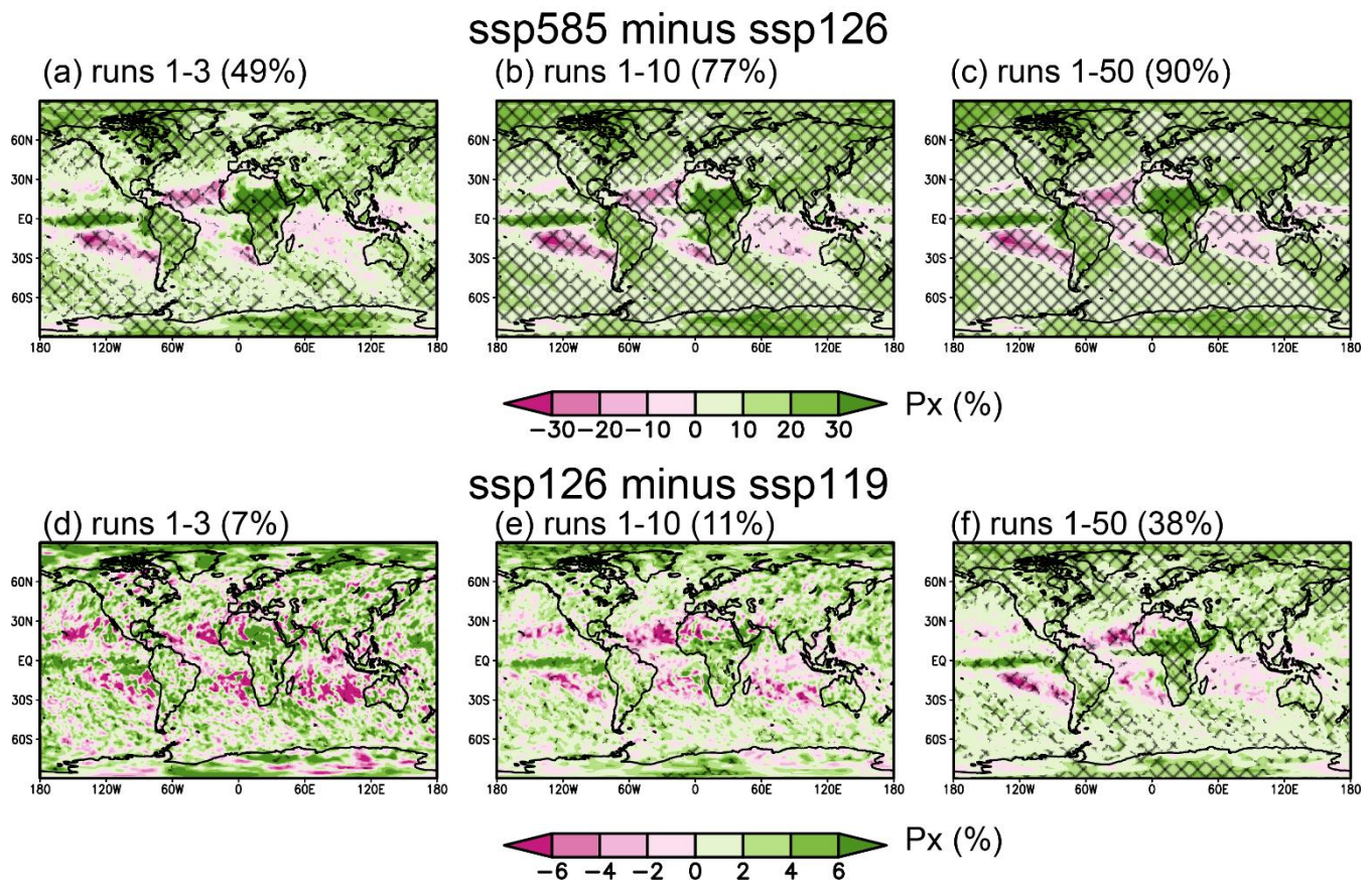
595 Figure 8: (Top) Differences in changes in Px (percent changes of 2050-2100 relative to 1850-1900) between ssp585 and ssp126 runs. Shading shows the ensemble mean of (a) runs 1-3, (b) runs 1-10 and (c) runs 1-50. Hatching denotes the regions where the differences are significant at 5% levels of the t test. Numbers in parentheses indicate the fraction of the areas with significant differences. (Bottom) The same as the top panels but for differences between ssp126 and ssp119.
