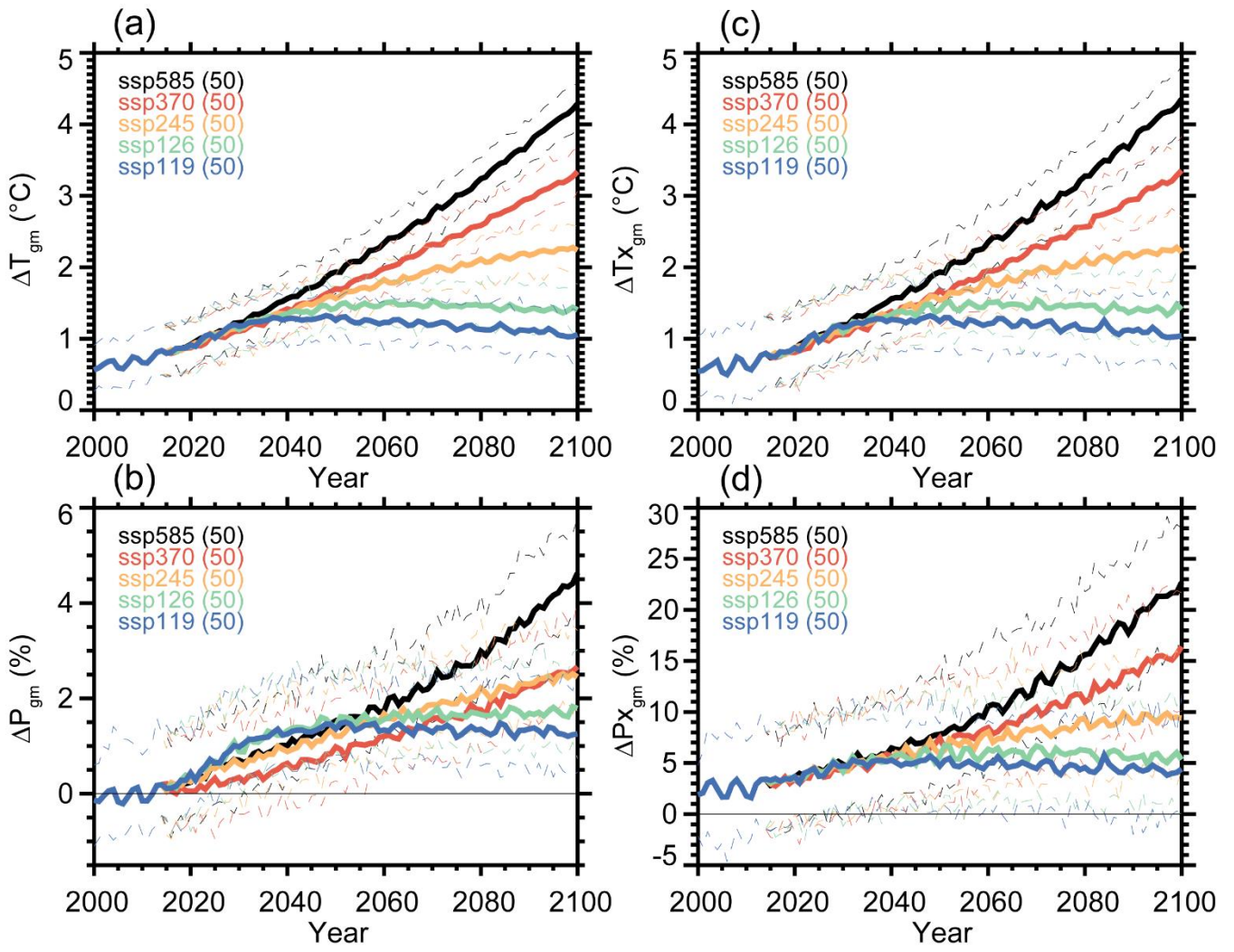
590 Figure 7: Future changes in global mean (a) T ( ^{\circ}C ), (b) P (%), (c) Tx ( ^{\circ}C ) and (d) Px (%) relative to the 1850-1900 averages. Solid lines are the ensemble averages of ssp585 (black), ssp370 (red), ssp245 (orange), ssp126 (green) and ssp119 (blue). Thin dashed lines denote the minimum and maximum values of the ensemble members. Numbers in parentheses indicate the ensemble sizes.
