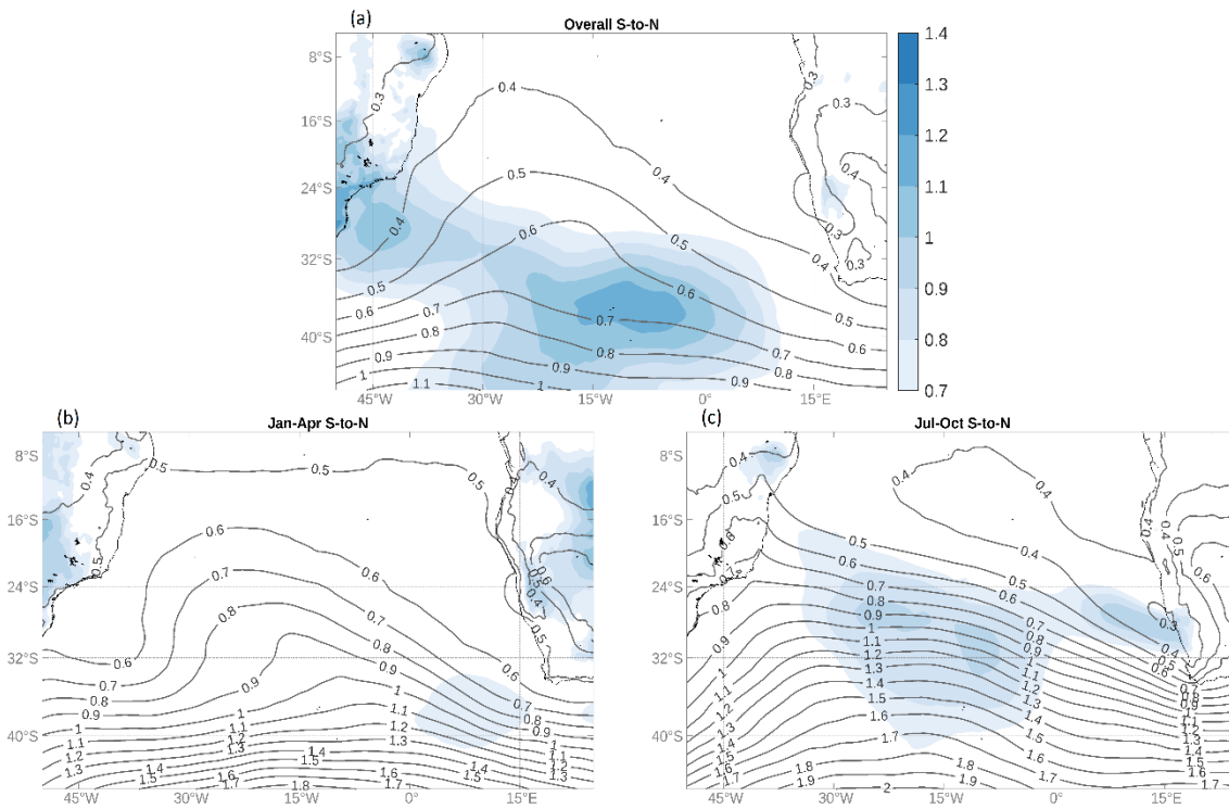
415 Figure 5: Spatial pattern of the variability (i.e., \sigma_{yr} ; contours; hPa) and signal-to-noise ratio (S/N) associated with the long-term trend (color shading) of the ERA5 SLP over 1979-2021. Panel (a) represents the values obtained for yearly mean SLP over the entire calendar year, whereas panels (b) and (c) correspond to the average over Jan-Apr and Jul-Oct, respectively.
