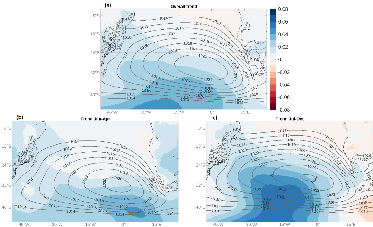
400 Figure 4: Long-term mean (contours; hPa) and trend (color shading; hPa/yr) of the ERA5 SLP for 1979-2021. Panel (a) represents the trend ( \alpha ) and mean-state obtained over the entire calendar months for yearly mean SLP, whereas (b-c) corresponds to the averages over Jan-Apr and Jul-Oct, respectively.
