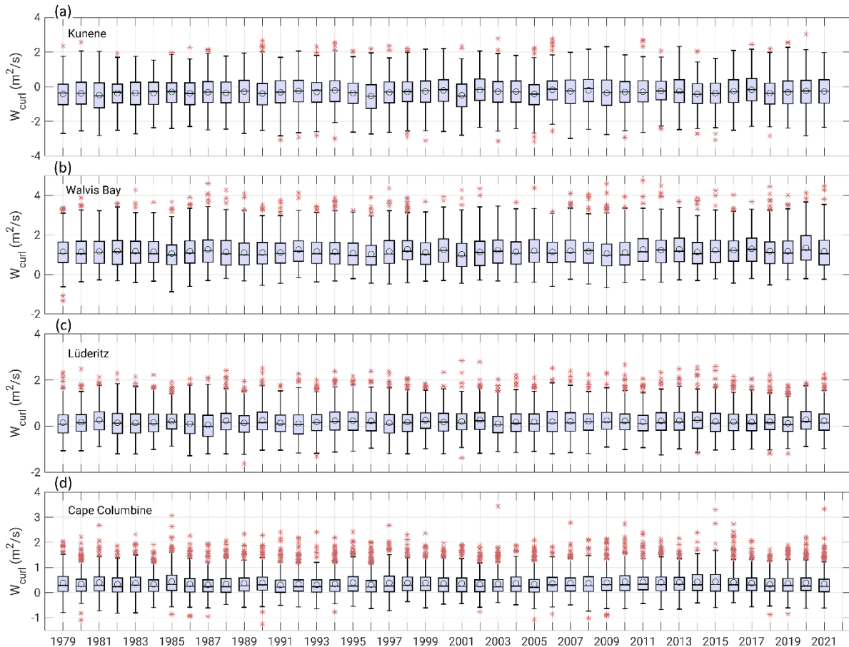
450 Figure 7: Boxplot representing the median and the interquartile range of W_{curl} in Kunene (a), Walvis Bay (b), Lüderitz (c), and Cape Columbine (d) upwelling cells derived from ERA5 data over 1979-2021. Each box represents the distribution of the daily W_{curl} in the corresponding year. The bands and circles inside the boxes represent the medians and mean, respectively. The red crosses indicate the extreme events defined as the values exceeding the confidence limits (i.e., outliers). 455 W_{curl} for the Kunene, Walvis Bay, Lüderitz, and Cape Columbine are the average over 17.5°S-17°S, 23.5°S-23°S, 27°S-26.5°S, and 33.25°S-32.75°S, respectively.
