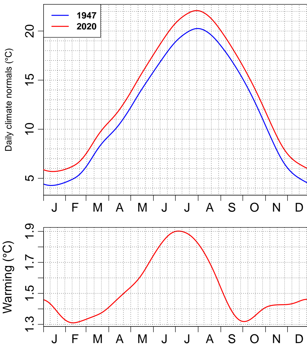
Figure 4. Changing climate normals Top: Daily climate normals for the daily mean temperature over France, estimated in 1947 and 2020, following the methodology of Rigal et al. (2018). Bottom: Difference between the 1947 and 2020 climate normals, i.e., 1947 to 2020 warming as function of the time of the year.
