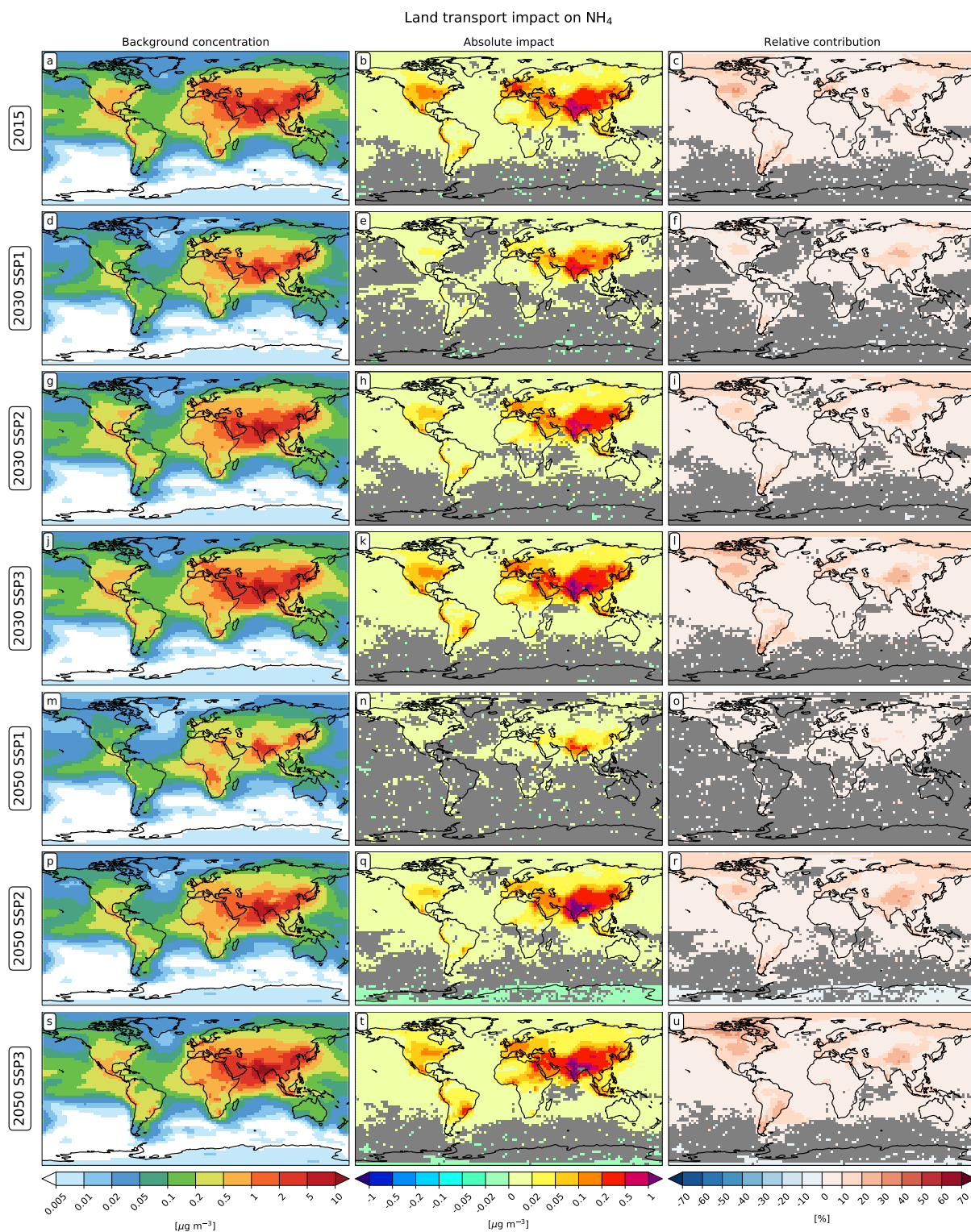
Figure S4: Land transport impact on surface-level \text{NH}_4 concentration. The left panels show the background concentration for reference. The middle and right panels show the land-transport-induced absolute impacts and the relative contributions, respectively. Grid points where the impacts are not significant to a 95% confidence level are masked out in gray.
