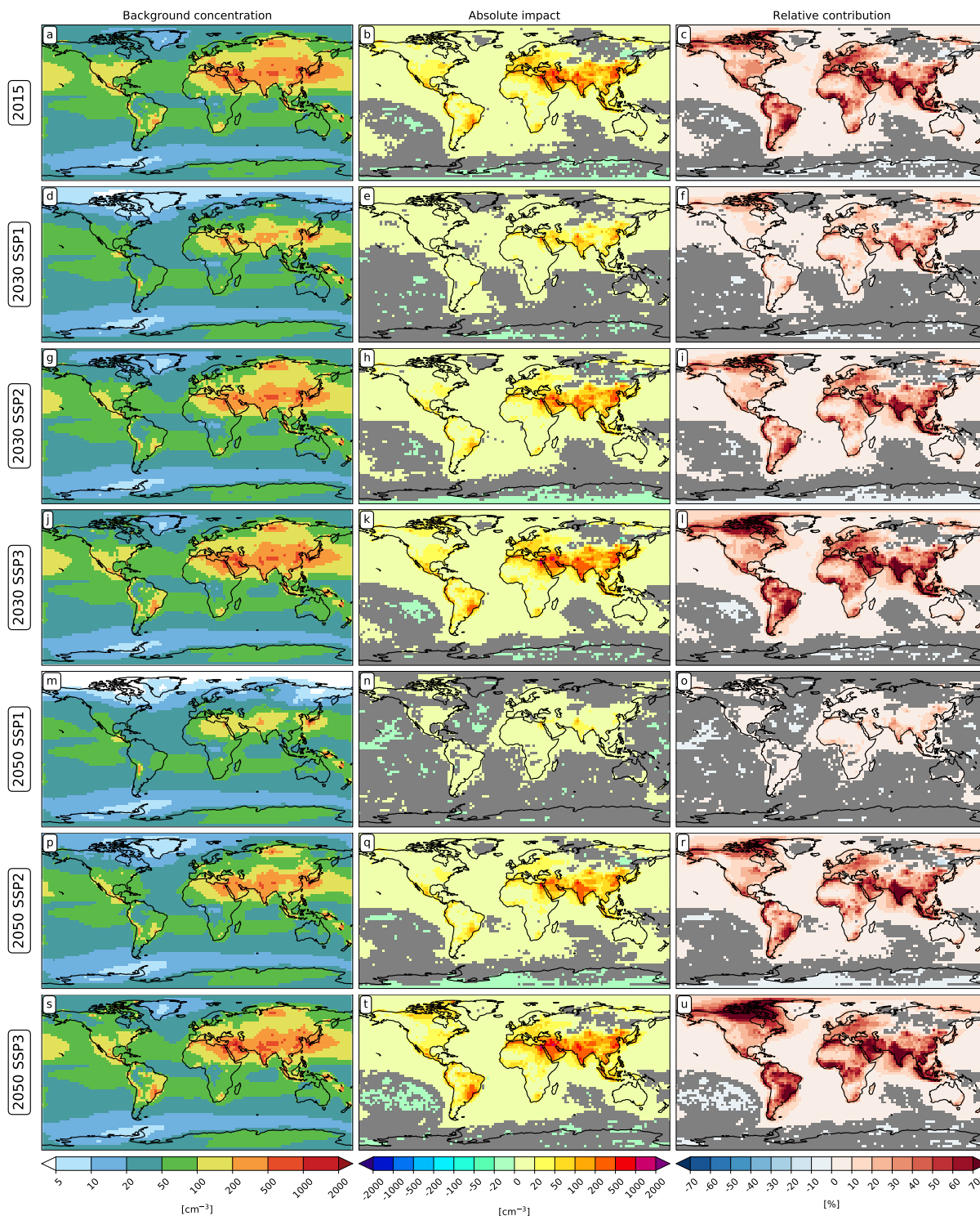
Land transport impact on particle number (Aitken mode)
