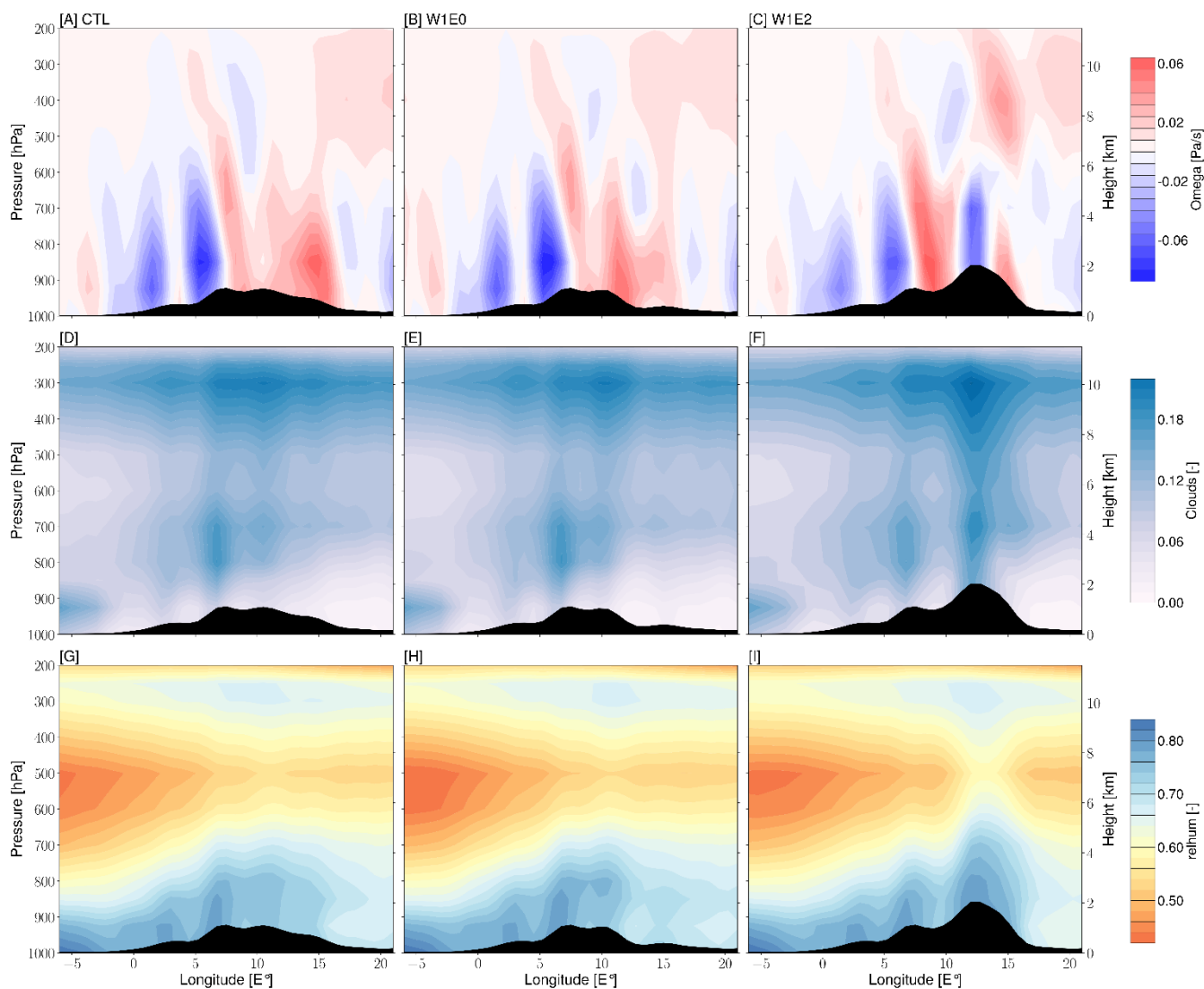
460 Figure 10: Seasonal (JJA) means of vertical wind velocity (omega) (A-C), cloud cover (D-F), and relative humidity (G-I) averaged between 45 - 48 °N across the Alps for the W1 (i.e., W1E0, W1E2) and CTL experiments. The black shadings represent the cross-section of topography for each scenario. The omega values represent the speed of air motion in the upward or downward direction. Since vertical pressure decreases with height, negative values indicate upward or ascent velocity and positive values indicate downward or subsidence velocity.
