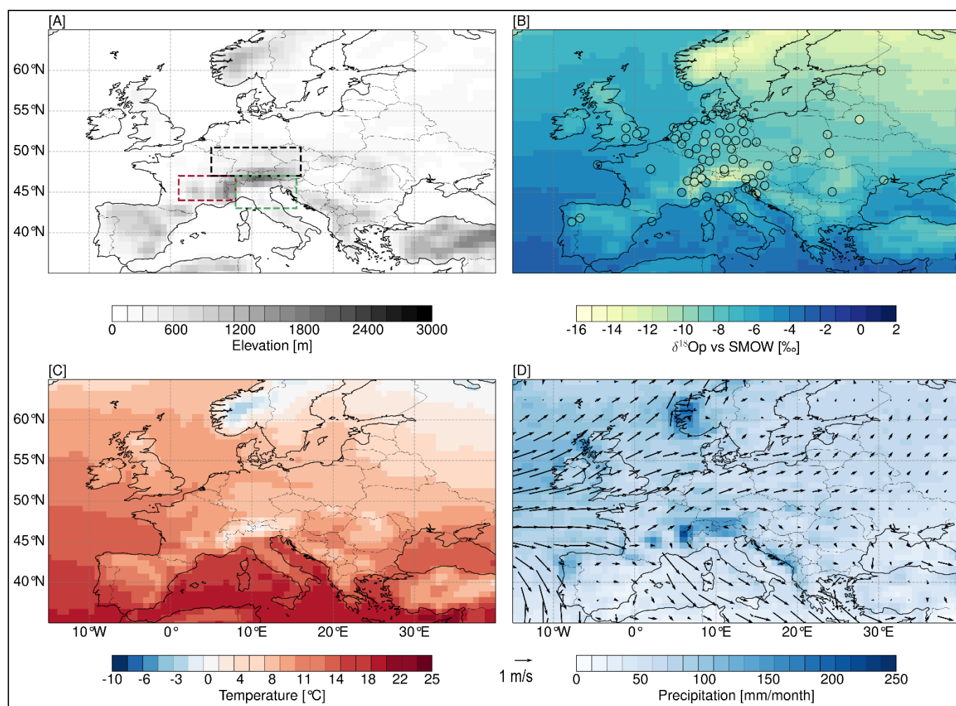
Figure 1: Present-day (PD) simulation topography (with geographical windows used for isotopic lapse rate calculations) (A), simulated (shading on map), and observed (circles) annual means of \delta^{18}\text{O}_p values. Colored circles represent observed \delta^{18}\text{O}_p values obtained from GNIP network stations (B), simulated near-surface temperature (C), and precipitation amount (colored shading) with near-surface wind patterns (arrows: length of arrows indicates wind speed, m/s) (D).
