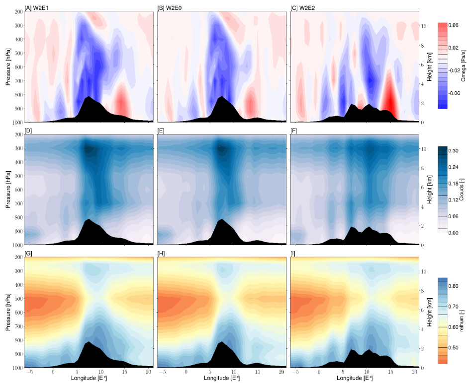
Figure 11: Seasonal (JJA) means of vertical wind velocity (omega) (A-C), cloud cover (D-F), and relative humidity (G-I) averaged between 45-48°N across the Alps for the W2 of scenario 1 (i.e., W2E1, W2E1), scenario 2 (i.e., W2E2) and CTL experiments. The black shadings represent the cross-section of topography for each scenario. The omega values represent the speed of air motion in the upward or downward direction. Since vertical pressure decreases with height, negative values indicate upward, or ascent velocity and positive values indicate downward or subsidence velocity.
