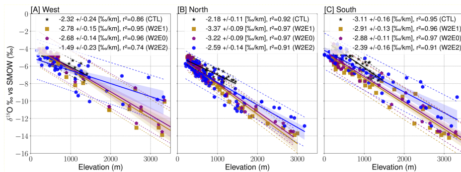
Figure 7: Summer isotopic lapse rates (ILR) estimates for the W2 topography scenarios (i.e., W2E0 (purple), W2E1 (gold), CTL (black), and W2E2 (blue) experiments) for the different transects around the Alps as shown in Fig. 6 E ((West: 44 - 47 °N, 1- 8 °E, south: 43-47 °N, 8-15 °E, and north: 47-50 °N, 5-16 °E). The ILRs are estimated as the \delta^{18}\text{O}_p -elevation gradients using linear regression. The lapse rate uncertainties are determined using the 95% confidence interval around the calculated OLS slope using t-distribution with n-2 degrees of freedom where the standard deviation of the slope is the point estimate, coefficient of determination ( r^2 ) is the measure for the fraction of the variability of the \delta^{18}\text{O}_p values that can be explained by the best-fitted OLS estimates and the 95% confidence and prediction interval around the regression fitted model to highlight the uncertainties around the individual topographic configuration if it was meant to be used to calculate the paleoelevation for a reconstructed \delta^{18}\text{O}_p values.
