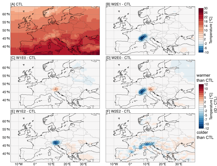
390 Figure 3: Seasonal (JJA) long-term mean of the near-surface temperature of the CTL experiment (A) and seasonal (JJA) mean difference of near-surface temperature for the different topography scenarios (i.e., W2E1-CTL (B), W1E0-CTL (C), W2E0-CTL (D), W1E2-CTL (E) and W2E2-CTL (F)). Red color ranges represent warmer temperatures, and blue color ranges represent colder temperatures than in the CTL experiment. Regions that experience changes that are statistically significant, as indicated by student t-test analysis with a 95% confidence level, are marked with black slash stippling.
