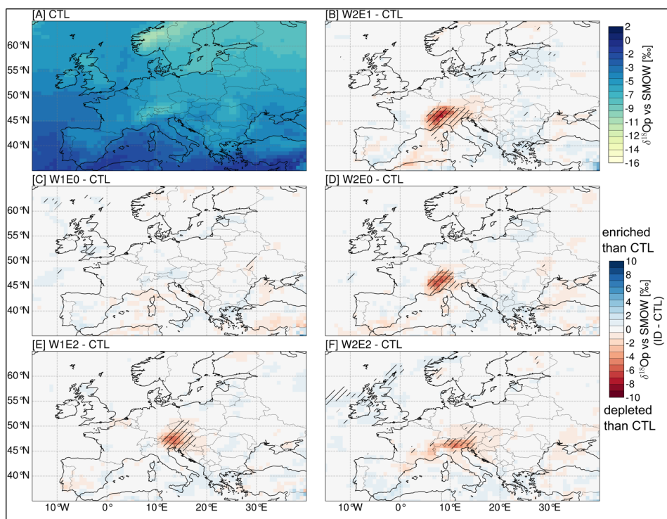
370 Figure 2: Seasonal (JJA) long-term mean of \delta^{18}\text{O} values of the CTL experiment (A) and seasonal (JJA) mean difference of \delta^{18}\text{O} values for the different topography scenarios (i.e., W2E1-CTL (B), W1E0-CTL (C), W2E0-CTL (D), W1E2-CTL (E) and W2E2-CTL (F)). Red color ranges represent heavy isotope depletion, and blue color ranges represent an enrichment in heavy isotopes relative to the CTL experiment. Regions that experience changes that are statistically significant, as indicated by student t-test analysis with a 95% confidence level, are marked with black slash stippling.
