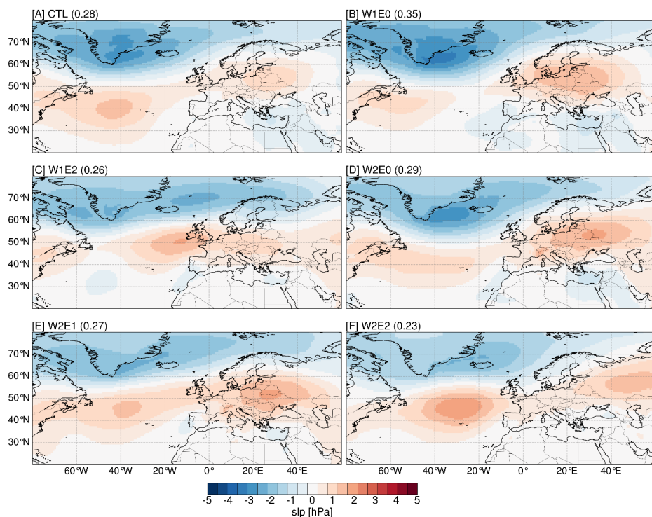
Figure 12: The spatial patterns and explained variance of the first Empirical Orthogonal Function (EOFs) extracted from the topography experiments. These resemble the leading mode of variability extracted from the ERA5 data (cf. Fig. S13 in the
