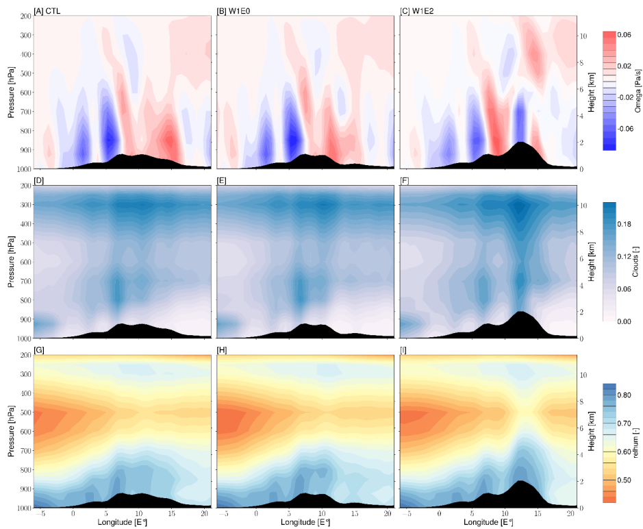
Figure 10: Seasonal (JJA) means of vertical wind velocity (omega) (A-C), cloud cover (D-F), and relative humidity (G-I) averaged between 45-48 °N across the Alps for the WI (i.e., W1E0, W1E2) and CTL experiments. The black shadings represent the cross-section of topography for each scenario. The omega values represent the speed of air motion in the upward or downward direction. Since vertical pressure decreases with height, negative values indicate upward , or ascent velocity and positive values indicate downward or subsidence velocity.
