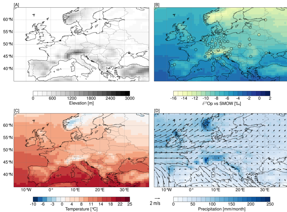
335 Figure 1: Present-day (PD) simulation topography (A), simulated (shading on map), and observed (circles) annual means of \delta^{18}\text{O}_p values. Colored circles represent observed \delta^{18}\text{O}_p values obtained from GNIP network stations (B), simulated near-surface temperature (C), and precipitation amount (colored shading) with near-surface wind patterns (arrows: length of arrows indicates wind speed, m/s) (D).
