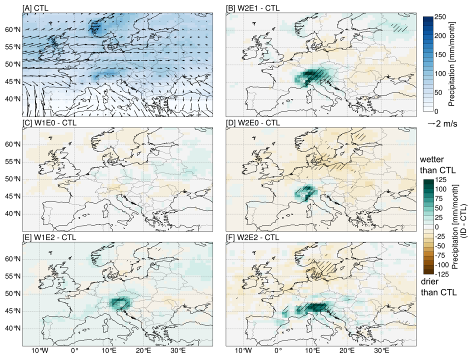
410 Figure 4: Seasonal (JJA) long-term mean of precipitation amount (shading) with near-surface wind patterns (arrows) of the CTL 415 experiment (A) and mean difference of precipitation amount for the different topography scenarios (i.e., W2E1-CTL (B), W1E0- CTL (C), W2E0-CTL (D), W1E2-CTL (E) and W2E2-CTL (F)). Green color ranges represent wetter, and brown color ranges represent drier conditions than in the CTL experiment. Regions that experience changes that are statistically significant, as indicated by student t-test analysis with a 95% confidence level, are marked with black slash stippling.
