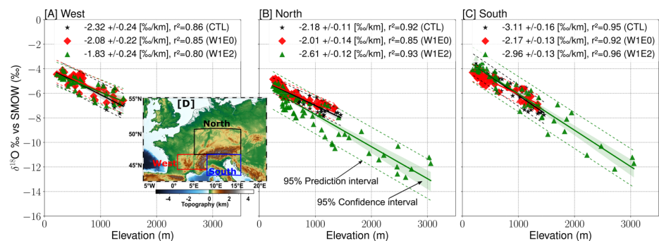
465 Figure 6: Summer isotopic lapse rates (ILRs) estimates for the W1 topography scenarios (i.e., W1E0 (red), W1E2 (green)), and CTL (black) experiments for the different transects around the Alps as shown in E (West: 44.47 °N, 1.8 °E, south: 43.47 °N, 8.15 °E, and north: 47.50 °N, 5.16 °E). The ILRs are estimated as the \delta^{18}O_p -elevation gradients using linear regression. The lapse rate uncertainties are determined using the 95% confidence interval around the calculated OLS slope using t-distribution with n-2 degrees of freedom where the standard deviation of the slope is the point estimate, coefficient of determination ( r^2 ) is the measure for the fraction of the variability of the \delta^{18}O_p values that can be explained by the best-fitted OLS estimates and the 95% confidence
