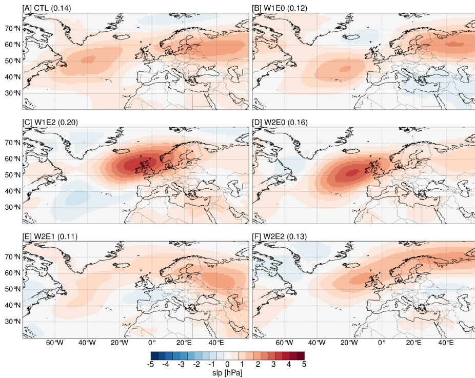
610 Figure 13: The spatial patterns and explained variance of the Empirical Orthogonal Functions (EOFs) that resemble the second mode of variability extracted from the ERA5 data (cf. Fig. S13 in the supplemental material). The patterns are calculated from summer mean sea level pressure (slp) anomalies and represent the covariance matrix of the Principal Component time series and the EOFs.
