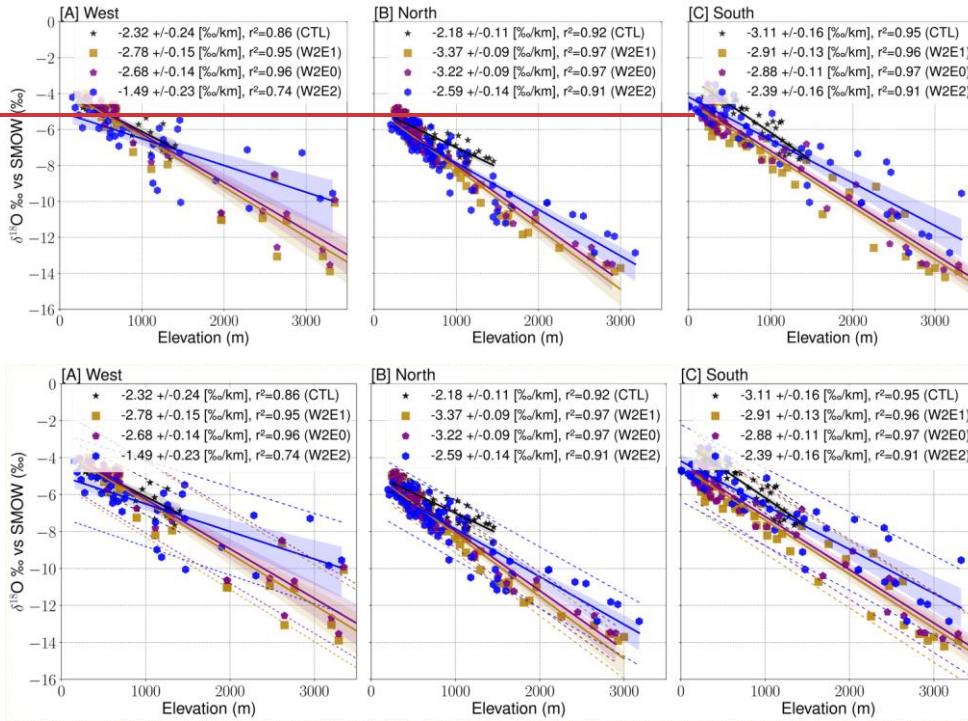
Figure 7: Summer isotopic lapse rates (ILR) estimates for the W2 topography scenarios (i.e., W2E0 (purple), W2E1 (gold), CTL (black), and W2E2 (blue) experiments for the different transects around the Alps as shown in Fig. 6 E ((West: 44 - 47 °N, 1- 8 °E, south: 43 - 47 °N, 8 -15 °E, and north: 47 - 50 °N, 5-16 °E). The ILRs are estimated as the \delta^{18}\text{O}_s -elevation gradients using linear regression. The lapse rate uncertainties are determined using the 95% confidence interval around the calculated OLS slope using t-distribution with n-2 degrees of freedom where the standard deviation of the slope is the point estimate, coefficient of determination ( r^2 ) is the measure for the fraction of the variability of the \delta^{18}\text{O}_s values that can be explained by the best-fitted OLS estimates and the 95% confidence and prediction interval around the regression fitted model to highlight the uncertainties around the individual topographic configuration if it was meant to be used to calculate the paleoelevation for a reconstructed \delta^{18}\text{O}_s values. r^2 -values represent the associated correlation coefficients. The lapse rate uncertainties are estimated assuming a 95% confidence interval.
