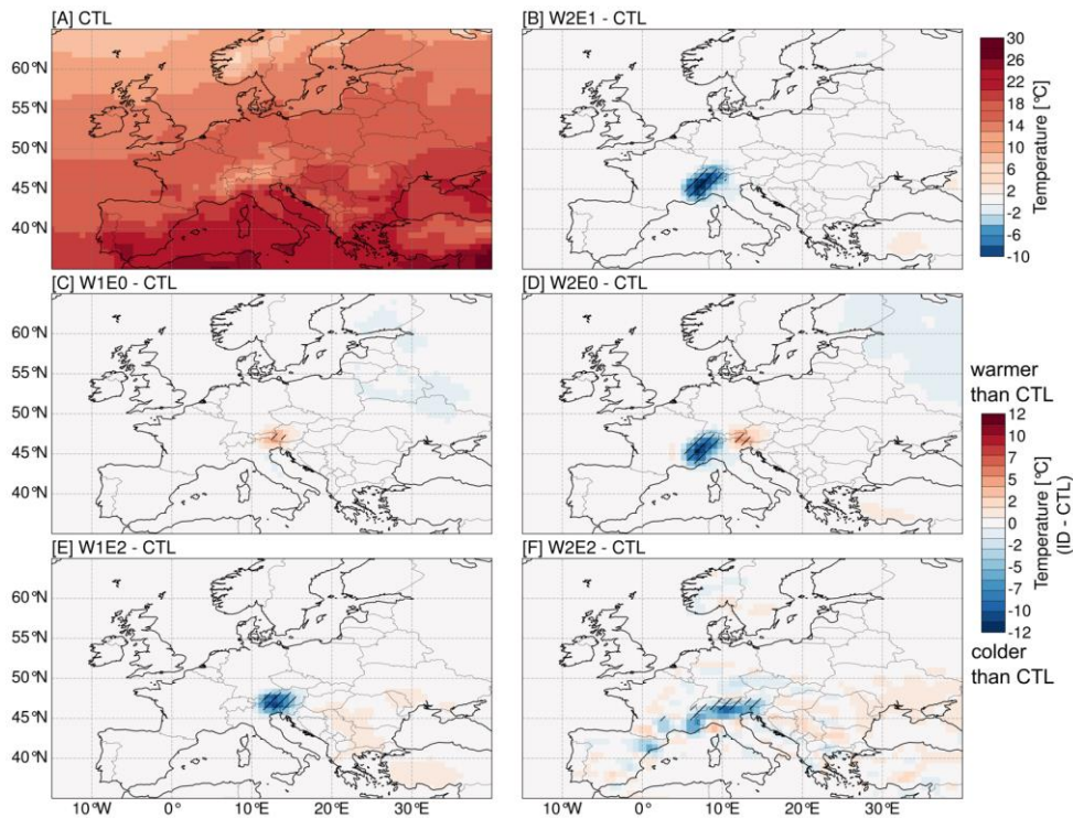
370 Figure 3: Seasonal (JJA) long-term mean of the near-surface temperature of the CTL experiment (A) and seasonal (JJA) mean difference of near-surface temperature for the different topography scenarios (i.e., W2E1-CTL (B), W1E0-CTL (C), W2E0-CTL (D), W1E2-CTL (E) and W2E2-CTL (F)). Red color ranges represent warmer, and blue color ranges represent colder temperatures than in the CTL experiment. Regions that experience changes that are statistically significant, as indicated by student t-test analysis with a 95% confidence level, are marked with black slash stippling.
