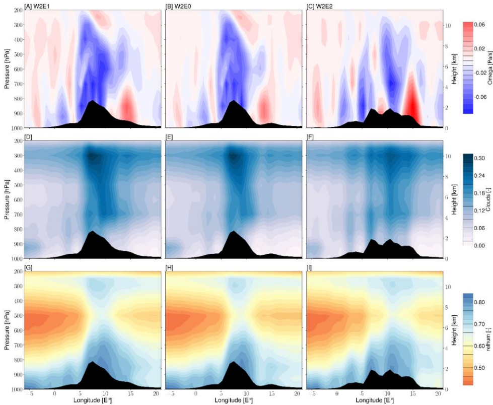
520 Figure 11: Seasonal (JJA) means of vertical wind velocity ( \omega ) (A-C), cloud cover (D-F), and relative humidity (G-I) averaged between 45 - 48 °N across the Alps for the W2 of scenario 1 (i.e., W2E1, W2E1), scenario 2 (i.e., W2E2) and CTL experiments. The black shadings represent the cross-section of topography for each scenario. The \omega values represent the speed of air motion in the upward or downward direction. Since vertical pressure decreases with height, negative values indicate upward, or ascent velocity and positive values indicate downward or subsidence velocity.
