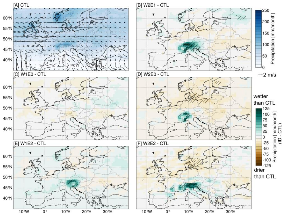
390 Figure 4: Seasonal (JJA) long-term mean of precipitation amount (shading) with near-surface wind patterns (arrows) of the CTL experiment (A) and mean difference of precipitation amount for the different topography scenarios (i.e., W2E1-CTL (B), W1E0-CTL (C), W2E0-CTL (D), W1E2-CTL (E) and W2E2-CTL (F)). Green color ranges represent wetter, and brown color ranges represent drier conditions than in the CTL experiment. Regions that experience changes that are statistically significant, as indicated by student t-test analysis with a 95% confidence level, are marked with black slash stippling.
