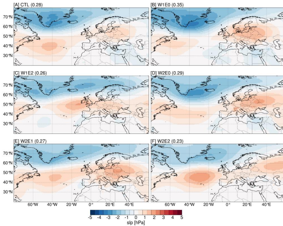
Figure 12: The spatial patterns and explained variance of the first Empirical Orthogonal Function (EOFs) extracted from the topography experiments. These resemble the leading mode of variability extracted from the ERA5 data (cf. Fig. S13 in the
