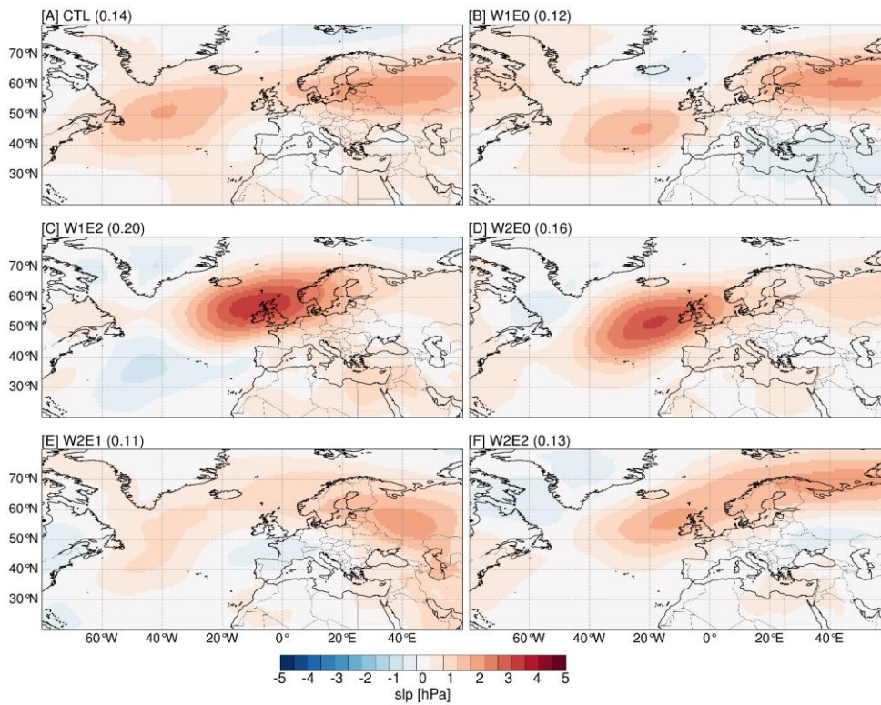
Figure 13: The spatial patterns and explained variance of the Empirical Orthogonal Functions (EOFs) that resemble the second mode of variability extracted from the ERA5 data (cf. Fig. S13 in the supplemental material). The patterns are calculated from summer mean sea level pressure (slp) anomalies and represent the covariance matrix of the Principal Component time series and the EOFs.
