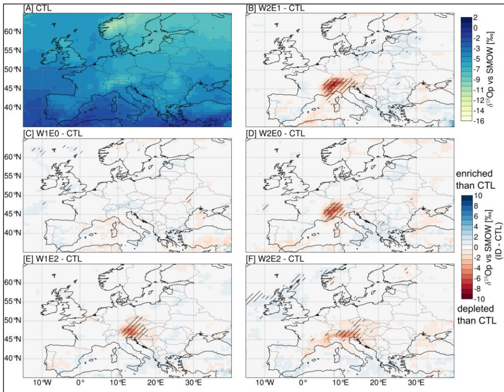
350 Figure 2: Seasonal (JJA) long-term mean of \delta^{18}\text{O} values of the CTL experiment (A) and seasonal (JJA) mean difference of \delta^{18}\text{O} values for the different topographic scenarios (i.e., W2E1-CTL (B), W1E0-CTL (C), W2E0-CTL (D), W1E2-CTL (E) and W2E2-CTL (F)). Red color ranges represent heavy isotope depletion, and blue color ranges represent an enrichment in heavy isotopes relative to the CTL experiment. Regions that experience changes that are statistically significant, as indicated by student t-test analysis with a 95% confidence level, are marked with black slash stippling.
