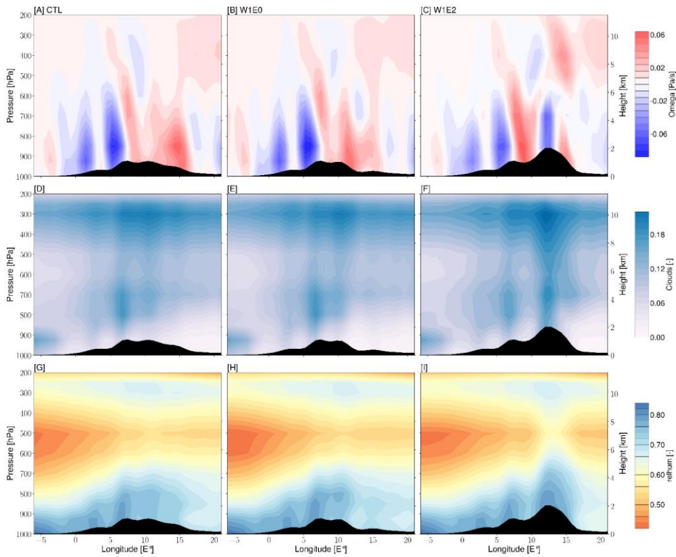
515 Figure 10: Seasonal (JJA) means of vertical wind velocity ( \omega ) (A-C), cloud cover (D-F), and relative humidity (G-I) averaged between 45 - 48 °N across the Alps for the W1 (i.e., W1E0, W1E2) and CTL experiments. The black shadings represent the cross-section of topography for each scenario. The \omega values represent the speed of air motion in the upward or downward direction. Since vertical pressure decreases with height, negative values indicate upward or ascent velocity and positive values indicate downward or subsidence velocity.
