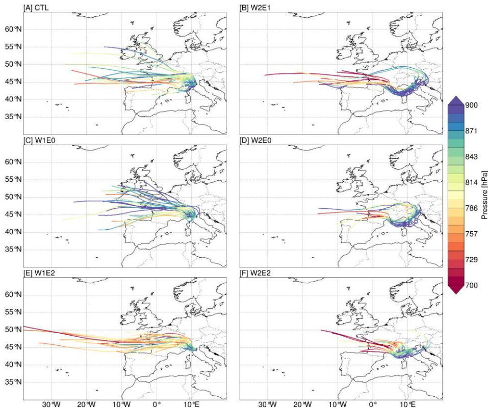
Figure 9: 5 days summer back-trajectories with the receptor location set to the 850 hPa level above Bologna (44.49 °N, 11.38 °E). The colored lines represent the vertical pressure level of the trajectories. The trajectories were estimated with the 6h wind fields (i.e., u, v, and omega) from the topographic experiments using the LAGRANTO tool.
