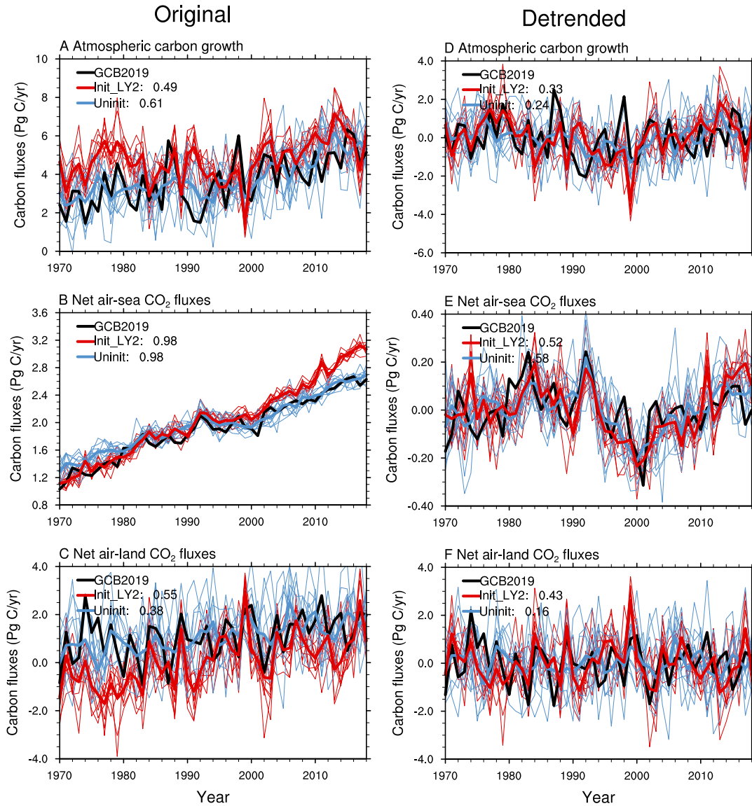
Figure 6. Left panels: Time series at a lead time of 2 years for atmospheric carbon growth rate, i.e., G_{ATM} (A), net air-sea \text{CO}_2 fluxes, i.e., S_{OCEAN} (B) and net air-land \text{CO}_2 fluxes, i.e., ELUC+S_{LAND} (C) from the initialized simulations together with values from the uninitialized simulations and estimates from the 2019 Global Carbon Budget (GCB 2019, (Friedlingstein et al., 2019)). Right hand panels are the same as the left hand side panels, but show the linearly detrended time series. The time series shown are based on annual mean data for the time period of 1970-2018. Positive values in panels B, C, E, and F imply \text{CO}_2 fluxes into the ocean or land. The numbers in the legend show the correlation coefficients between the simulations and GCB2019, and the ensemble mean data is used for the calculation.
