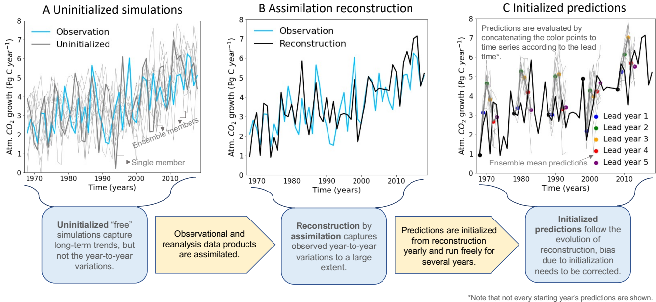
Figure 1. Illustration of the decadal prediction system based on the MPI Earth system model. The illustrated time series of the atmospheric CO 2 growth rate shows annual means from model simulations plotted together with observations from the Global Carbon Project (GCP). We conduct three sets of simulations, from left to right in sequential order: i) uninitialized "free" simulations which are the same as the freely-evolving Coupled Model Intercomparison Project (CMIP) historical type simulations; ii) an assimilation simulation to reconstruct the evolution of the climate and carbon cycle towards the real world by nudging the model towards observation and reanalysis data during its integration; iii) initialized predictions are started from reconstruction states produced by the assimilation simulation and integrated freely (i.e., no nudging towards observations) for 5 years. The time series in the left panel A shows that the uninitialized simulations capture the long-term trend well, but the year-to-year variations are out of phase with the observations. The time series in the middle panel B shows that the assimilation simulation forces the variations in the uninitialized freely run simulation towards the real world, and results in a reconstruction that is closer to the observations. The right panel C shows the reconstruction together with the 5-year long initialized predictions (i.e., hindcasts). To make the illustration more clear, only predictions with starting years at 10-year intervals are shown.
