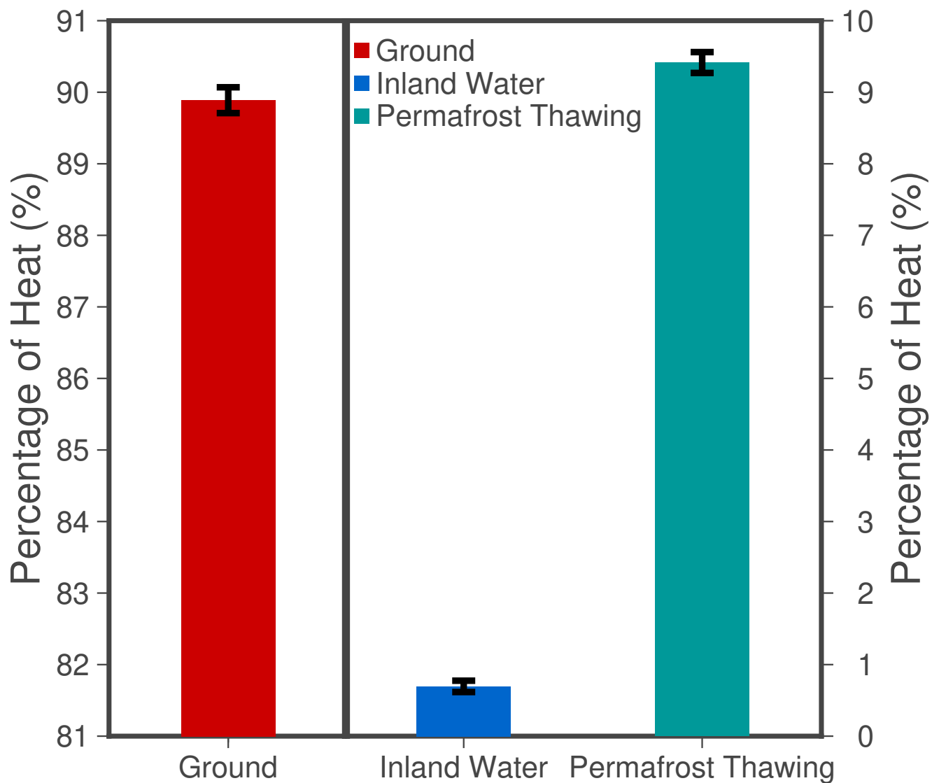
Figure 4. Percentage (%) of the continental heat storage within each analysed land component for the period 1960-2020: ground (red), inland water bodies (blue), and permafrost thawing (green). Left axis corresponds to ground results, the right axis corresponds to results for permafrost soils and inland water bodies.
