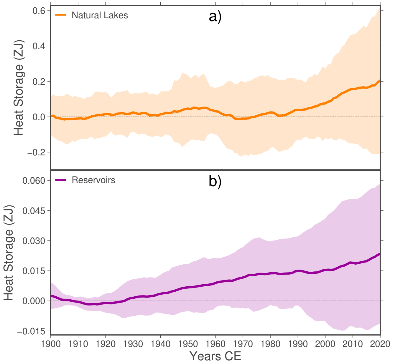
Figure 3. Heat storage by natural lakes (a), reservoirs (b). Shown are 6-year moving averages relative to the 1900–1929 reference period. Note the different y-axis scales. Colour shades represent uncertainty range shown as the standard deviation of the used simulations (16 for lake and reservoir heat storage).
