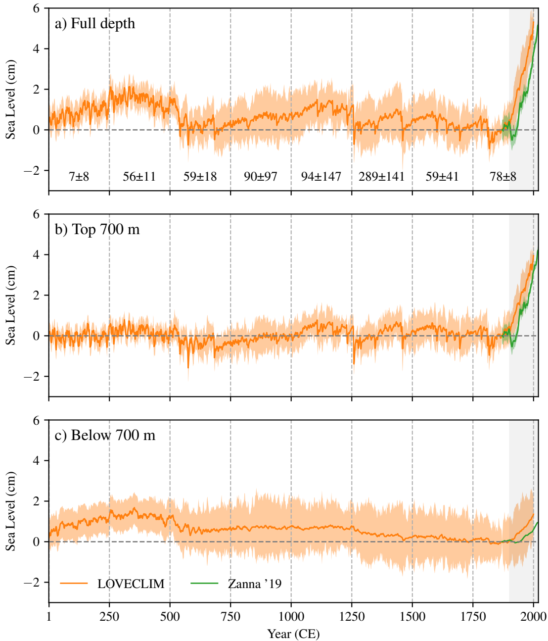
815 Figure 1: Global-mean thermosteric sea level from LOVECLIM climate model simulations (orange; 1-2000 CE) and Zanna et al. (2019) reconstruction (green; 1870 - 2018) for a) full depth (b) top 700 m and c) below 700 m. All curves are referenced to 1870 CE (when the reconstruction begins), and the shading indicates the 1- \sigma confidence level of the ensemble-mean curve. The percentage contribution of change in the top 700 meters thermosteric level to that of the full depth, estimated over chunks of 250-year periods (vertical dashed lines), is shown in panel a. The estimated 1900 – 2000 CE (period shown by grey shading) contribution of the upper 700 m for Zanna et al. (LOVECLIM) is 86% (74±8%).
