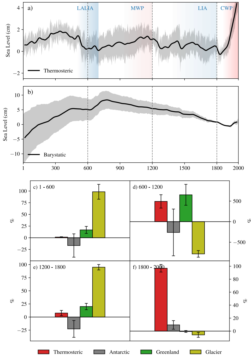
855 Figure 5: a) 31-year smoothed global-mean thermosteric (a) and barystatic (i.e. the sum of Antarctic, Greenland and glacier 860 contribution); b) sea level with their 1-sigma uncertainty level from EXP-I. We defined four time periods in the CE (1 – 600, 600 – 1200, 1200 – 1800 and 1800 – 2000; shown by dashed vertical lines in a, b) based on centennial-scale shifts seen in the global-mean thermosteric sea level. Those periods also mark the major sub-millennial climate epochs reported in the CE (The Late Antique Little Ice Age: LALIA (~ 600-700), The medieval warm period: MWP (~ 900 – 1300), The little ice age: LIA (~ 1300 – 1800) and the current warming period: CWP (post-1800). The respective contribution of thermosteric, ice-sheet and glacier mass-balance changes to model GMSL is estimated for these four periods and shown in panels c (1 – 600), d (600 – 1200), e (1200 – 1800) and f (1800 – 2000). Percentage contribution is calculated by a linear regression method, and the error bar represents the 1- \sigma standard deviation of the contribution across the large ensemble.
