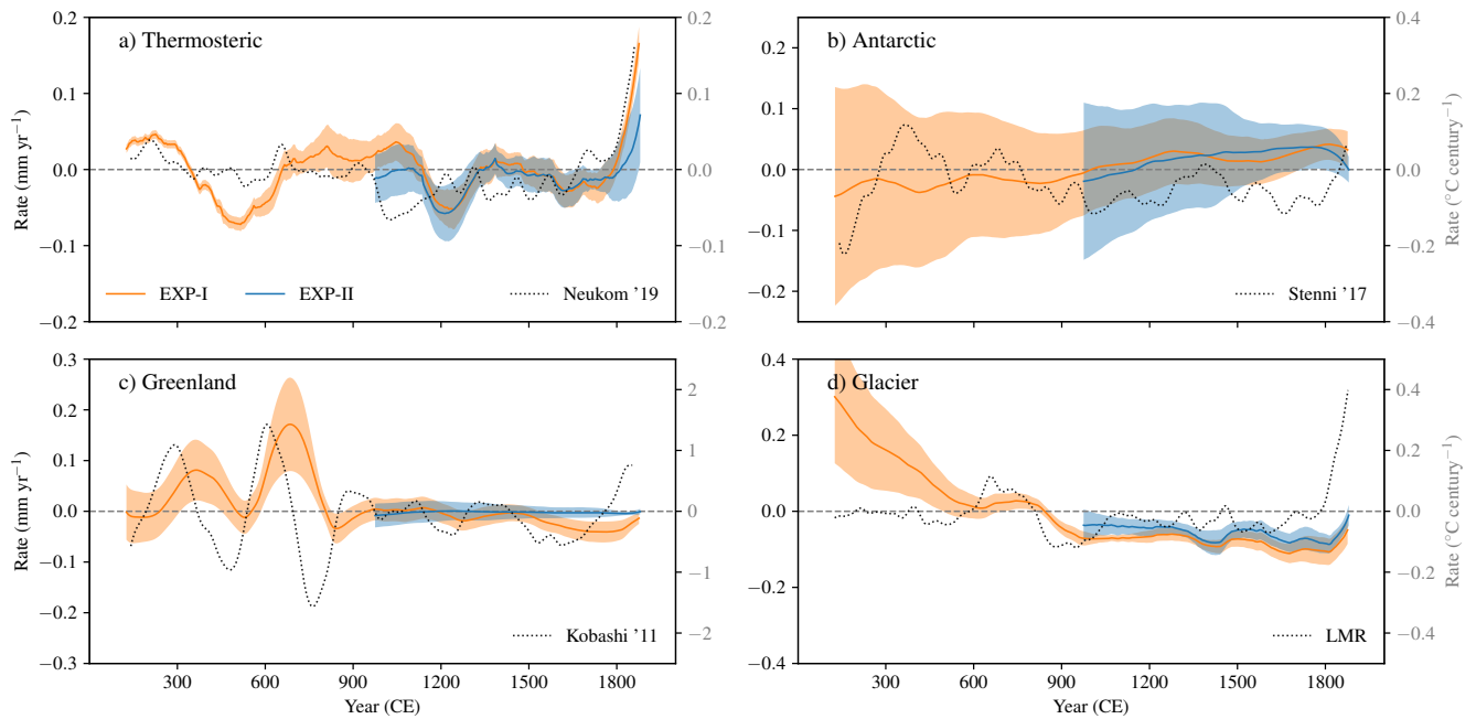
840 Figure 3: 250-year moving rate of sea level for each of the components shown in Figure 2. a) thermosteric b) Antarctic c) Greenland and d) Glaciers mass balance. 250-year rate of global (a) and regional surface temperature (shown in figure 2) is also shown (dotted grey lines). Shading around sea-level rates indicates 1- \sigma confidence level of the ensemble mean rate.
