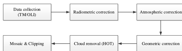
Figure 2. Preprocessing of Landsat Thematic Mapper (TM)/Operational Land Imager (OLI) scenes.
