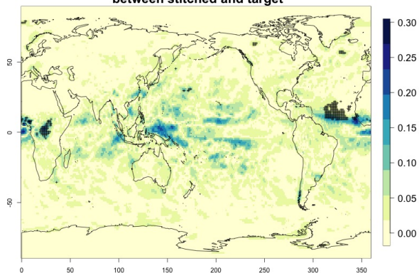
CAMS, SSP245 r1, pr: abs. differences in trends (mm/day/decade) between stitched and target
