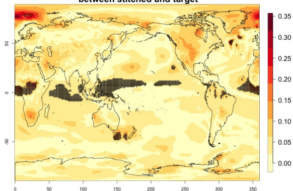
CAMS, SSP245 r1, TAS: abs. differences in trends (C/decade) between stitched and target
