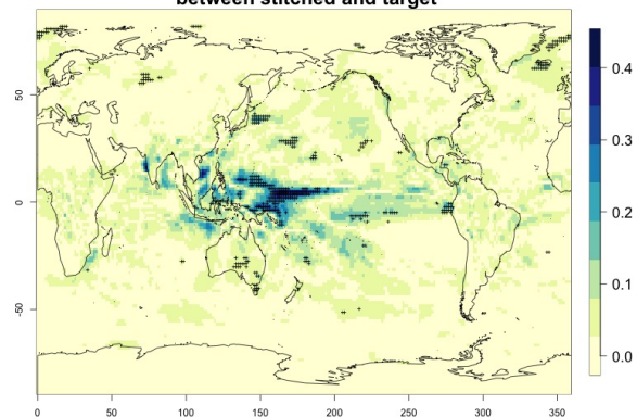
MIROC6, SSP370 r3, PR: abs. differences in trends (mm/day/decade) between stitched and target
