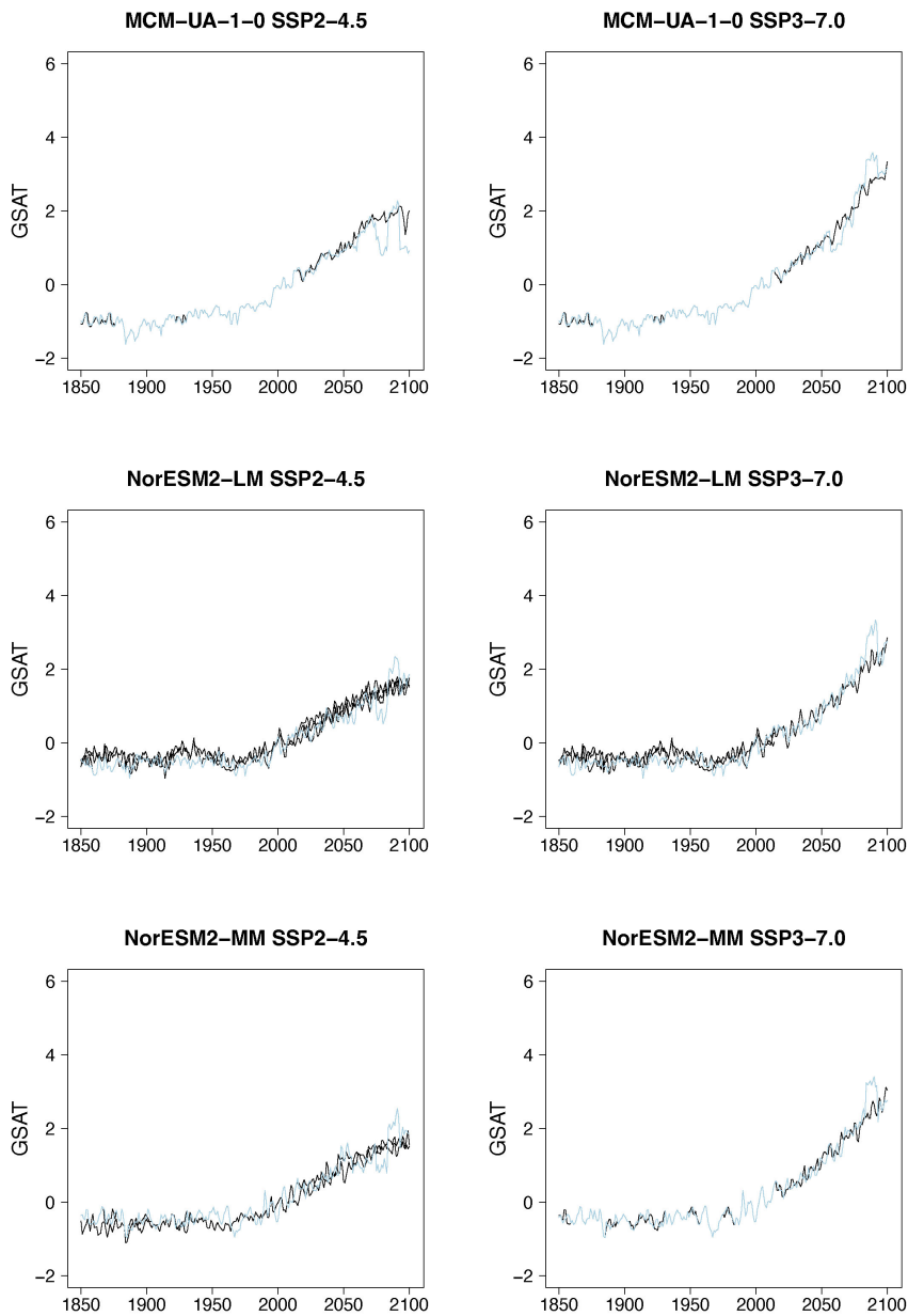
Figure B4. Examples of target (black lines) and stitched (colored) GSSAT time series for ESMs in the PANGEO archive that ran at least one trajectory along the Tier 1 experiments of ScenarioMIP (SSP1-2.6; SSP2-4.5; SSP3-7.0; SSP5-8.5). We use the two bracketing scenarios and emulate trajectories that follow the two intermediate scenarios.
