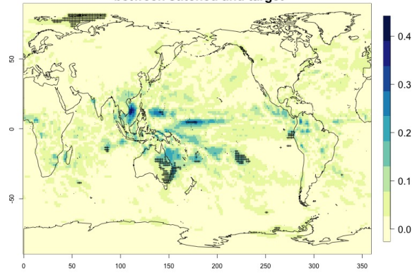
MIROC6, SSP370 r2, PR: abs. differences in trends (mm/day/decade) between stitched and target
