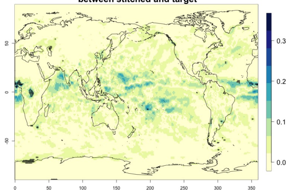
CAMS, SSP370 r1, PR: abs. differences in trends (mm/day/decade) between stitched and target
