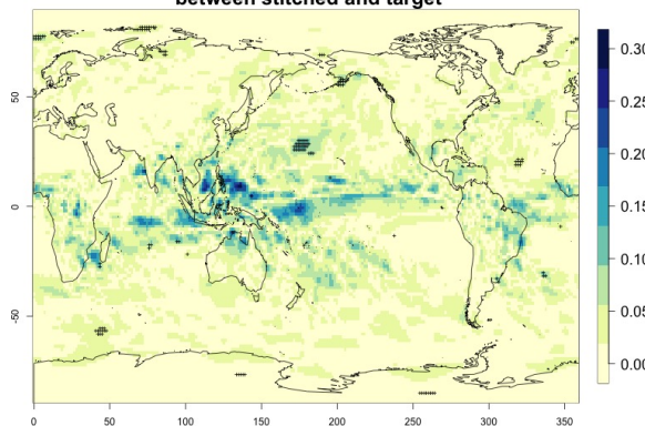
MIROC6, SSP245 r3, PR: abs. differences in trends (mm/day/decade) between stitched and target
