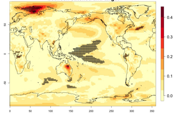
MIROC6, SSP370 r2, TAS: abs. differences in trends (C/decade) between stitched and target
