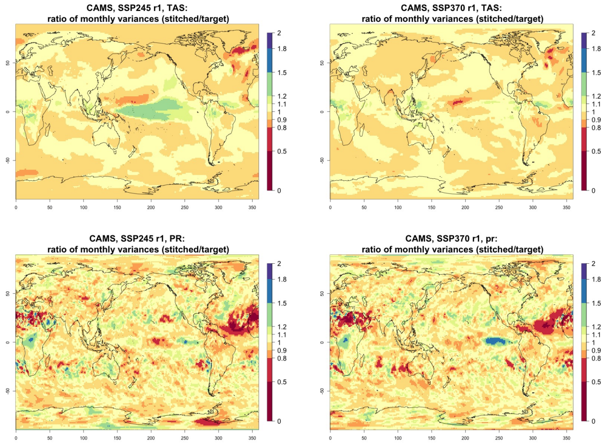
Figure 4. Ratio in monthly variability (standard deviation of residuals from trends) of future temperature (TAS) and precipitation (PR) between stitched (at the numerator) and target (at the denominator) realizations. The value of the ratio is expressed by the color scale which highlights the transition at 0.8 and 1.2. Emulation of CAMS-CM1-0 monthly time series for 2015-2100 under SSP2-4.5 and SSP3-7.0.
