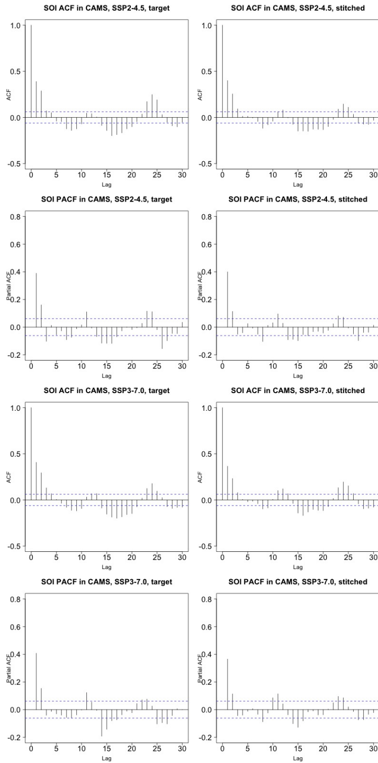
Figure 6. Auto-correlation (ACFs) and Partial auto-correlation functions (PACFs) for real and stitched SOI time series. Top two rows: SSP2-4.5 ACF for target and stitched series and respective PACFs. Bottom two rows: SSP3-7.0 ACF for target and stitched series and respective PACFs. (Our software – R function acf(..., type="partial") – does not define the PACF at lag zero.)
