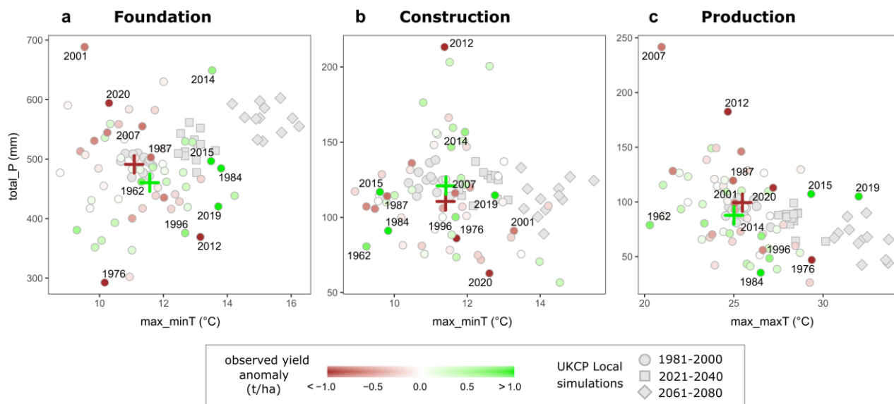
740 Figure 4: Association between observed wheat yields and climate during the three wheat-growing phases. Anomalies of observed 745 UK wheat yields are shown for total area-averaged precipitation ( total_P ) and the maximum of area-averaged minimum/maximum daily temperature within each phase (i.e. the metrics total_P , max_minT , and max_maxT , chosen for their associations with crop yields; Table 2), alongside UKCP projections. Columns: Foundation phase (01 st October to 09 th April); Construction phase (10 th April to 10 th June); Production phase (11 th June to 26 th July). Yield time series are shown for the national scale here (longer than regional time series, see Figure 1a vs 1b) and are the same in the three panels. Small green circles indicate positive yield anomalies for individual years; small brown circles indicate negative yield anomalies for individual years. Large green crosses indicate the mean for all the years with positive wheat yield anomalies; large brown crosses indicate the mean for all the years with negative wheat yield anomalies. Grey diamonds indicate UKCP Local projections of temperature and precipitation for the historical (circle: 1981-2000) and future (square: 2021-2040; diamond: 2061-2080) periods, where each symbol indicates one of the 12 ensemble members. Specific years mentioned in the main text are labelled.
