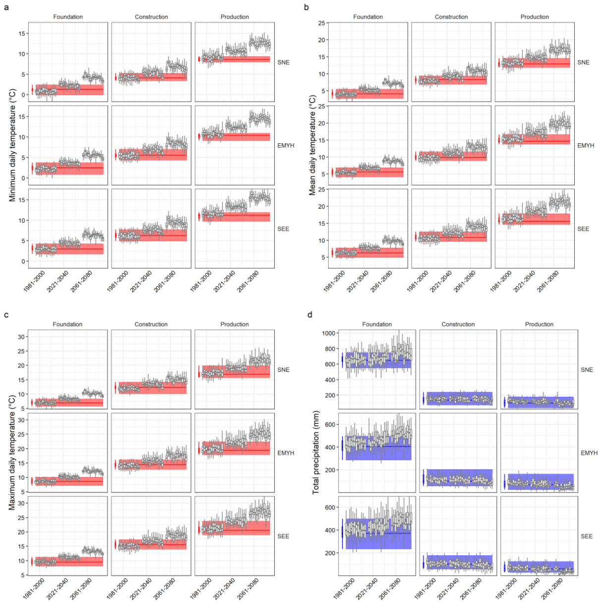
725 Figure 3: Bias-correction of each UKCP 2.2km ensemble member, for (a-c) the minimum, mean and maximum daily temperature ( mean_minT , mean_meanT and mean_maxT ), respectively; and (d) total precipitation ( total_P ), within each phase, for each of the three regions (SNE, EMYH, SEE). Red (blue) boxplots and rectangles indicate the range of observed temperature (precipitation) over the first period (1981-2000), based on the HadUK dataset. Grey boxplots indicate projections (one for each of 12 UKCP Local ensembles) for three periods (historical – 1981-2000; future – 2021-2040; 2061-2080) using RCP8.5. Boxplot hinges represent 25th and 75th percentiles, and horizontal bar indicates the median. Whiskers extend to the largest value no further than 1.5 times the interquartile range (distance between 25th-75th percentiles) from the hinge. 730
