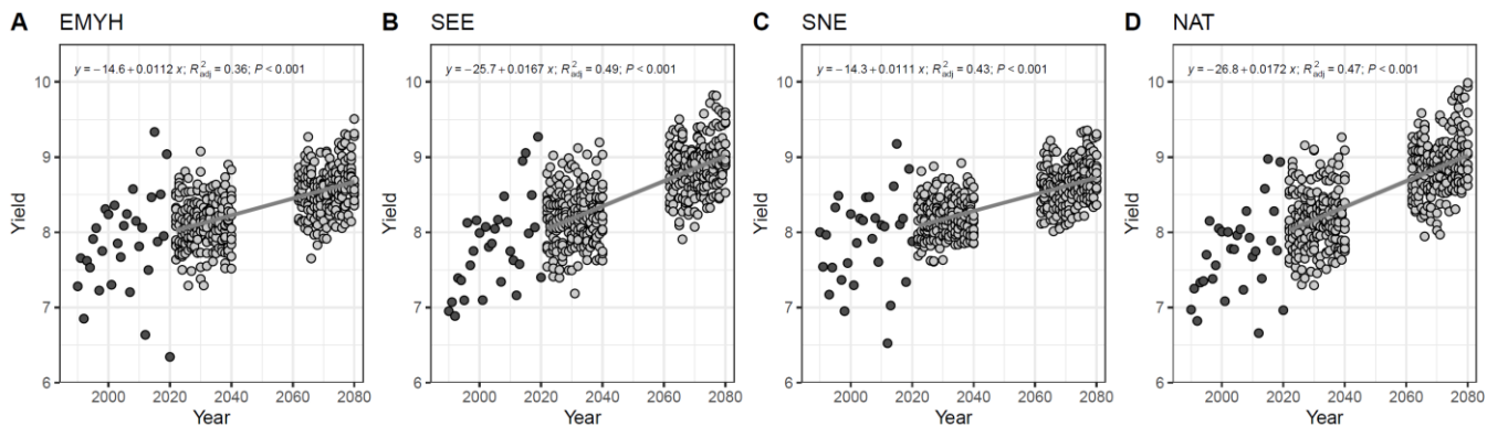
Figure 6: Temporal trends in wheat yields (tonnes/hectare): observations and future projections. The observations (black circles, 1990-2020) are the same as in Figure 1. The projections (grey circles; 12 members per year) are obtained by forcing a multiple linear regression model (Equation 1; Table 4) obtained for each region with the UKCP Local projections of the same climate variables in each growth stage (see Methods section 2.5). Grey lines indicate the linear regressions between the ensemble of projected values and time (the regression equation, adjusted R2, and p-value are indicated on each panel).
