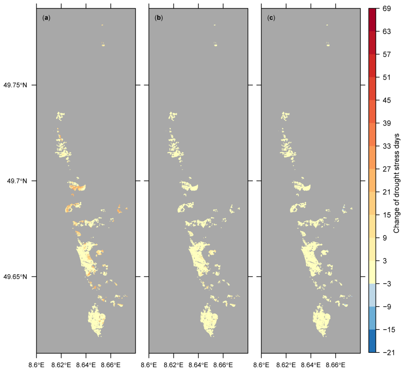
Figure 12: Projected change of the occurrence of drought stress days for the growing region Hessische Bergstraße (Germany), for the emission scenario RCP8.5, calculated with a water balance model on the assumption of cover crop use in every row. The maps show the difference between the number of the mean drought stress days per vegetation period (1 May–30 Sep) for the periods 2041–2070 minus 1989–2018 at the spatial scale of the individual vineyard plots. (a) Results of the climate simulation calculating the strongest increase, (b) the simulation close to the ensemble median, and (c) the simulation projecting the strongest decrease of the drought stress area of an ensemble of 10 climate models.
