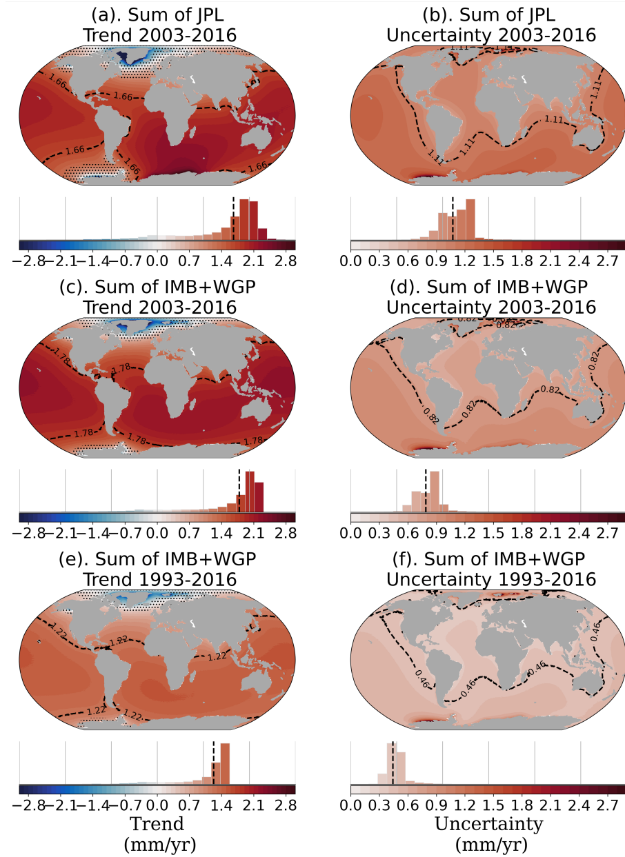
Figure 7. Total GRD-induced SLC fields of the trend and uncertainty ( \text{mm} \cdot \text{year}^{-1} ) (AIS+GIS+LWS+Glaciers contributions; intrinsic + temporal + spatial uncertainties) for GRACE (a,b) and IMBIE+WaterGAP for 2003-2016 (c,d) and for 1993-2016 (e,f). Histograms underneath each map indicates the distribution of the regional values across the oceans, in which the 5 to 95th percentile range (90%-range) is based on. Spatial average of the regional trend and uncertainty indicated by black dashed lines in the maps and bar charts. Regions with trends smaller than the 1-sigma uncertainty are indicated in the map with stipples.
