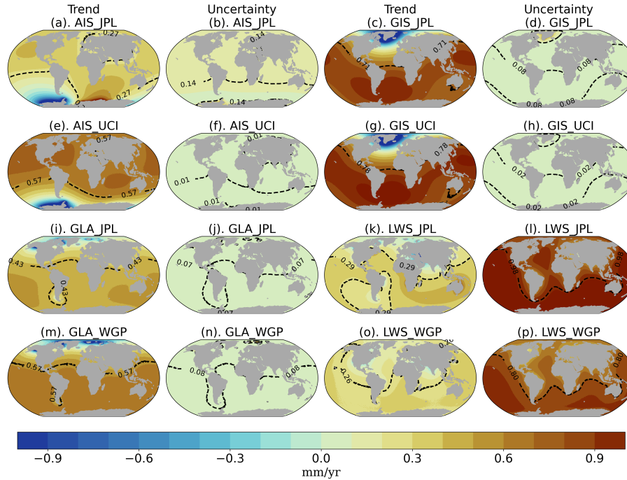
Figure 4. GRD-induced sea-level trend and temporal uncertainty ( \text{mm} \cdot \text{year}^{-1} ) for GRACE (JPL) and independent combination (UCI + WGP) for 2003-2016. Black dashed contour line and number indicates the spatial average of the regional trend and uncertainty. Trends and uncertainties of CSR, IMB, ZMP and GWB presented in Supplementary Figure A3
