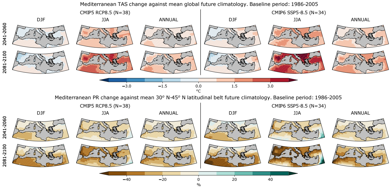
Figure 2. Mediterranean region TAS (upper rows) and PR (lower rows) change differences with respect to the mean global temperature change and the mean 30^{\circ} N- 45^{\circ} N latitudinal belt precipitation change, respectively. The changes for periods 2041-2060 (1st and 3rd row) and 2081-2100 (2nd and 4th row) are evaluated against the 1986-2005 mean. The differences are shown for the CMIP5 (left) and CMIP6 (right) DJF, JJA and annual mean projections (columns) under the high emission scenario RCP8.5 and SSP5-8.5, respectively. N indicates the number of models included in the ensemble mean.
