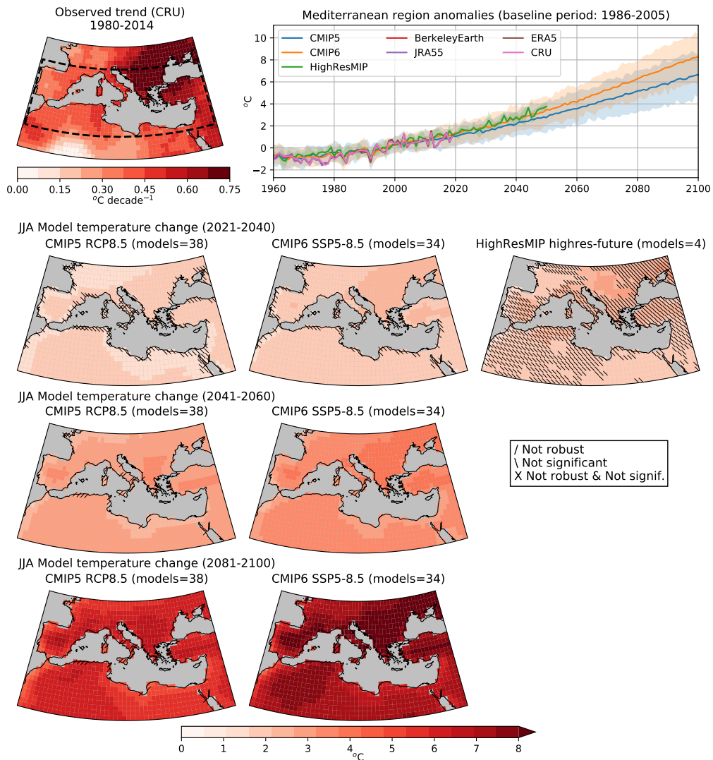
Figure 5. Summer \Delta TAS change according to CMIP5, CMIP6 and HighResMIP ensemble means (columns) for the three relevant future periods (rows), under the RCP8.5 and SSP5-8.5 scenarios. The time series plot shows the anomalies in the Mediterranean region with respect to the period 1986-2005 for the multi-model ensembles and the observational references. A solid line indicates the one-member-per-model ensemble mean and the shaded region indicates the 5th-95th percentiles range. CRU trend for the period 1980-2014 is shown along with the dashed line which bounds the Mediterranean region. Non-significant coastline grid points are due to differences in the original grid resolutions between models. Coarse models have masked data in complex coastline regions once regridded, making the ensemble smaller and therefore reducing the degrees of freedom for the t-Student test.
