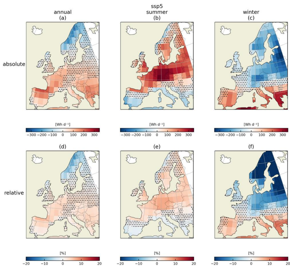
Figure 4: Impacts of climate change on PV generation in SSP5-8.5. The figure is structured as Fig. 3.
