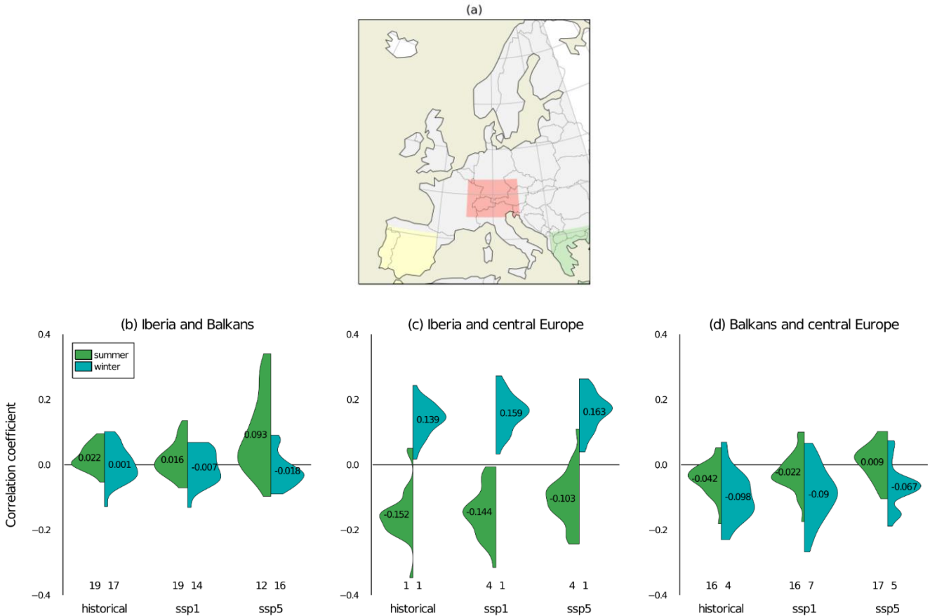
Figure 6: (a) Selected regions for the case study: Iberia ( 10^{\circ} W - 0^{\circ} , 35 - 42.5^{\circ} N; yellow), the Balkans ( 20^{\circ} W - 30^{\circ} E, 35 - 42.5^{\circ} N; green) and central Europe ( 5 - 15^{\circ} E, 45 - 50^{\circ} N; red). Lower panels: Correlation of deseasonalized PV electricity production (b) between Iberia and the Balkans, (c) between Iberia and central Europe and (d) between the Balkans and central Europe for the historical and the two SSP scenarios based on daily data. The green and blue colors distinguish correlations in summer and winter, respectively. The shapes represent the probability density function of 28 used models. The numbers in the middle indicate the mean correlation coefficient for the specific scenario in each season. The values below each violin part shows the number of models (out of 28) for which the null hypothesis (zero correlation) cannot be rejected at the 5% level. At the same time, the rest of the models have a statistically significant non-zero correlation.
