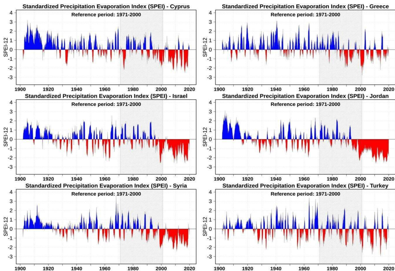
Figure 4 Standardized Precipitation Evaporation Index (SPEI) anomalies for six selected countries in the eastern Mediterranean. The plot is based on the CRU TS4.04 gridded monthly precipitation and temperature data set (Harris et al., 2020). Positive values (blue) indicate wet periods, negative values (red) indicate dry periods.
