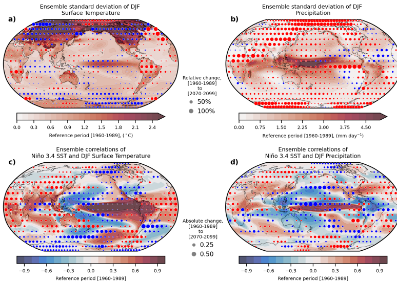
795 Figure 4: Changes in the patterns of interannual variability and Niño3.4 correlation coefficients of December-January-February (DJF) surface temperature and precipitation. (Top) Color shading shows the time-averaged absolute \sigma -ensemble \sigma_D of the DJF seasonal mean surface temperature (a) and precipitation (b) for the period 1960-1989. Circles show the relative changes in the \sigma_D between 2070-2099 and 1960-1989, where insignificant change ( p \geq 0.05 ) has been removed. Statistical significance of the changes (circles) was determined based on the p -values of the two-sample Welch's t -tests for the equality of temporal means of the \sigma_D s, with the equivalent sample sizes adjusted to account for serial correlations (Methods). 800 (Bottom) Color shading shows ensemble-wise correlations of the Niño3.4 index with surface temperature (c) and precipitation (d) anomalies for DJF, averaged over the period 1960-1989. Circles show the absolute change in correlations between 2070-2099 and 1960-1989, where statistically insignificant changes ( p \geq 0.05 ) have been removed. The Niño3.4 index for ENSO is the spatial average of sea surface temperature within 5°S-5°N, 170°W-120°W. Statistical significance of the changes (circles) was determined based on the p -values of two-sample Student's t -test of the Fisher z -transformed correlation coefficients (Timmermann et al., 2014). Note that the t -test treats the ensemble standard deviations and correlations as stationary and serially uncorrelated with either of the two periods. For all four panels, the circles represent subsampled fields at 10° intervals over the global domain. The corresponding analysis for June-July-August (JJA) is presented in fig. S9 . 805
