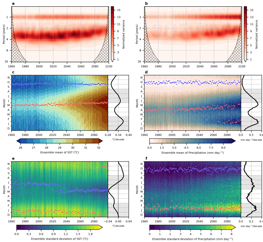
780 Figure 3: Changes in the dominant frequencies and seasonal variance of sea surface temperature (SST, left) and precipitation (right), in the Niño3.4 region (5°S-5°N, 170°W-120°W). (Top) The wavelet power spectra of Niño3.4 (a) SST and (b) precipitation using a Morlet wavelet, normalized by \sigma^{-2} , where \sigma is the ensemble mean standard deviation of the respective Niño3.4 time series (Torrence and Compo, 1998). The y-axis shows the equivalent Fourier period in years. The hatching indicates regions where the wavelet spectrum is not trustworthy due to edge effects. Prior to calculating the wavelet spectra, the time series were detrended by subtracting the ensemble-mean annual means, which were linearly interpolated to a 785 monthly timestep. (Middle) The ensemble-mean of Niño3.4 (c) SST and (d) precipitation indicated for each day (ordinate) and year (abscissa) using daily output. The red/blue dots indicate the maximum/minimum daily values of each year. The black line to the right in panels (c)-(f) indicates the linear trend over 1960-2100. (bottom) Same as for (c) and (d), but for the across- ensemble SDs of (e) SST and (f) precipitation.
