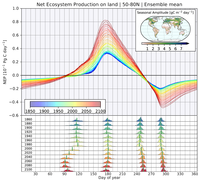
815 Figure 5: Expansion of growing season length, or equivalently the carbon uptake period, over 50°N-80°N (shown here for all 90 members for which daily-mean land output was saved). Upper panel: Evolution of ensemble mean seasonal cycle (one line for every five years, color-coded) of integrated net ecosystem productivity (NEP), with positive values indicating net 820 terrestrial carbon uptake and negative values indicating loss of carbon from the aggregated land region. The first zero crossing marks the start of the growing seasons, and the second zero crossing marks the end of the growing seasons; Lower panel: Histograms of first occurrence of zero crossing, peak, second zero crossing, and minimum as a function of the day of year. The horizontal axis for both panels is a climatological calendar day of the year , and aggregation is done across 90 members. 825 The histograms represent model output sampled at 20-year intervals. The inset map (upper right) shows the ensemble mean amplitude of the seasonal cycle of NEP averaged over 1960-1989 ( \text{gC m}^{-2} \text{ day}^{-1} ).
