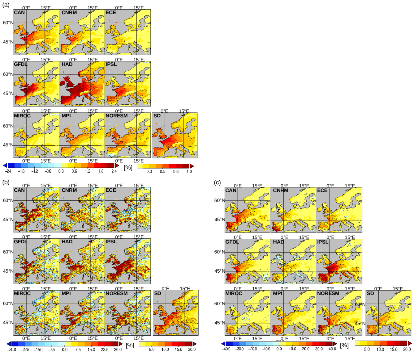
Figure 11. (a) Change in AR day frequency (2070–2099 minus 1970–1999). (b) Same as panel (a) but for percentage in AR-forced yearly maximum precipitation (% AMP); (c) same as panel (a) but for AR fractional contribution to heavy precipitation (% 95P). Note the RCA realizations are denoted by their forcing global model simply. SD CE3 denotes the inter-model standard deviation across all nine models (CAN, CNRM, ... NorESM). Long bars indicate the color scale of the ensemble member indices. Short bars are for inter-model standard deviation. All maps reflect changes for RCP8.5.
