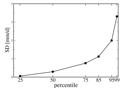
Figure 10. Inter-model standard deviation from the nine down-scaled models calculated for the 25th, 50th, 75th, 85th, 95th, and 99th percentiles of precipitation. The average over all the land grid cells of the models is shown. The percentiles have been derived from the 6-hourly time series of precipitation.
