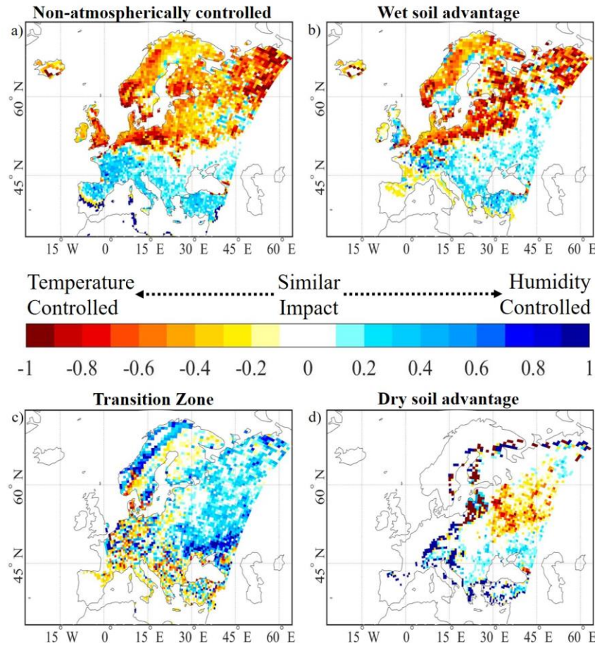
Figure 87: Sensitivity score of a) non-atmospherically controlled days per summer season, b) wet soil advantage days per summer season, c) transition zone days per summer season and d) dry soil advantage days per summer season to changes individual modifications in the air temperature profile (-1 = totally temperature controlled) and specific humidity profiles (1 = totally humidity controlled).
