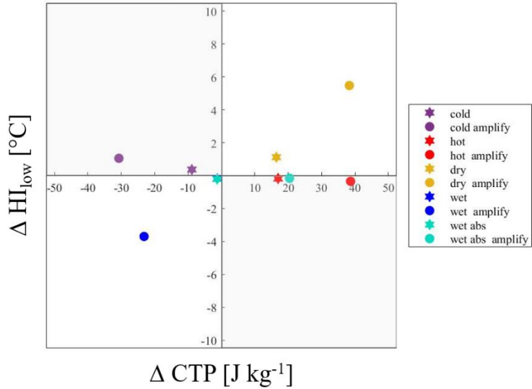
Figure 109: Changes in convective triggering potential (CTP) and low-level humidity index ( HI_{low} ) due to the divergence factors.
