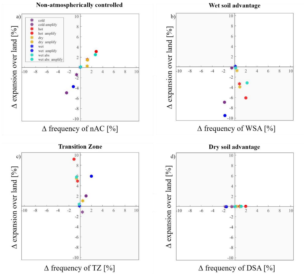
Figure 1140: Impacts of the divergence cases on the spatial expansion and the occurrence of the feedback-categoriescoupling classes in summer for a) non-atmospherically controlled (nAC) days, b) wet soil advantage (WSA), c) transition zone (TZ), and d) dry soil advantage (DSA). The x-axis depicts the changes in the average frequency of occurrence during summer and the y-axis shows changes in the fraction of land area covered by the respective coupling regime.
