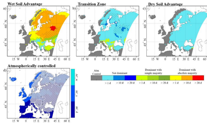
Figure 1544: Uncertainty maps of the non-atmospherically controlled classes: a) wet soil advantage, b) transition zone, c) dry soil advantage. The colours indicate whether a class is on average dominant in absolute or simple majority, or whether another class is dominant. The colour gradation denotes the average number of days. The hatching indicates that in these regions the variance in the number of days in this class is larger than 10%. Subplot d) indicates the dominant atmospherically controlled class the contours denote the maximum variance in the number of days in atmospheric control between the perturbation modification cases.
