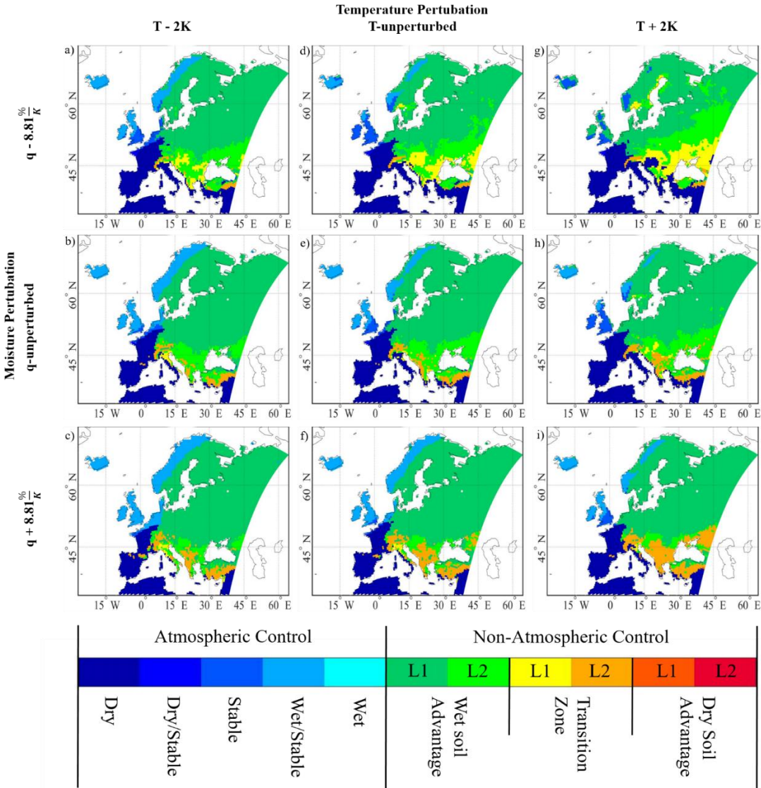
Figure 76: Long-term classification of coupling regimes for the core-set perturbationmodification cases. The columns denote a temperature change and the rows a change in moisture. The center image is the CTRL case and modified after Jach et al. (2020) (their Fig. 3a). The columns denote the temperature change and the rows the relative change in moisture.
