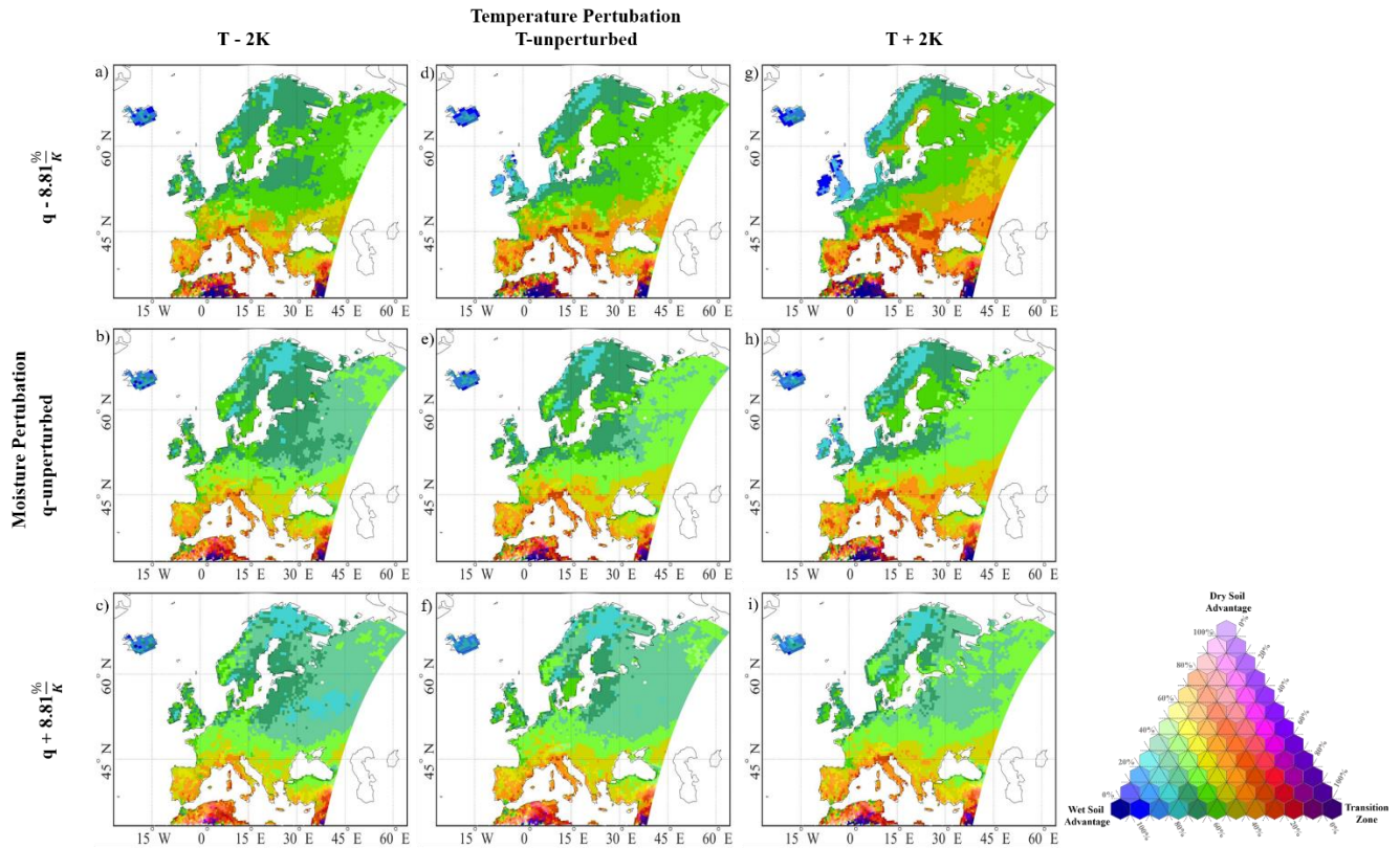
Figure 65: Composition of the non-atmospherically controlled days comprising wet soil advantage, dry soil advantage and transition zone days for all core- perturbationmodification cases. The columns denote the temperature change and the rows the relative change in moisture.
