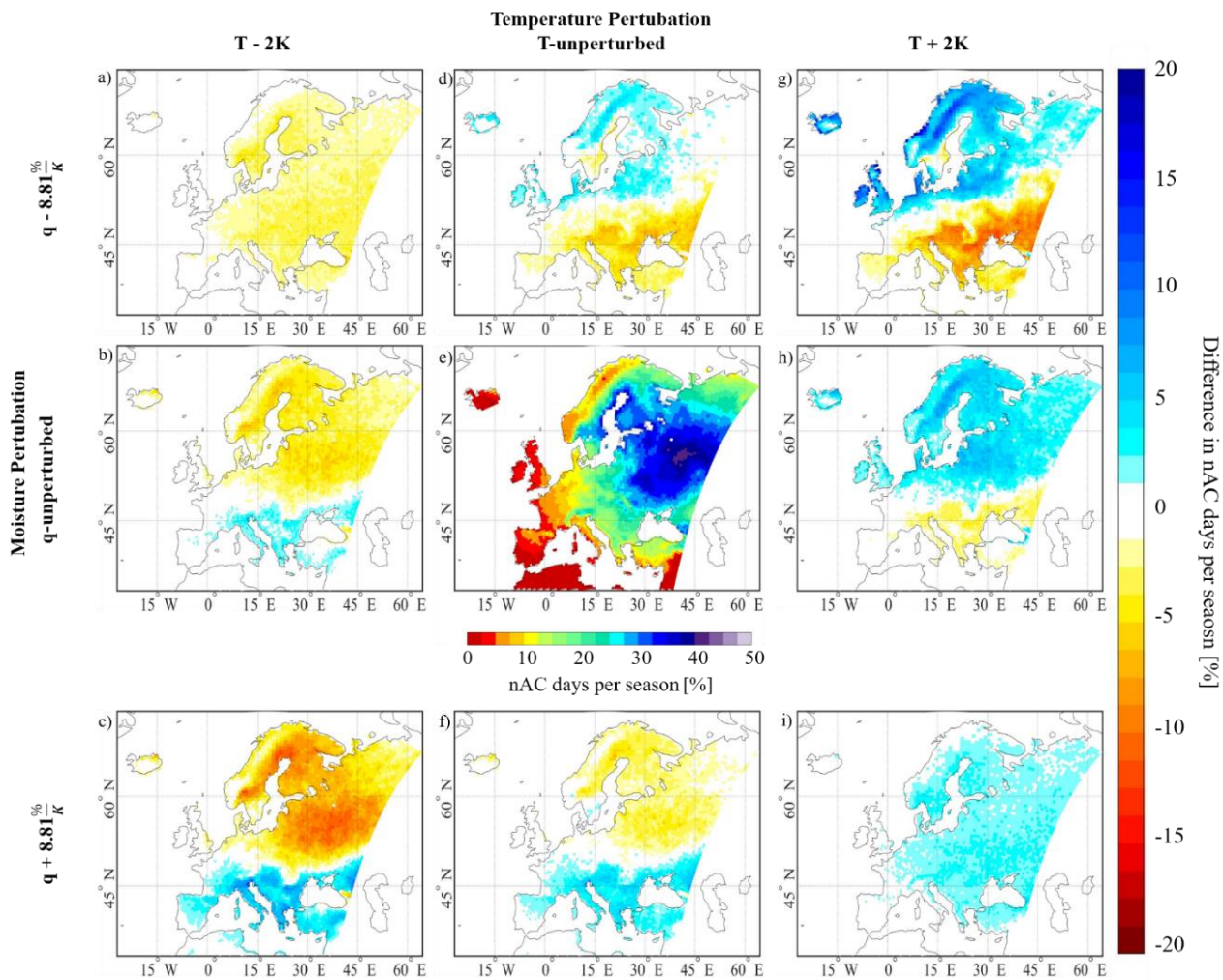
Figure 54: Difference in the seasonal share of non-atmospherically controlled (nAC) days [%] from CTRL for each perturbationmodification case of the core-set. The center image is the CTRL case modified after Jach et al. (2020) (their Fig. 4g). The columns denote the temperature change and the rows the relative change in moisture.
