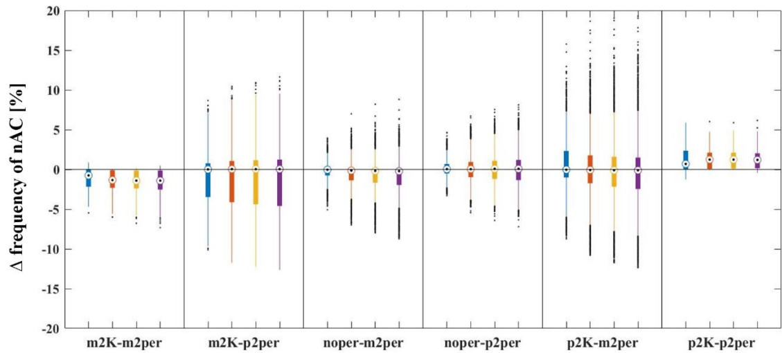
Figure 32: Changes in frequency of non-atmospherically controlled (nAC) days in response to different combinations of temperature and moisture changes in the core- perturbation modification set. m2K denotes a cooling by 2K at the surface, p2K a warming of 2K at the surface, m2per denotes a dry of two times the scaling factor and p2per denotes a moistening by two times the respective scaling factor in the domain for different T-q scaling factors. Blue: 5% K -1 , orange: 7.74% K -1 , yellow: 8.81% K -1 , purple: 9.66% K -1 .
