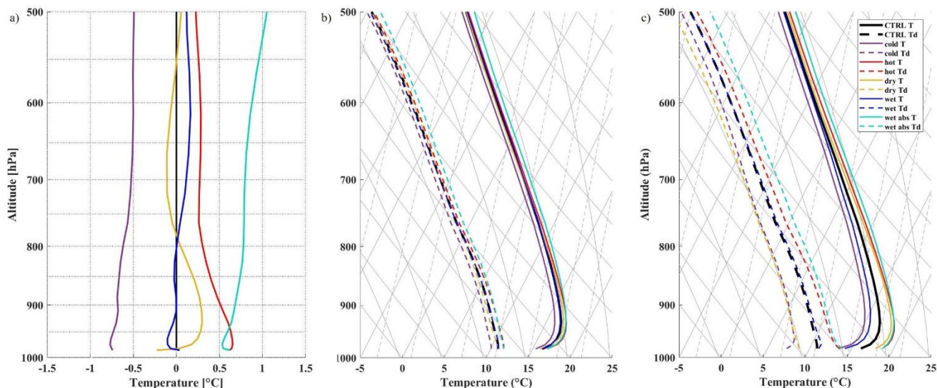
Figure 98: a) D ivergence temperature (T) factors derived from differences of the domain average temperature profiles of the corresponding summers to the 30-year mean (Tab. 2) which were used to perturb-modify daily model output, b) domain average of T and Td Profiles for the divergence T-factors, and c) their additional modifications with the core T-factor. purple: cold, red: hot, yellow: dry, blue: wet, turquoise: wet abs; Solid lines represent temperature and dashed lines represent dew point temperature.
