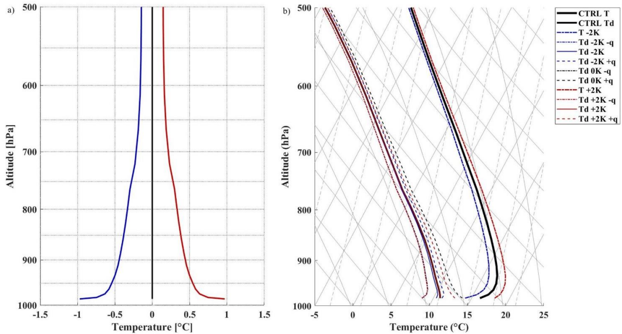
Figure 43: Temperature perturbationmodification factor derived using a simple linear regression model and extracting the coefficient of determination for each atmospheric layer (left). Profiles of temperature (T) and dew point temperature (Td) after perturbationmodification (right). Red indicates warmer temperature, blue cooler temperatures and unchanged temperature is denoted in black. Dash-dotted lines indicate a reduction in moisture, solid lines unchanged moisture and dashed lines an increase in moisture.
