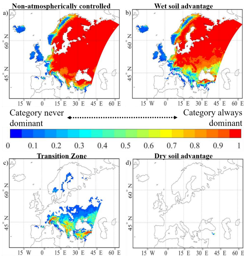
Figure 1312: Sensitivity of feedback coupling categories-classes of a) any feedback coupling category class , b) classified as wet soil advantage level-1 or level-2, c) classified as transition zone level-1 or level-2, and d) classified as dry soil advantage level-1 or level-2
