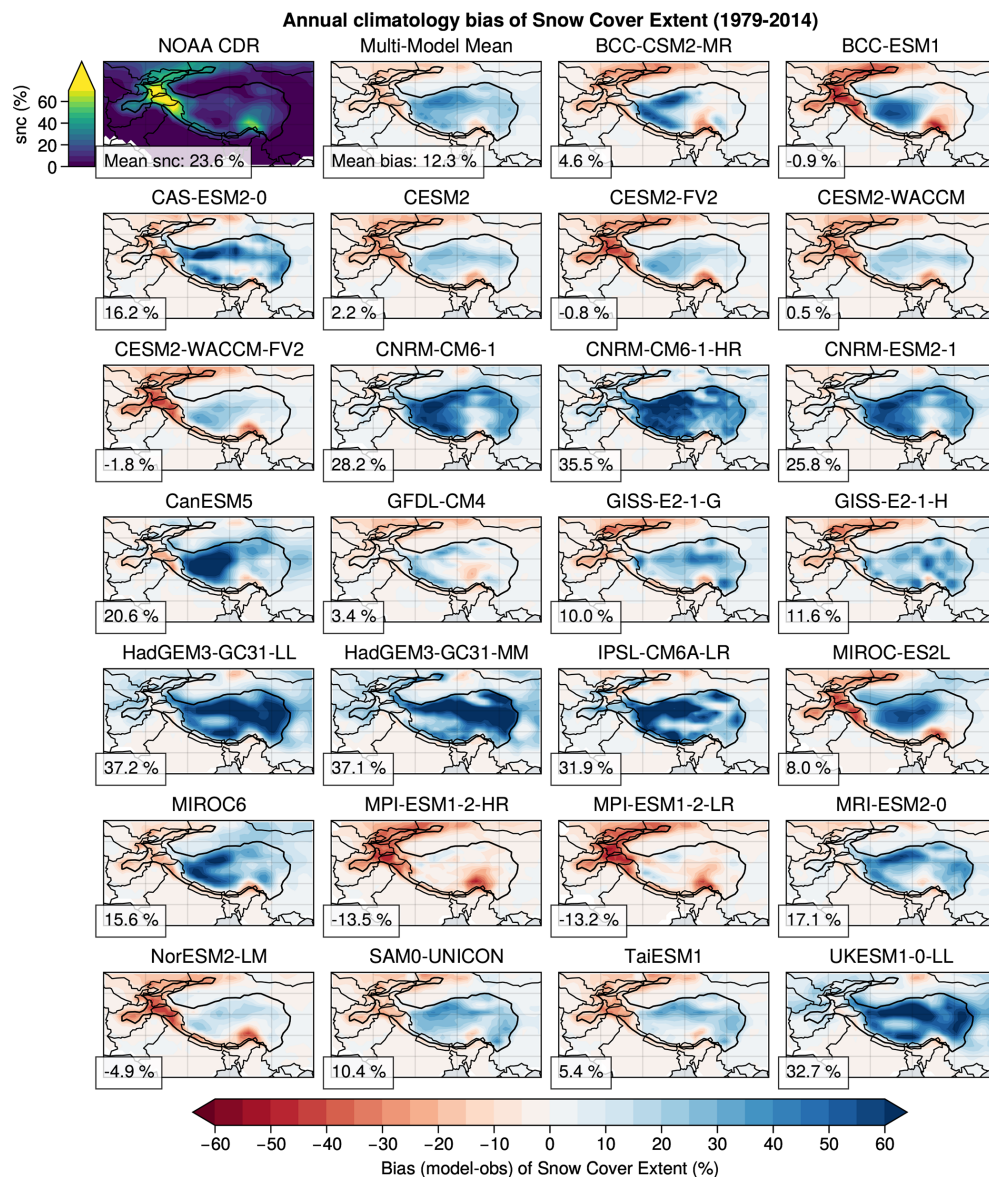
Figure B1. Same as Fig. 3 but for snow cover extent.
