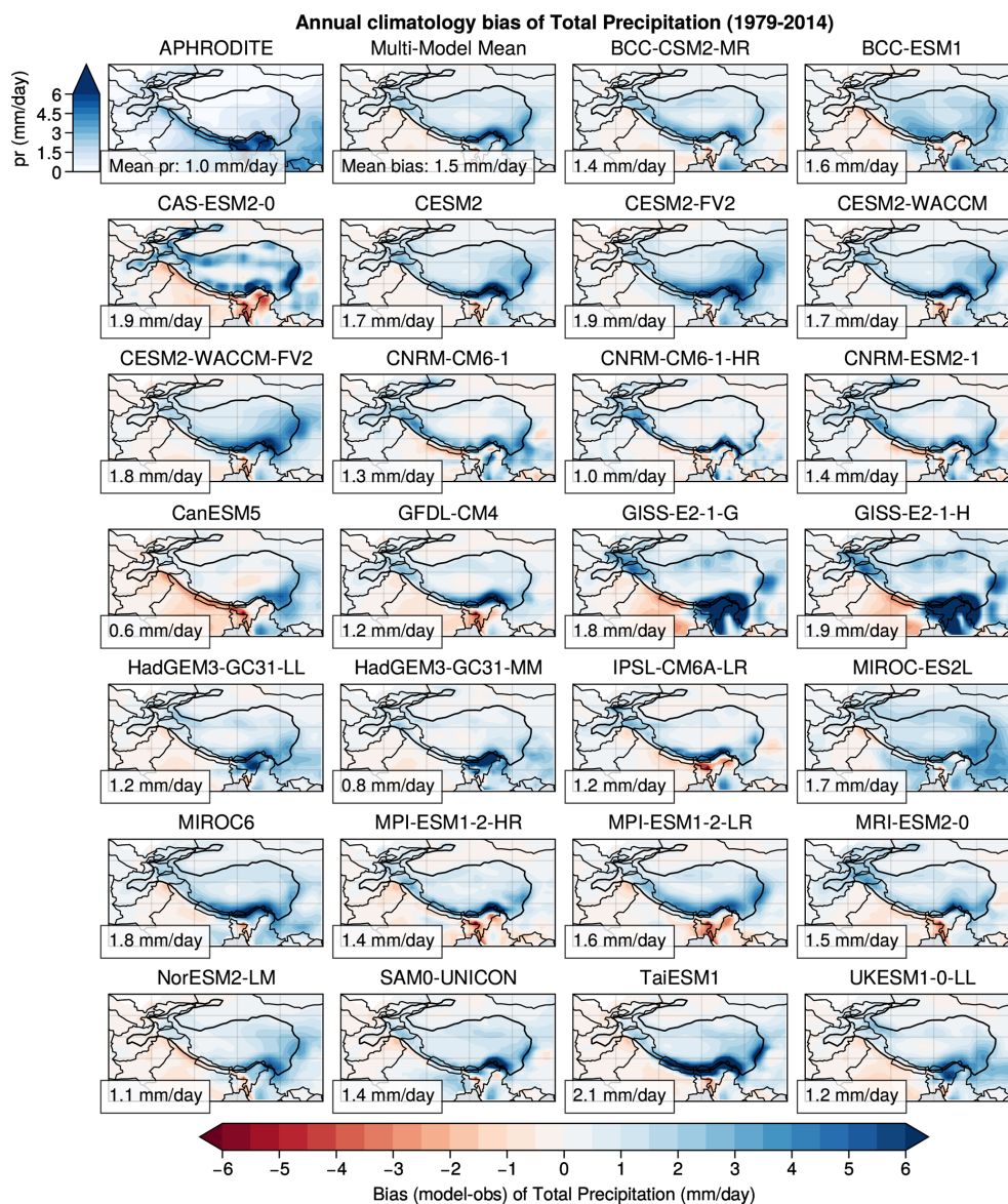
Figure B2. Same as Fig. 3 but for total precipitation.
