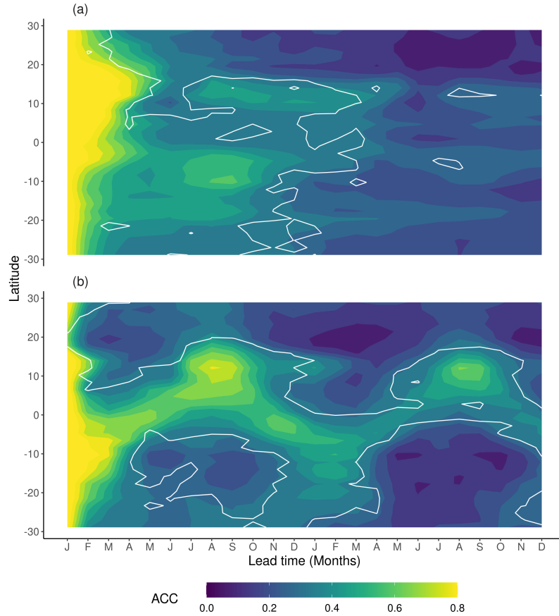
Figure 2. Zonal means of ACC derived from 35 ensemble simulations starting in January for (a) NPP and (b) Rh. Contour lines indicate correlations above the 95% confidence level.
