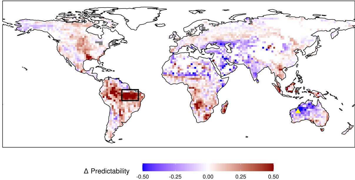
Figure 7. Difference in NPP predictability ( V_c ) based on the initial soil moisture. The mean NPP predictability of the first year from the 20% driest initializations are subtracted from the 20% wettest initializations for every grid cell. Red color means higher NPP predictability in wet years and blue color a higher predictability in dry years. Soil moisture from 19 – 78 cm depth is used to determine initial conditions. A large fraction of years included in the initializations are ENSO years, where the initial anomaly is further extended through persisting oceanic forcing. The black box and yellow triangle stand for regions examined in the main text.
