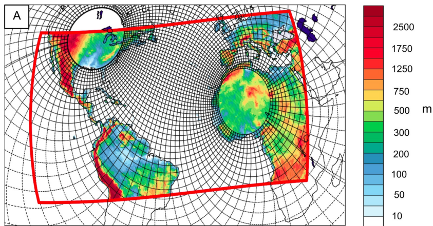
Figure 1S: ROM atmospheric and oceanic grids. The red line shows the limits of the atmospheric domain, while the black lines represent the oceanic mesh (each 12 th line is shown).
