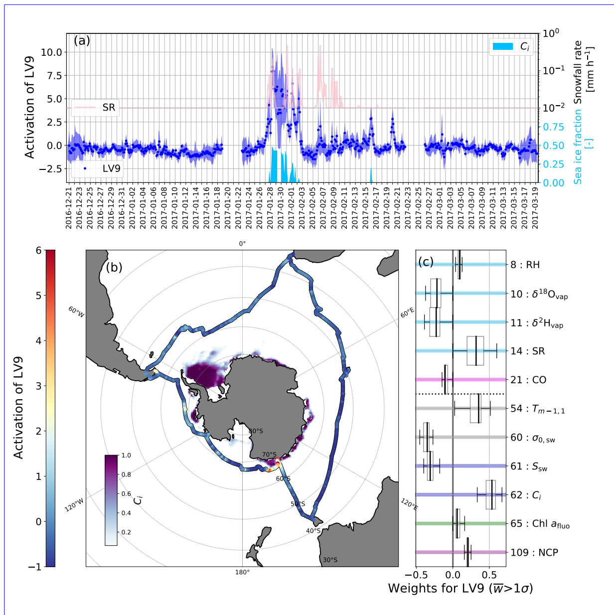
Figure 4. (a) time series of the activation of LV9 “Marginal sea ice zone and snowfall” (left axis), sea ice fraction (lower right axis), snowfall rate (upper right axis); (b) the ship track coloured by the activation of LV9 and the sea ice cover during ACE (Peng et al., 2013); (c) box and whisker plots of the activated weights.
