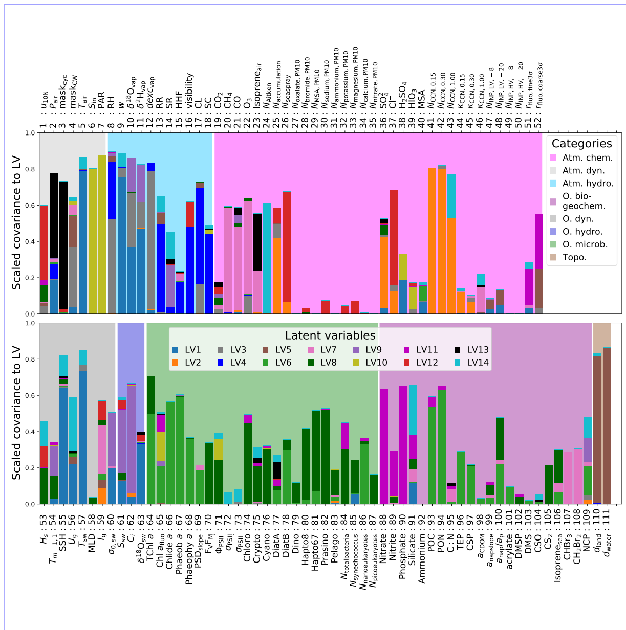
Figure 6. Covariance between the LVs and OV s scaled by the sPCA weights (see Equation 4) as stacked bar plots, with the colour denoting the LV (see legend in the lower panel). OV categories (see section 2.2) are indicated by the background shading (see legend in the upper panel).
