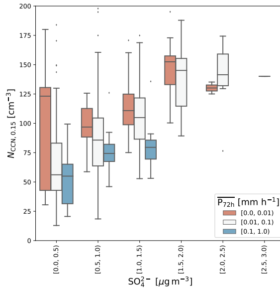
Figure A8. Box and whisker plots of N_{CCN,0.15} as function of the particulate SO_4^{2-} concentration and the average ERA5 total precipitation rate along the air mass back trajectories over 72 hours before arrival.
