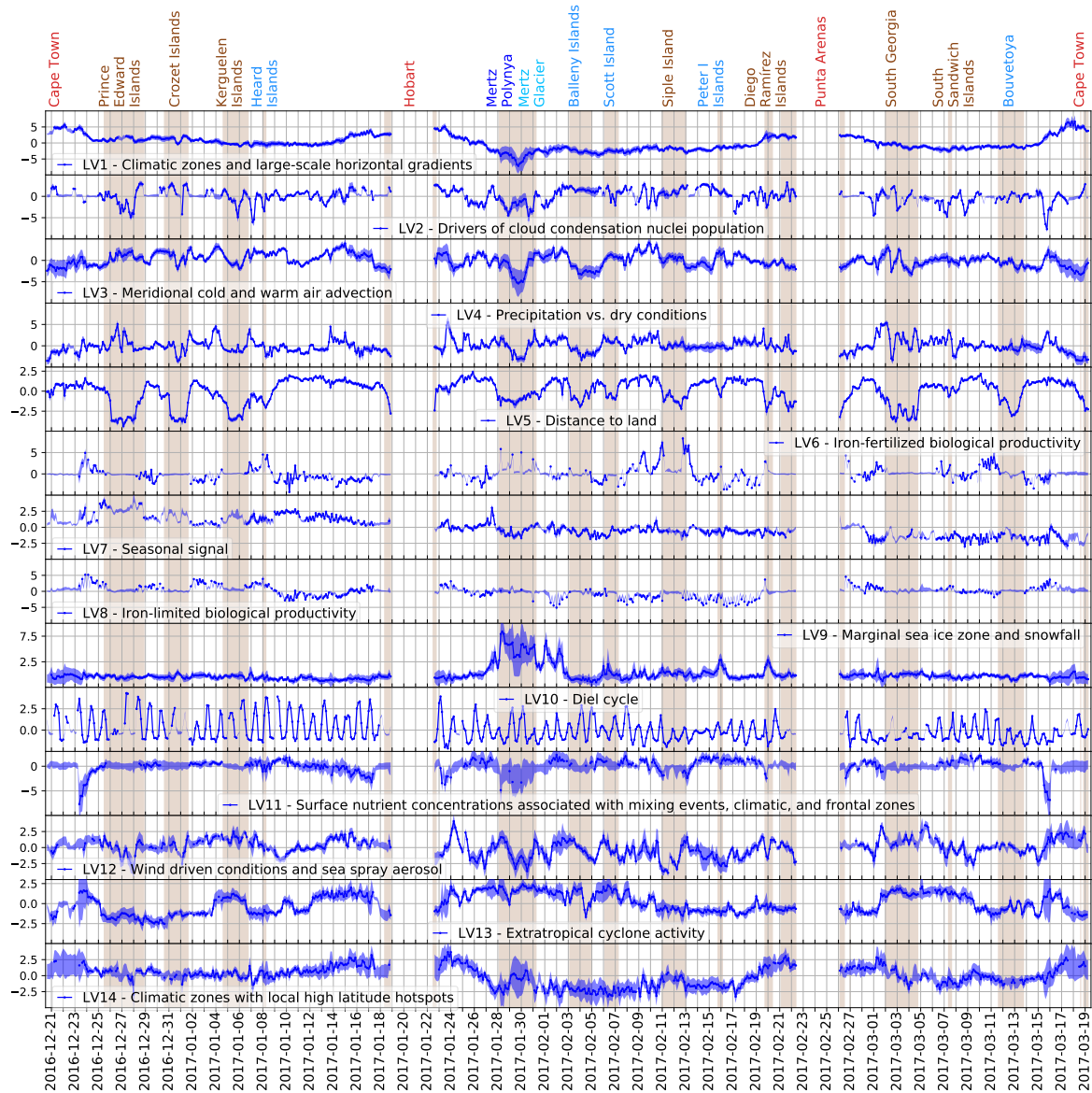
Figure 3. Time series of the LV activations LV_s . Each time series (blue dots) is calculated as the average of the principle components of the bootstrap runs and the standard deviation (STD) is used to estimate the 95% confidence interval as \pm 2STD . Mean activation of the LV (blue dots) is only shown if more than 50% of the OVs with the 50% largest weights were observed. Brown shading indicates periods when the ship was within 100 km of the nearest shore. Places visited (ports, islands and the Mertz Glacier and Polynya) are indicated at the top.
