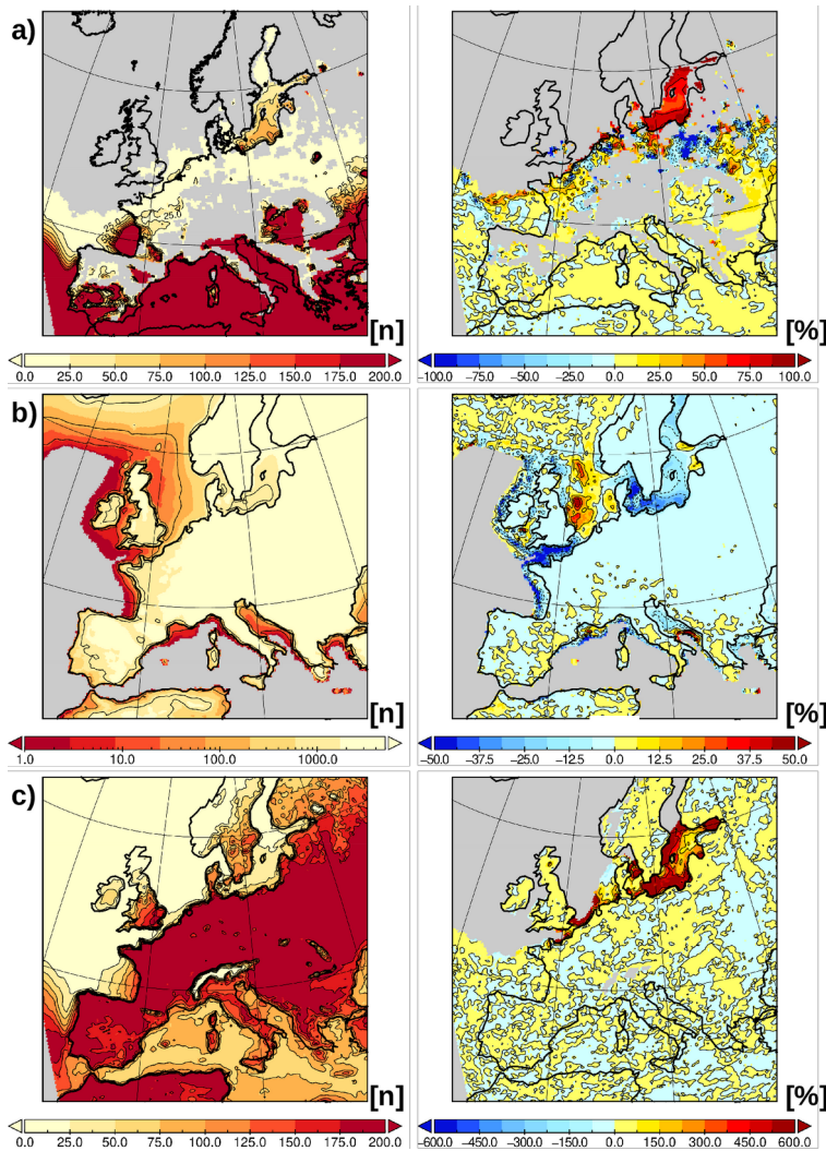
Figure 5: a) left: Number of tropical nights diagnosed from the coupled regional ocean atmosphere model during the reference period 1970-1999. right: Difference [%] of the coupled minus the uncoupled model. b) same as a) but for the number of frost days. c) left: number of periods of at least 3 consecutive warm days (days where the daily maximum temperature exceeds 20°C). right: Difference [%] of the coupled minus the uncoupled model.
