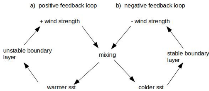
Figure 4:a) positive winter feedback loop. b) negative summer short circuit. Drawn after Gröger et al. (2015).
