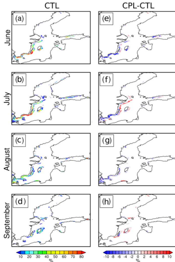
1005 Fig. 7: The left column shows the upwelling frequency during June to September, 2015, the right column shows the difference between the simulation considering wave influence and the control experiment (Figure is adapted from Wu et al., 2019b).
