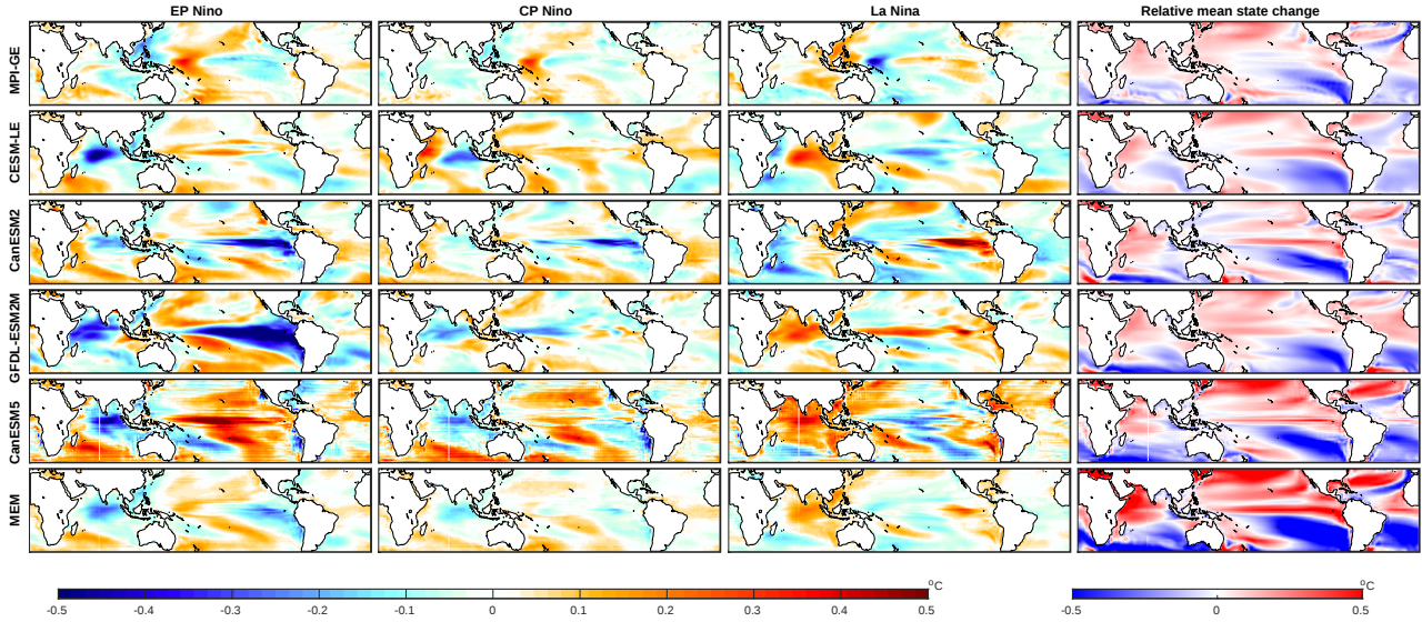
Figure 5. Change in SST pattern in each SMILE in the period 2050-2099 as compared to 1950-1999 for EP and CP El Niños, and La Niña events (left, centre left and centre right columns respectively). The mean state change in SST is shown in the right column. Shown for each individual SMILE (in order of appearance; MPI-GE, CESM-LE, CanESM2, GFDL-ESM2M, CanESM5) and the multi-ensemble mean (bottom row). The SST pattern is calculated as the November, December, January average and composited for each event type over each time-period. The relative mean state change is calculated as the ensemble mean SST over each time period, with the earlier period subtracted from the latter relative to the total change in the region shown (0-360E, 40S-40N). SMILE data has the forced response (ensemble mean) removed prior to calculation for the SST change, but not the mean state change.
