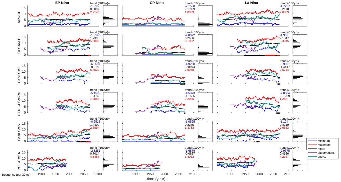
Figure 3. ENSO frequency in each SMILE for EP and CP El Niños, and La Niña events (left, middle and right columns respectively). Black line shows the ensemble mean for each year, red line shows the ensemble maximum, the blue line the ensemble minimum, the purple line is HadISST observations, and the green line is the first ensemble member. Frequency is calculated as the number of events in a single ensemble member per 30 years, taken as a running calculation along the time-series. PDFs show the distribution of ensemble members for the entire time-series. Black dots on the x-axis demonstrate when the signal (current ensemble mean minus the ensemble mean at the beginning of the time-series) is greater than the noise (standard deviation taken across the ensemble). Red dots show when the signal is 1.645 times the noise, while magenta dots show the same when the signal is greater than 2 times the noise. These thresholds correspond to the likely , very likely and extremely likely ranges. Maximum (red), mean (black) and minimum (blue) trends across the individual ensemble members are shown in text at the top right of each panel.
