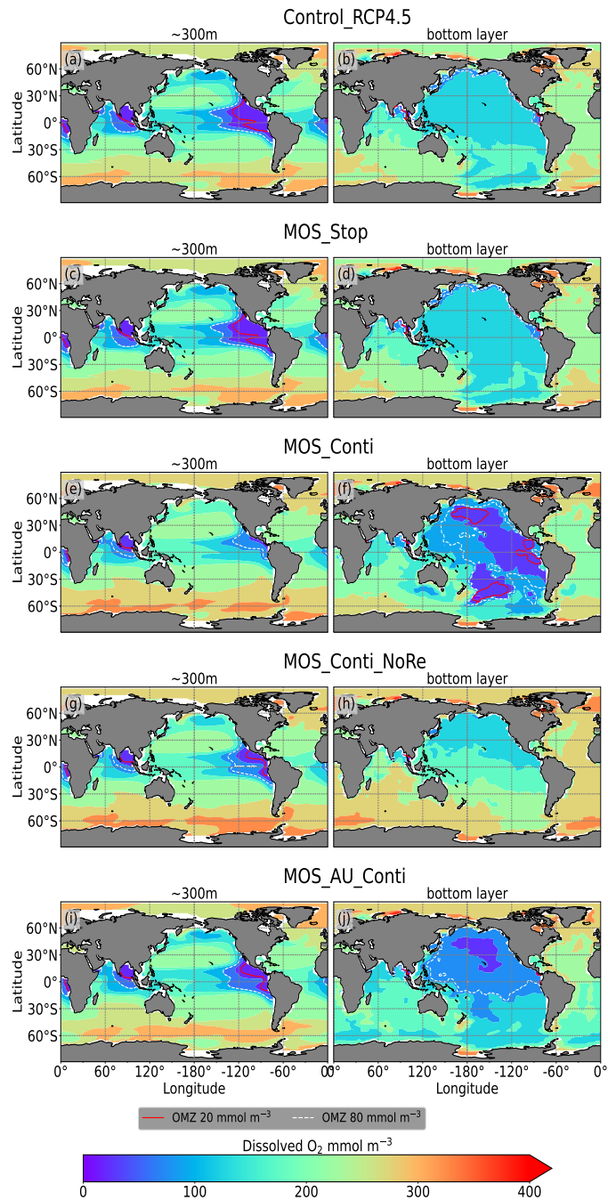
Figure 11. Dissolved O_2 concentrations at depth \sim 300\text{m} (left panel) and the ocean bottom (right panel) in year 3000: contour lines indicate boundaries of OMZs with less than 80\text{ mmol m}^{-3} oxygen (white dashed) and less than 20\text{ mmol m}^{-3} (red solid). Continuous MOS deployment further shrinks the OMZ at 300m depth (e,g,i) but expands them at bottom (f,j) except for the zero remineralization one in (h).
