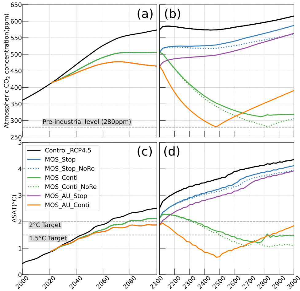
Figure 4. Simulations of: a, b: annual global mean atmospheric CO 2 concentration; c, d: surface averaged temperature relative to the pre-industrial (averaged of year 1850 to year 1900) level of 13.18°C ( \Delta SAT). Under RCP4.5 scenario, MOS reaches the 2°C target in conjunction with AU, while the 1.5°C cannot be met in all MOS simulations. Note that MOS is terminated whenever pre-industrial concentrations of atmospheric CO 2 are reached, as seen for MOS_AU_Conti (orange solid) and MOS_Conti_NoRe (blue dotted) in (b&d). Both atmospheric CO 2 and \Delta SAT remain lower than control after MOS termination.
